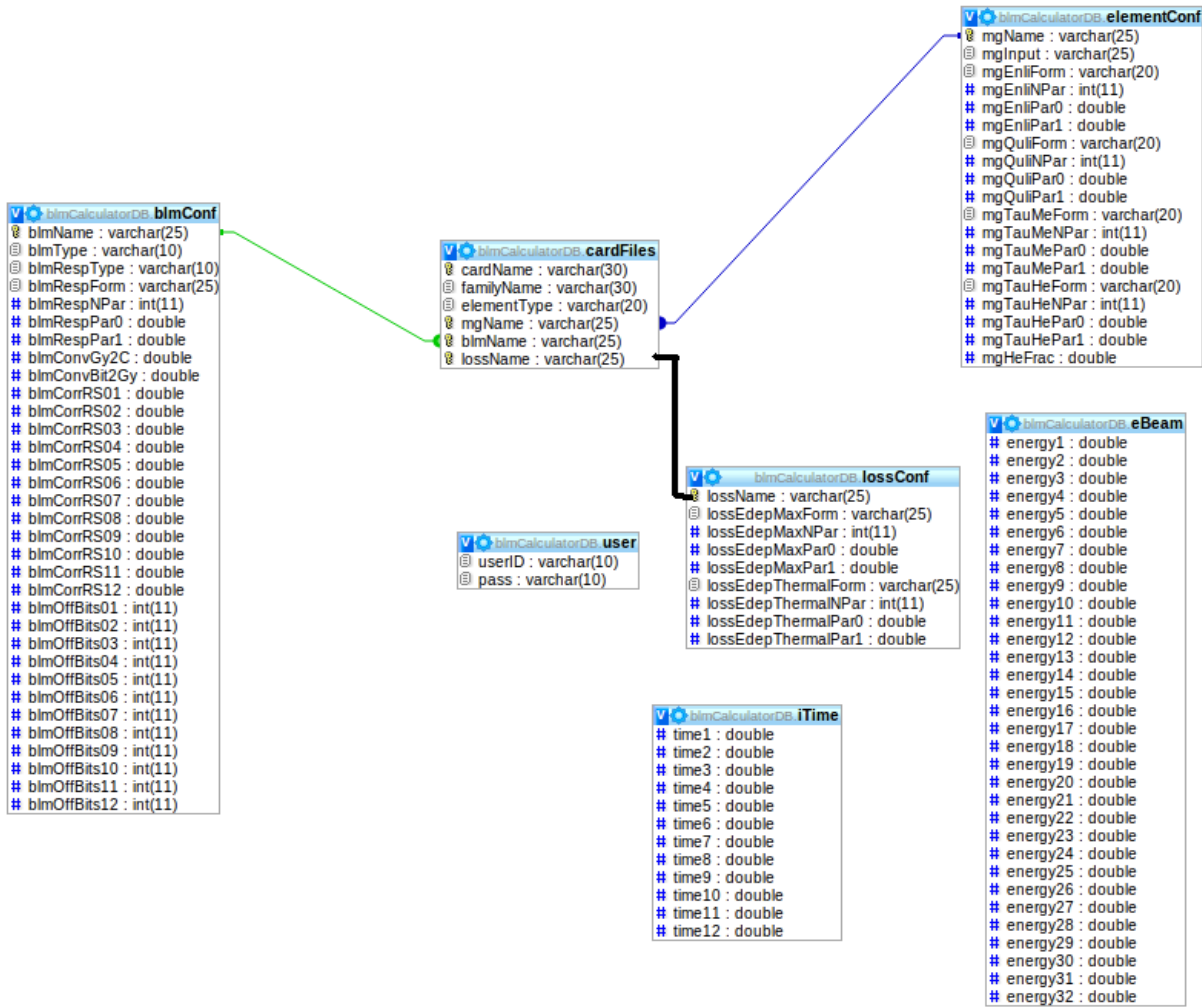
Figure 12: BLM abort threshold calculator entity relationship diagram.
