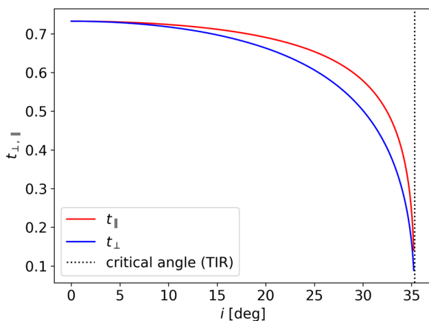
Fig. 2 A plot of the modified transmission coefficient, t_{\parallel} , t_{\perp} versus angle of incidence, i . The critical angle of the lunar surface is indicated in a black dot. Parallel and perpendicular components of the transmission coefficient are indicated with red and blue lines, respectively
