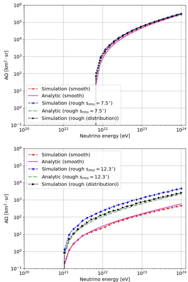
Fig. 14 Plot of the effective lunar aperture as a function of primary neutrino energy with a constant inelasticity, 20% and transmission coefficient, 0.6 and taking into account large scale surface roughness sampled from a distribution (rough distribution) or a single rms slope, s_{rms} (rough s_{rms} = 7.5^\circ at 150 MHz, 12.3^\circ at 1.5 GHz). Top: 150 MHz. Bottom: 1.50 GHz. Smooth in the legend implies surface roughness was not taken into account
