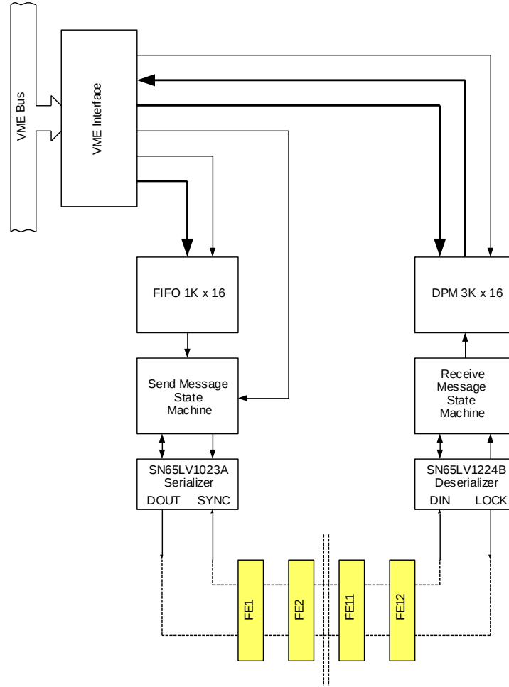
Fig. 3 Data transmission logic
