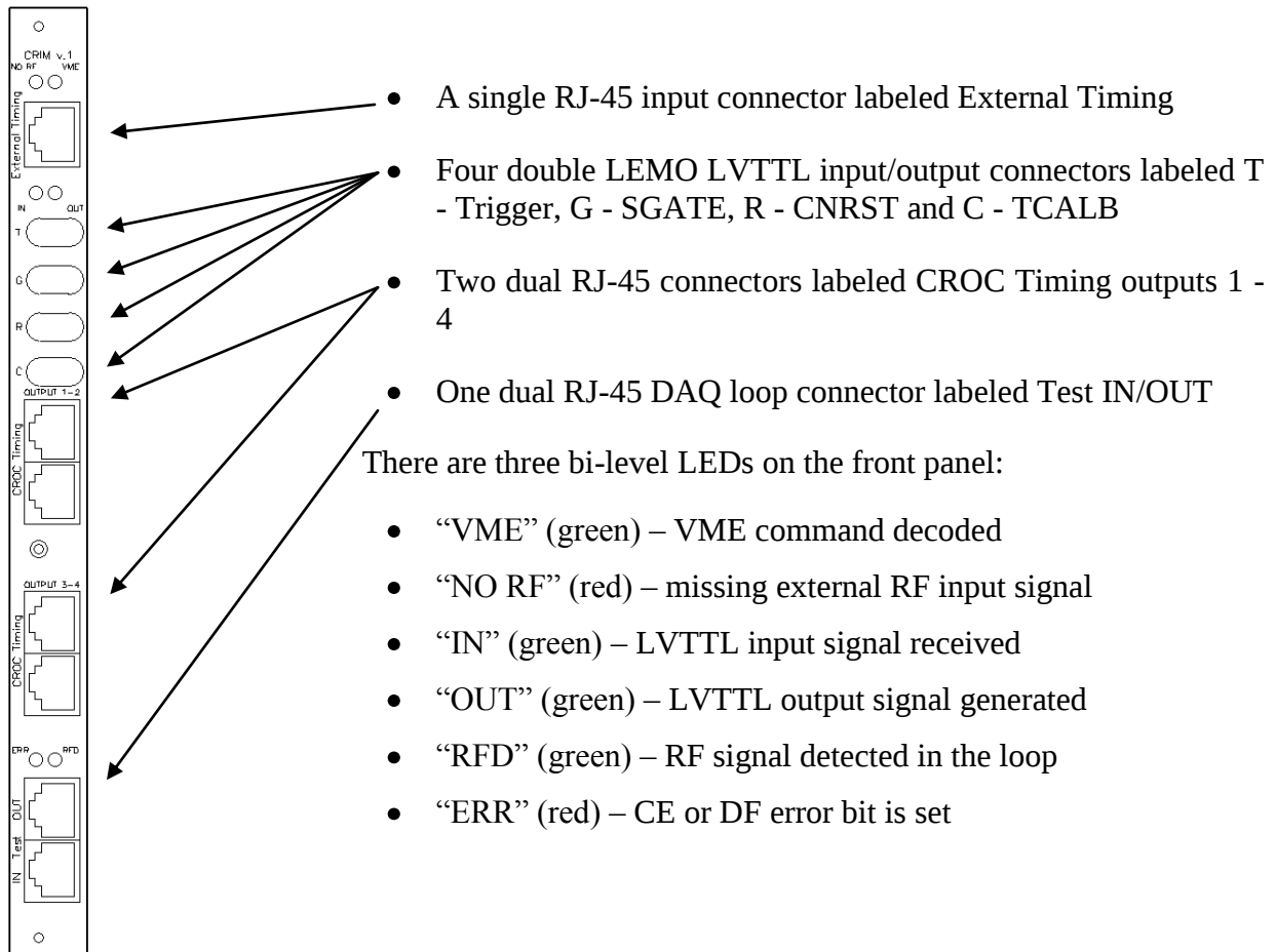
Fig. 8 CRIM front panel
