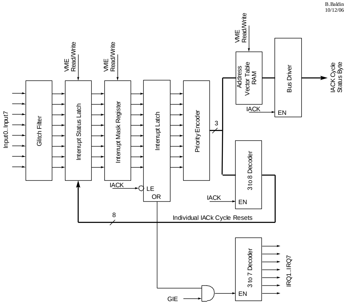
Fig. 5 Block Diagram of the CRIM Interrupter Logic
