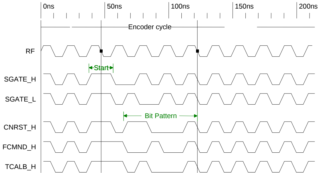
Fig. 2 Timing Encoder signals
