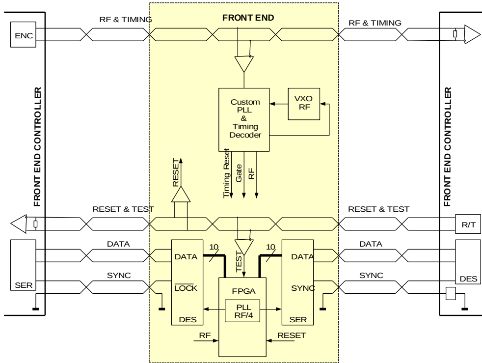
Fig. 1 Diagram of the DAQ loop signals
