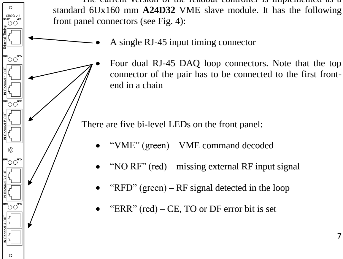
Fig. 4 CROC front panel
