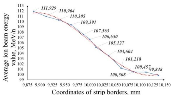
Figure 2: Distribution of energy peaks over strips.
