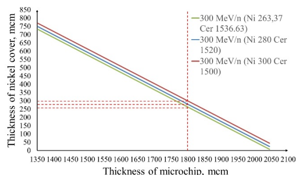
Figure 4: The dependence of the thickness of the nickel cover on the thickness of the microchip.
