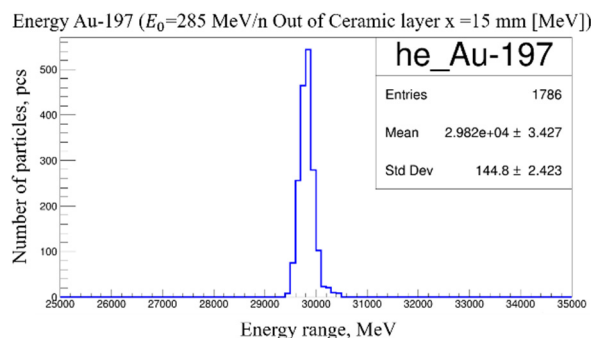
Figure 6: The energy spectrum of the ion beam at the exit from the ceramic layer after passing through distance 15 mm (an average energy of the ion beam is E_2=151.37 MeV/n).
