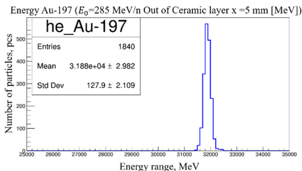
Figure 5: Energy spectrum of the ion beam at the exit from the ceramic layer after passing through distance 5 mm (an average energy of the ion beam is E_1=161.83 MeV/n).
