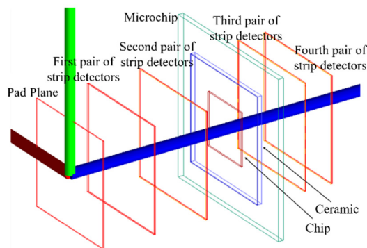
Figure 1: The geometry's target unit (sample microchip, set of detectors in front of and behind sample microchip).
