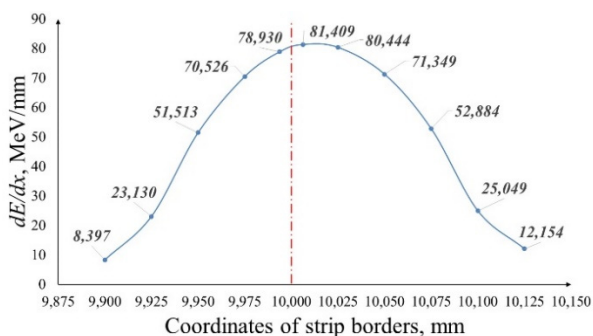
Figure 3: The derivative of the energy peaks in the transverse plane (over strips).
