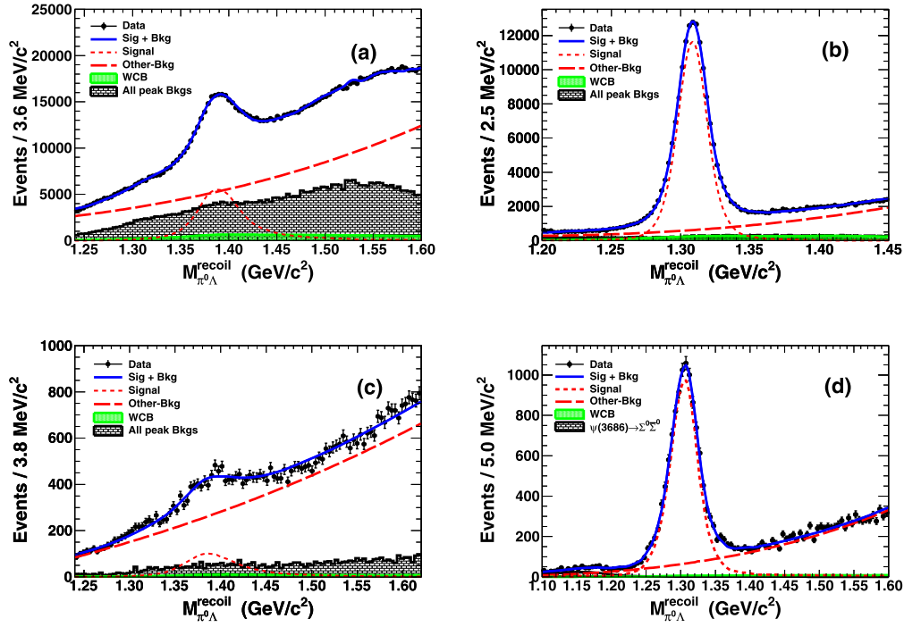
Fig. 3. (Color online.) Recoil mass spectra of \pi^0 \Lambda for (a) J/\psi \rightarrow \Sigma(1385)^0 \bar{\Sigma}(1385)^0 , (b) J/\psi \rightarrow \Xi^0 \bar{\Xi}^0 , (c) \psi(3686) \rightarrow \Sigma(1385)^0 \bar{\Sigma}(1385)^0 , and (d) \psi(3686) \rightarrow \Xi^0 \bar{\Xi}^0 . Dots with error bars indicate the data, the blue solid lines show the fit result, the red short-dashed lines are for signal, the red long-dashed ones are for the remaining background (Other-Bkg), and the green hatched ones are for wrong combination background (WCB), the black hatched ones are for the peaking backgrounds.
