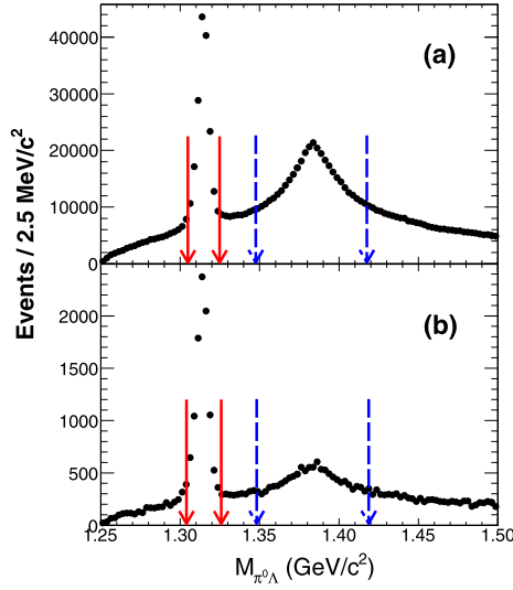
Fig. 2. Distribution of M_{\pi^0\Lambda} for (a) J/\psi and (b) \psi(3686) data. The arrows denote the applied requirements, where the dashed arrows the \Sigma(1385)^0\bar{\Sigma}(1385)^0 signal region and the solid arrows show the \Xi^0\bar{\Xi}^0 signal region.
