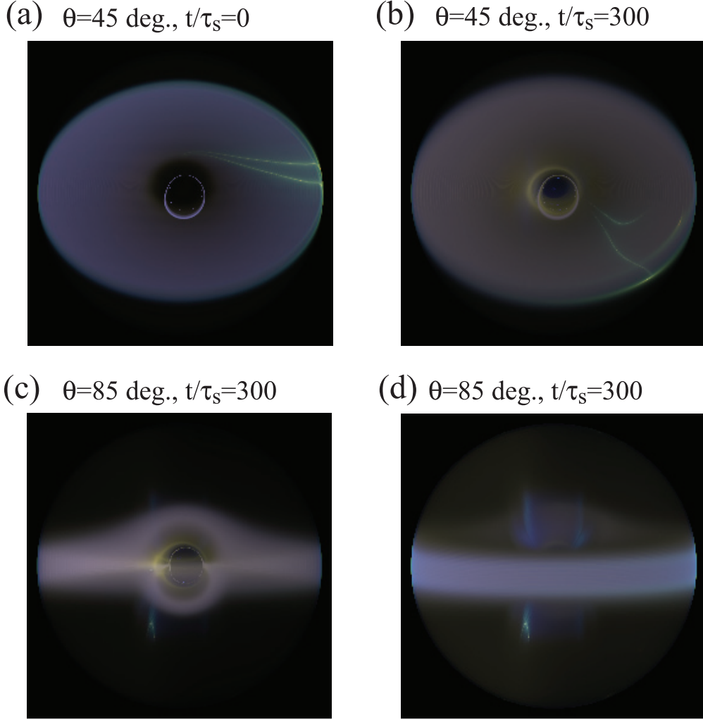
Fig. 2.— Top : Images of emission from the simulated flows viewed at an inclination angle of 45^\circ at t/t_s = 0 and 300 , corresponding to the simulation initial and final states respectively. The jet is invisible, but bright synchrotron filaments can be seen near the disk surface. The bright blue ring at the center is a first-order lensed disk image. A new fuzzy yellowish ring appears near the center of the image of t/t_s = 300 . It corresponds to the direct thermal free-free emission from highly dense gas piled up in the inner accretion disk. Bottom : Images of emission from flows viewed at an inclination angle of 85^\circ for optically thin and optically thick cases (panels c and d respectively). For the optically thick case, we consider an additional opacity due to Thomson scattering. We approximate this process by assuming that it only removes the line-of-sight photons without adding photons into the line-of-sight substantially. As the thermal synchrotron and the thermal free-free emission are both optically thin, the absorptive opacity is provided by Thomson scattering. The counter-jet is visible below the equatorial plane in the optically thin case. The details of the jet are more visible in the optically thick case.
