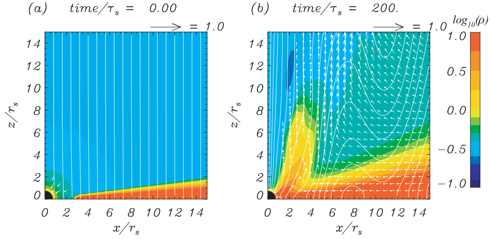
Fig. 1.— Snapshots of proper density of the accretion inflow and outflow obtained by the GRMHD simulation at t/t_s = 0 and 200. The white curves represent magnetic field lines (contours of poloidal vector potential) and the arrows depict the poloidal velocities normalized to the speed of light.
