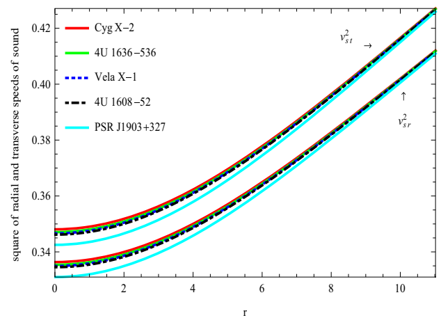
Fig. 8 Behaviour of the square of radial and transverse speeds of sound against the radial coordinate r of our stellar model for strange astrophysical stars Cyg X-2, 4U 1636-536, Vela X-1, 4U 1608-52 and PSR J1903+327 for the parameters given in Table 1
