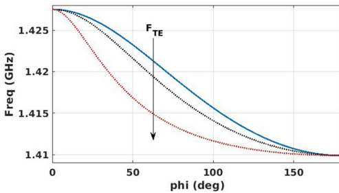
(b) Effect of TE-TM interaction
