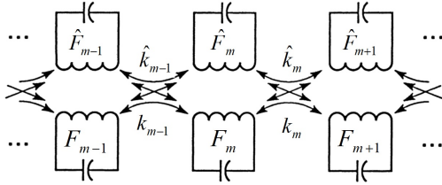
Figure 2: Equivalent circuit representation: m is the cell index, F_m is the single cell frequency, k_m the coupling constant between two adjacent cells. The quantities with the symbol “ \wedge ” refer to the TE mode.
