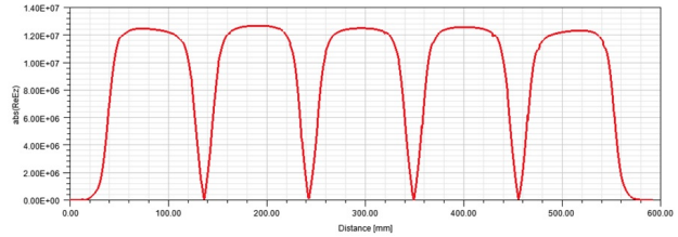
Figure 4: Profile of the absolute value of the electric field on axis.
