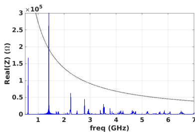
Figure 6: Impedance combination of structures with slot apertures of 23.5^\circ and 25^\circ . Black dashed line is the LCBI threshold.
