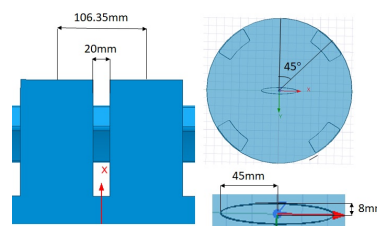
Figure 1: Standard cell with its main parameters.
