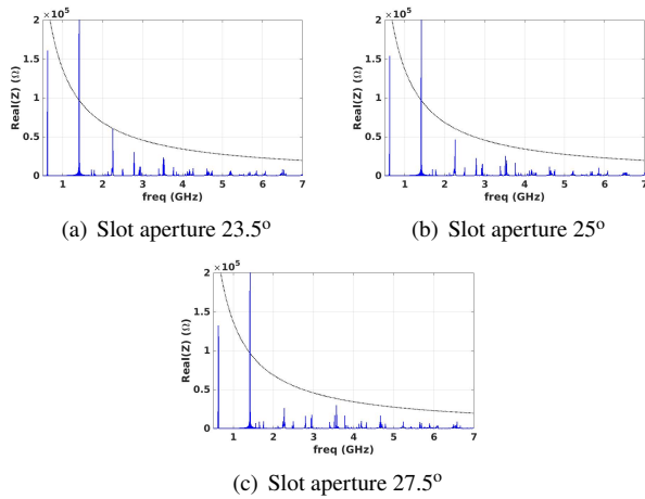
Figure 5: Longitudinal impedance and LCBI threshold (black dashed line).
