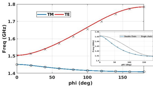
(a) Model prediction vs HFSS simulation data
