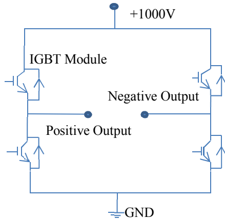
Figure 3: Topology of the dipole power supply.
