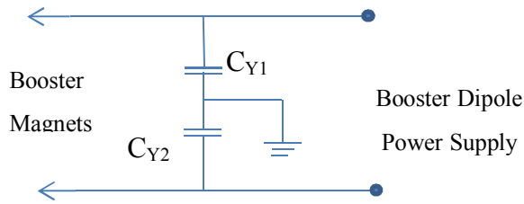
Figure 6: Adding a Y circuit to the output stage.
