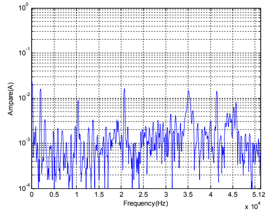
Figure 8: Current ripple in the dc mode with an added common-mode filter (frequency from 0 to 51.2 kHz).
