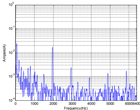
Figure 7: Current ripple in the dc mode and with an added common-mode filter (frequency from 0 to 6.4 kHz).
