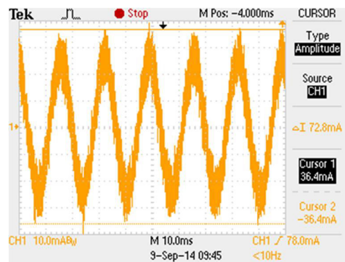
Figure 4: Using the negative output line and ground line of the AC source connection to measure the current.
