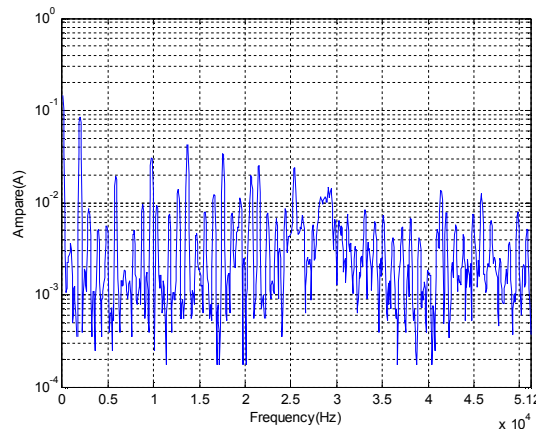
Figure 2: Current ripple in dc mode (frequency from 0 to 51.2 kHz).
