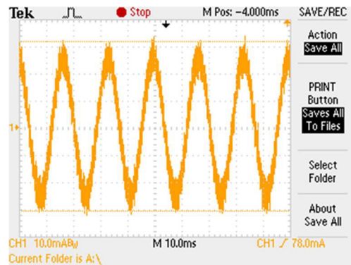
Figure 5: Using the positive output line and ground line of the AC source connection to measure the current.
