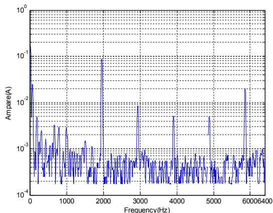
Figure 1: Current ripple in the dc mode (frequency from 0 to 6.4 kHz).
