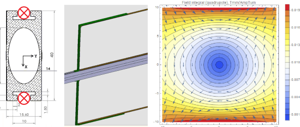
Figure 8: Two current carrying coils mounted on the vacuum chamber (left and middle) and the quadrupole field integral (right) produced by coil consisting of one turn with 1 A current.
