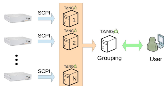
Figure 1: Control System integration architecture.
