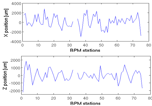
Figure 6: Beam orbit measurements.
