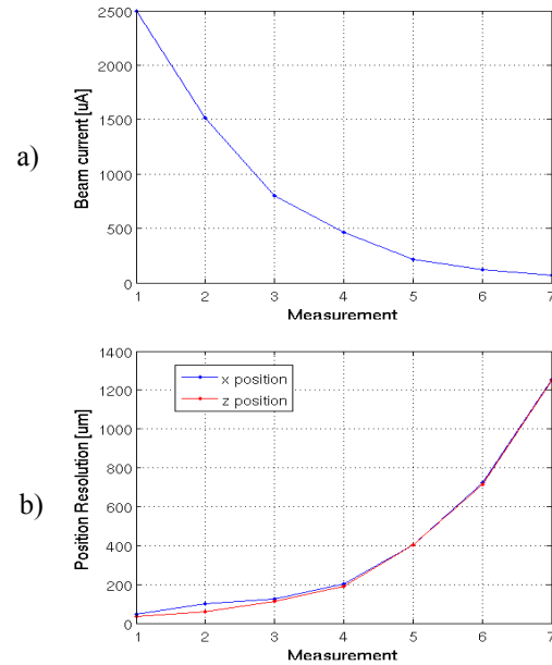
Figure 4.a: current measurements with the SUM signal; Figure 4.b: X and Z position resolution Vs current.
