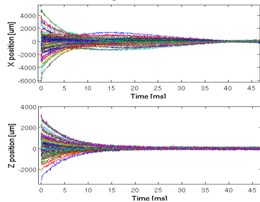
Figure 5: Beam position from all the BPMs.
