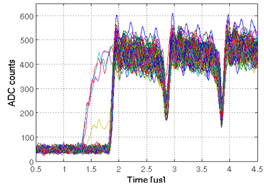
Figure 8: ADC data from the beam injection.
