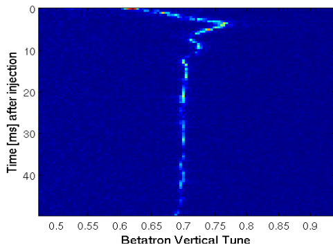
Figure 3: Vertical Tune measurements.
