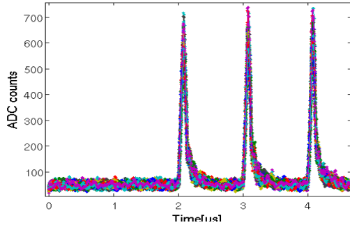
Figure 2: ADC processed data used to synchronize all the units with the beam arrival.
