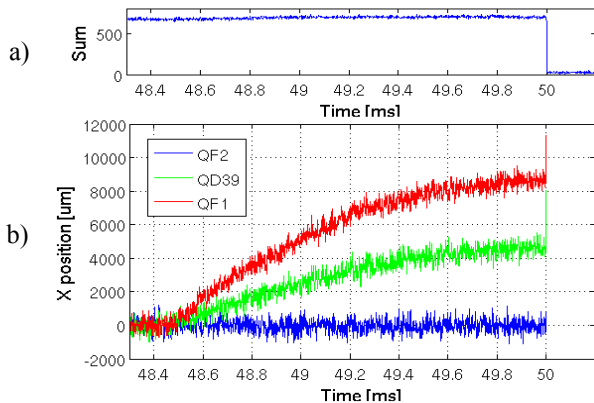
Figure 7.a: SUM signal during the extraction; Figure 7.b: X position signals during the extraction.
