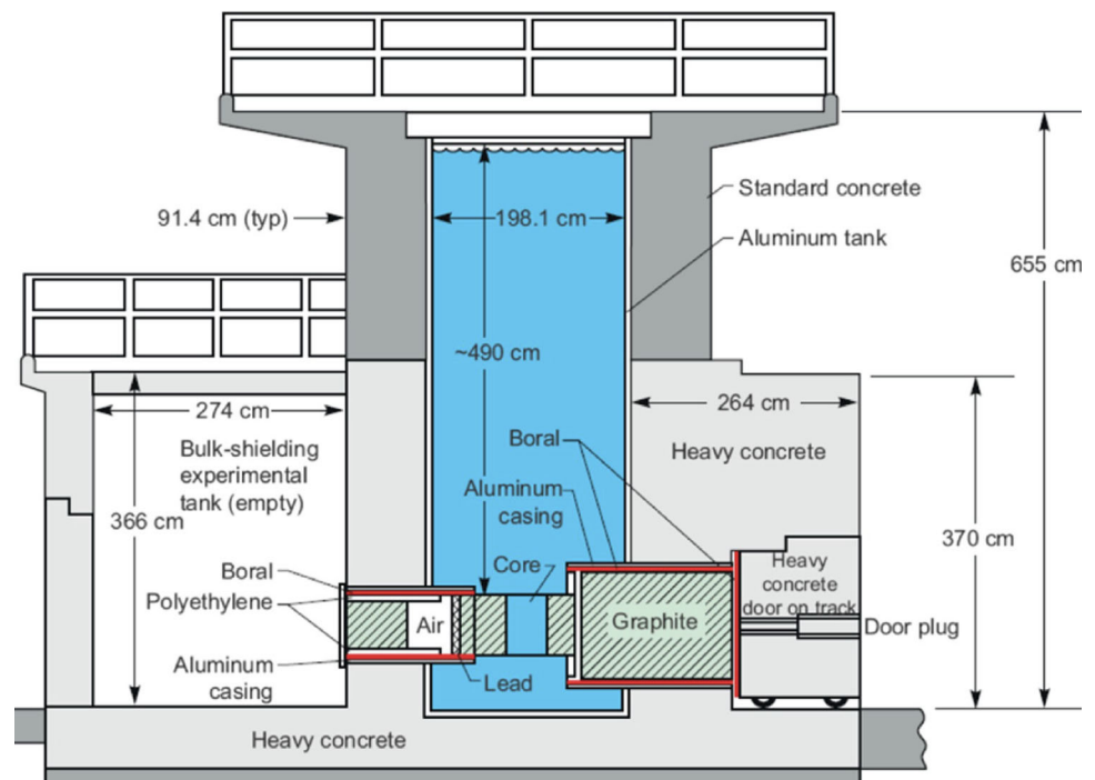
Fig. 1 Side view of the TRIGA MARK II reactor
