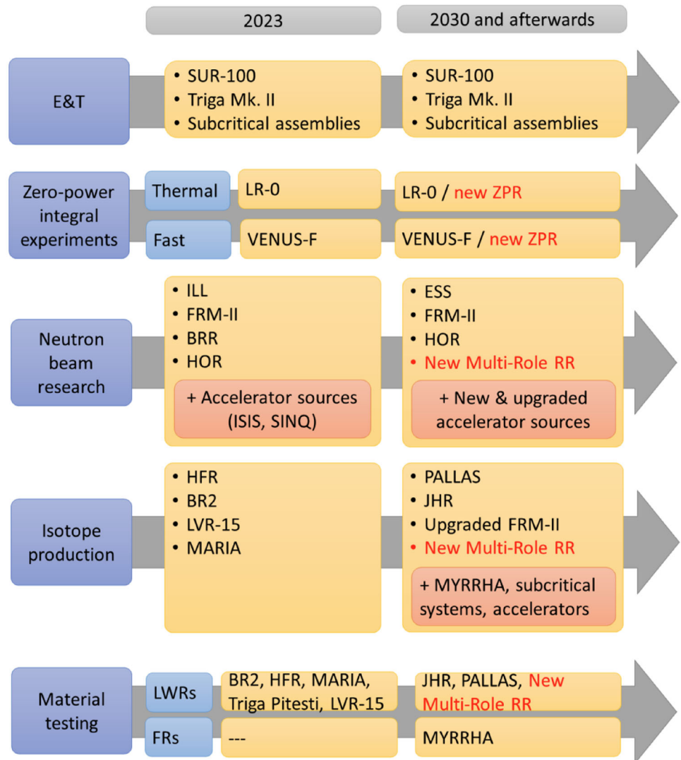
Fig. 5 Current and future European research reactor landscape with the strategy proposed in the scope of the TOURR project [65]. More information regarding the devised strategy can be obtained in project report [75], publicly available on “ https://www.tourr.eu/documents ”
