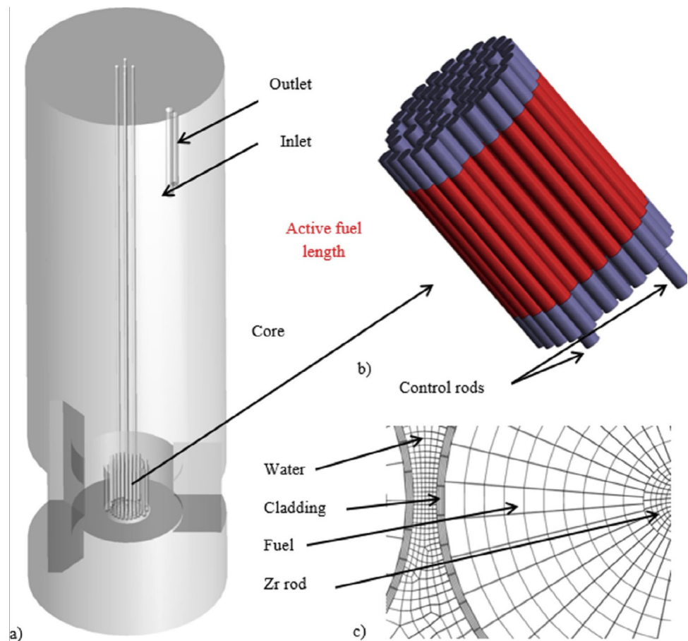
Fig. 2 Development, verification and validation of computer codes: geometry for coupled CFD/Monte Carlo analysis
