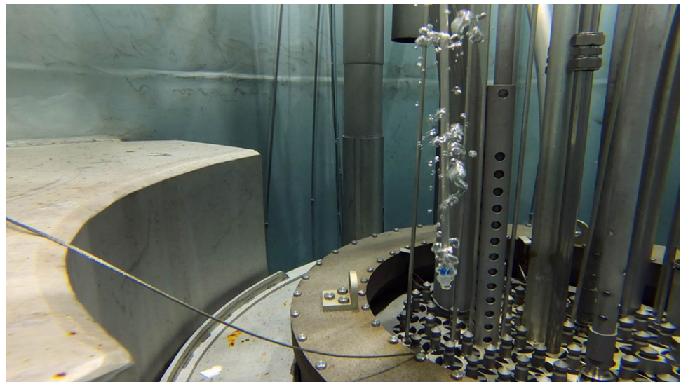
Fig. 3 Bubbles flowing through the core during the void reactivity coefficient experiment
