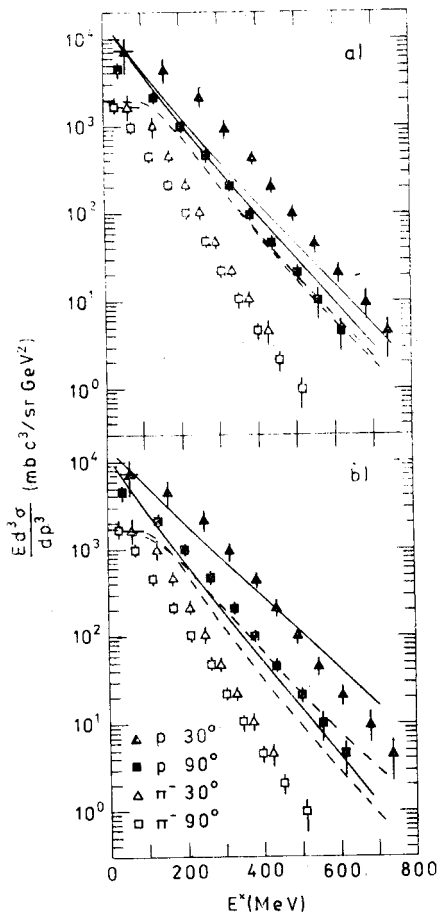
Fig. 2. Particle spectra at 30° and 90° from the two-fireball model compared with experimental results of Ref. [5] for the 800 MeV/nucI Ne on NaF collision. Solid lines — protons. Dashed lines — pions. Fig. 2a corresponds to -\varrho_0 \sigma \Delta p_z = 130 \text{ MeV/c fm} , while Fig. 2b to \varrho_0 \sigma \Delta p_z = 85 \text{ MeV/c fm} . All results are in the c.m. system
