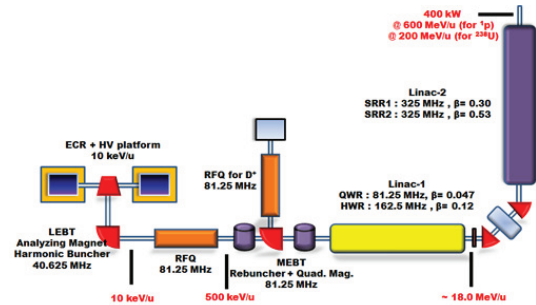
Figure 1: The schematic layout of the driver linac.
