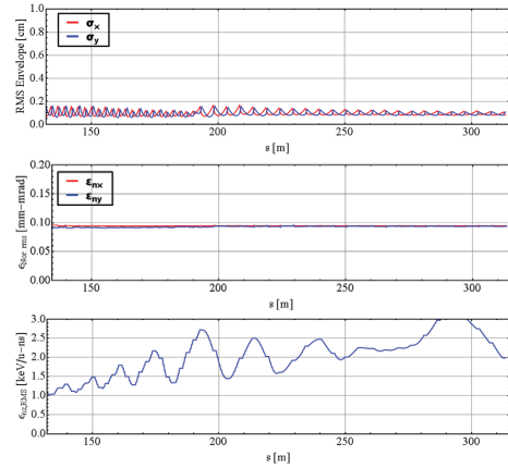
Figure 11: The beam envelope(top), transverse emittance (middle) and longitudinal emittance (bottom) in the high energy linac.
