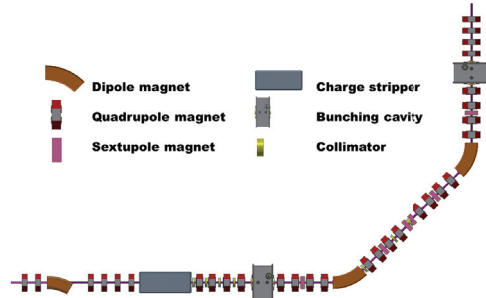
Figure 5: Layout of the charge stripper section of RAON.
