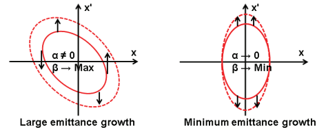
Figure 6: Schematic view to compensate for the emittance growth at the stripper.
