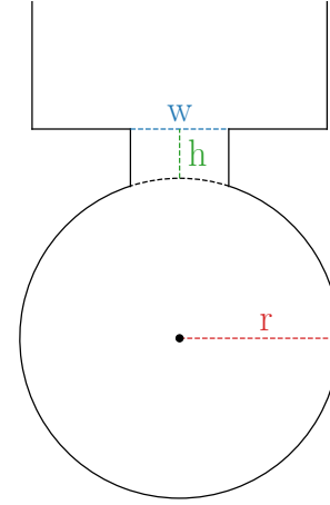
Figure 2: RF coupler geometry from wr284 waveguide to accelerating structure matching cell.
