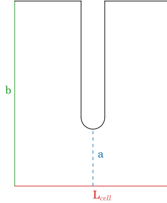
Figure 1: Geometry of a single cell of ECS RF structure with cylindrical symmetry.
