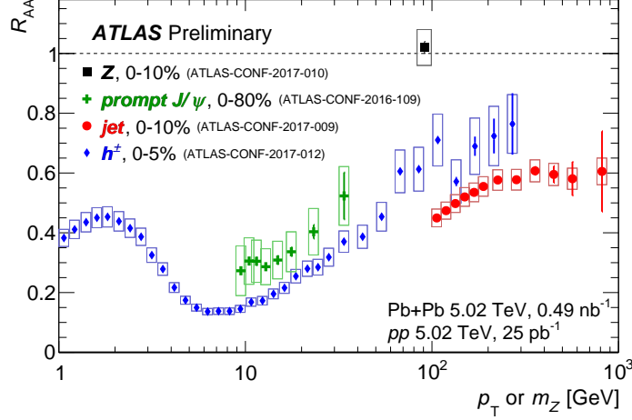
Fig. 1. Compilation of results for the nuclear modification factor R_{AA} vs. p_T or Z boson mass ( m_Z ) in different channels from the Run 2 Pb+Pb and pp data. Results are shown for Z bosons (black squares, plotted at m_Z ), jets (red circles), charged hadrons (blue diamonds) and prompt J/\Psi 's (green crosses). The error bars and shaded bands indicate statistical and systematic uncertainties, respectively. Figure taken from Ref. [1].
