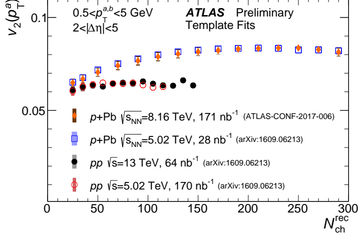
Fig. 2. Comparison of the second-order azimuthal harmonic v_2 obtained from the template fitting procedure in the 13 TeV pp , 5.02 TeV pp , 5.02 TeV p+Pb and 8.16 TeV p+Pb data, as a function of number of charged particles in the event. The error bars and shaded bands indicate statistical and systematic uncertainties, respectively. Figure taken from Ref. [1].
