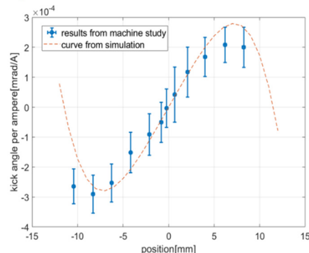
Figure 10: Horizontal survey results of Q-mode.
