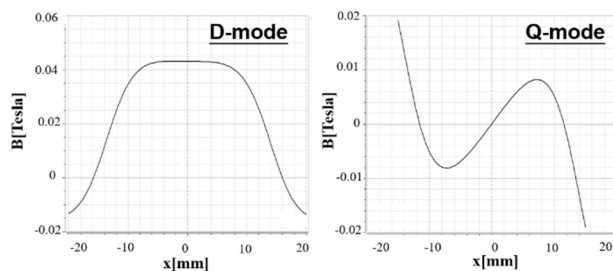
Figure 7: field distribution of D-mode and Q-mode.
