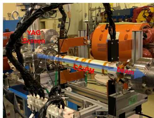
Figure 5: Installation of CCiPM at BT-dump line.
