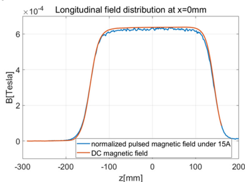
Figure 3: Magnetic field distribution along longitudinal axis.
