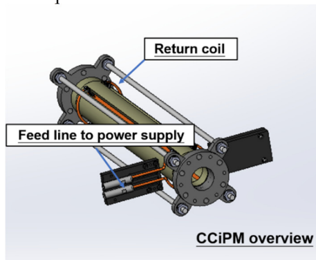
Figure 1: Design figure of CCiPM-D30.
