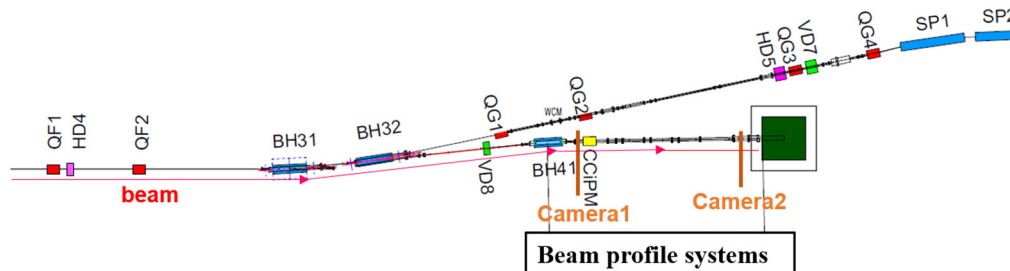
Figure 6: Layout of the monitor system at the BT-dump line.
