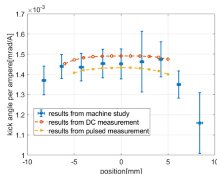
Figure 9: Horizontal survey results of D-mode.
