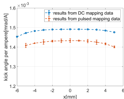
Figure 4: Kick angle calculated from DC and pulsed mapping data.
