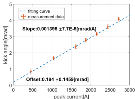
Figure 8: kick effect for current excitation of D-mode.
