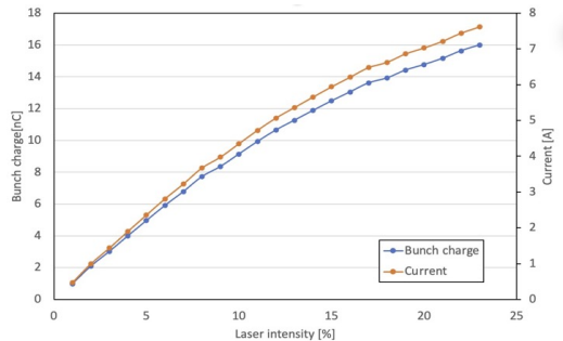
Figure 2: Gun bunch charge and peak current as a function of laser intensity.
