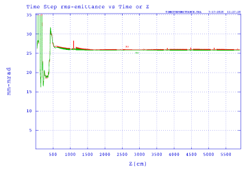
(a) RMS normalized transverse emittance
