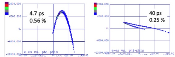
Figure 4: The longitudinal of phase space at exit of LINAC and exit of dechirp cavity. The RMS bunch length and RMS energy spread have been shown in the each plot, respectively.
