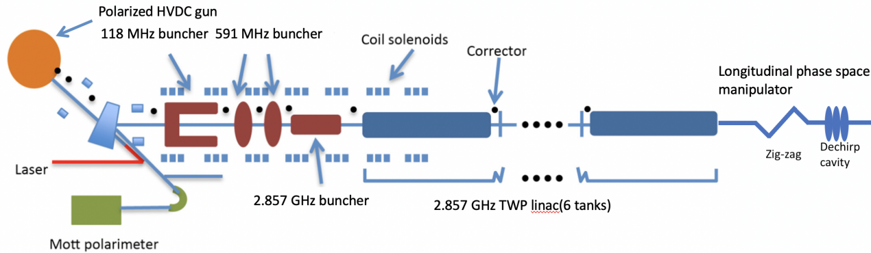
Figure 1: A schematic of the 400 MeV preinjector.
