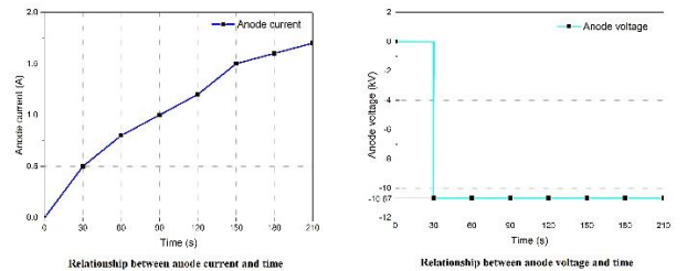
Figure 9: Curves of applied anode voltage and current as the function of time.
