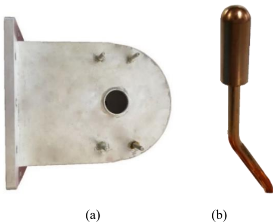
Figure 3: (a)The finished excitation chamber. (b)The finished output coupling antenna.
