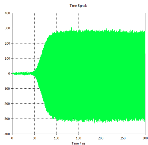
Figure 5: The output signal of the magnetron.
