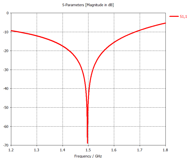
Figure 2: S_{11} of output structure.
