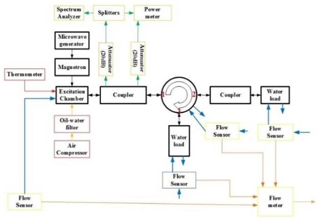
Figure 7: The schematic diagram of the power test of the magnetron.
