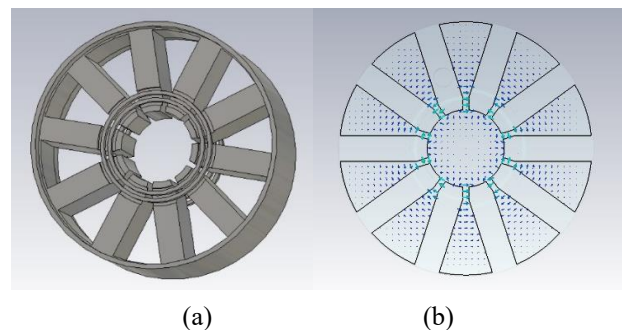
Figure 1: (a) The simulation model. (b) The electric field distribution of the \pi mode.
