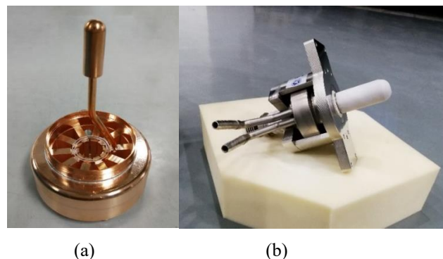
Figure 6: (a)The finished cavity. (b)The prototype of 1.5 GHz CW magnetron.
