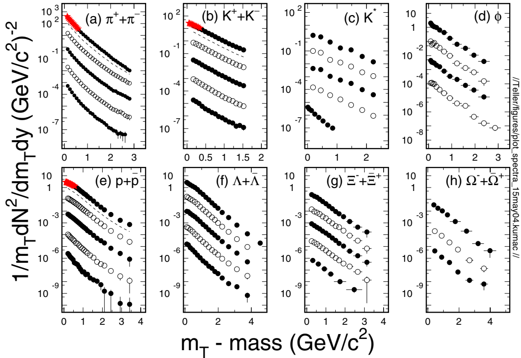
Figure 1. Mid-rapidity hadron spectra from \sqrt{s_{NN}} = 200 GeV Au + Au and p + p collisions. Most and least central collisions are listed from top-down. For pions (a), kaons (b), and protons (e) [4], the centrality bins are: 0-5%, 20-30% ( 10^{-1} ), 40-50% ( 10^{-2} ), 60-70% ( 10^{-3} ), and 80-92% ( 10^{-4} ). The star symbols (0-5%) are data from [5]. The dashed-lines represent the spectra from minimum biased collisions. For K^* (c) [6], from top to bottom, respectively, the centralities are 0-10%, 10-30%, 30-50%, 50-80% for Au + Au collisions and p + p collisions. For \phi -meson (d) [7], the centralities are: 0-5%, 10-30% ( 10^{-1} ), 30-50% ( 10^{-2} ), and 50-80% ( 10^{-3} ). For \Lambda (f) and \Xi (g) [8], the centrality bins are: 0-5%, 10-20% ( 10^{-1} ), 20-40% ( 10^{-2} ), 40-60% ( 10^{-3} ), 60-80% ( 10^{-4} ). For the \Omega baryon (h) [8], the centralities are: 0-10%, 20-40% ( 2 \times 10^{-2} ), and 40-60% ( 10^{-3} ).
