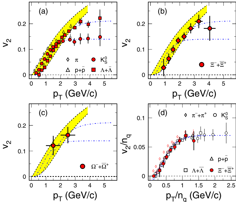
Figure 3. (a) Experimental results of the transverse momentum dependence of the event anisotropy parameters for \pi , K_S^0 , p + \bar{p} , \Lambda + \bar{\Lambda} [30, 29]. Hydrodynamic calculations are shown as thick-dashed-lines. From top to bottom are the results for \pi , K , p , \Lambda , \Xi^- + \Xi^+ , and \Omega^- + \Omega^+ ; Multi-strange baryon elliptic flow v_2 are shown in (b) for \Xi and (c) for \Omega . Plots (b) and (c) are from preliminary STAR results [8, 32]. (d) Number of constituent quark ( n_q ) scaled v_2/n_q versus scaled p_T/n_q . All curves are from [33].
