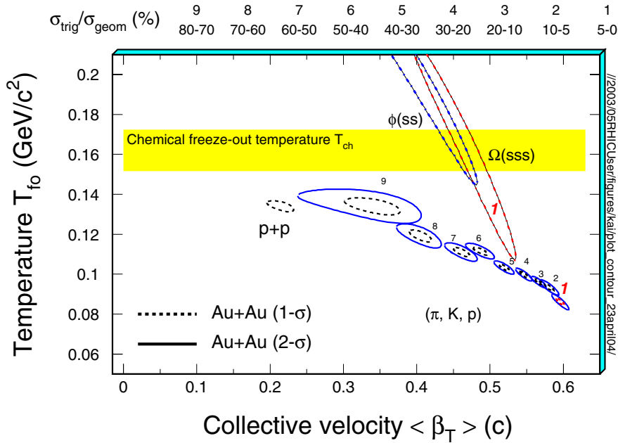
Figure 2. \chi^2 contours, extracted from the thermal+radial flow fits, for copiously produced hadrons \pi, K and protons and multi-strange hadrons \phi and \Omega . On the top of the plot, the numerical labels indicate the centrality selection. For \pi, K and protons, 9 centrality bins (from top 5% to 70-80%) were used from 200 GeV Au+Au collisions. The results from 200 GeV p + p collisions are also shown. For \phi and \Omega , only the most central results are presented. Dashed- and solid-lines are the 1- \sigma and 2- \sigma contours, respectively.
