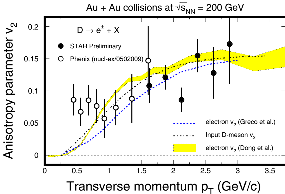
Figure 4. Non-photon electron elliptic flow v_2(p_T) from minimum bias Au + Au collisions at \sqrt{s_{NN}} = 200 GeV. Data from PHENIX [43] and STAR [45] experiments are shown as open- and filled-circles, respectively. Only statistical errors are shown. Dashed-line and the hatched band are charm-hadron decayed electron v_2(p_T) from refs. [33, 38].
