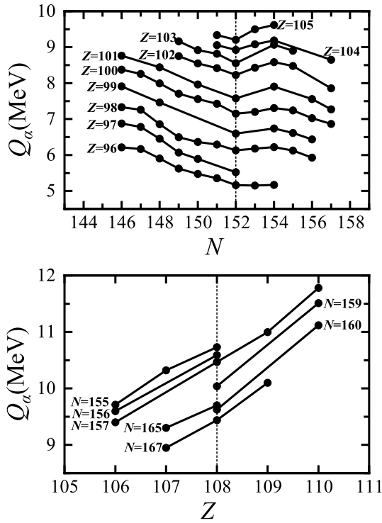
Fig. 1. Experimental \alpha -decay energy Q_\alpha are provided for (a) Z = 96 - 105 isotopic chains and (b) some N = 155 - 167 isotonic chains. The experimental data are obtained from the atomic mass table of Wang et al [46].
