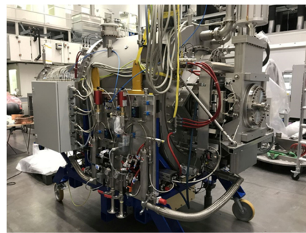
Figure 3: The first SC cavity cryomodule parked in a testing area for the FAT.
