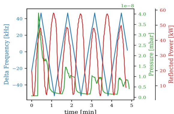
Figure 6: Cavity outgassing during RF frequency sweep conditioning.
