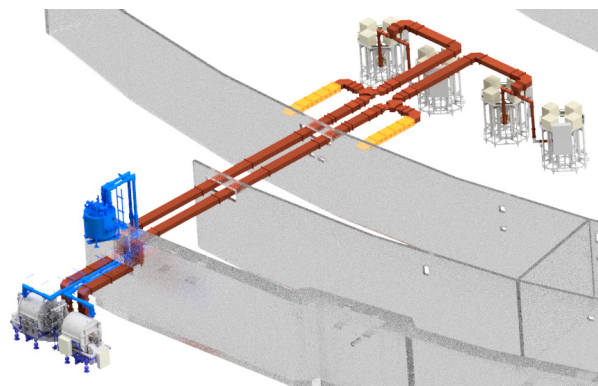
Figure 2: Layout of the RF system for the SC cavities in Phase 2.
