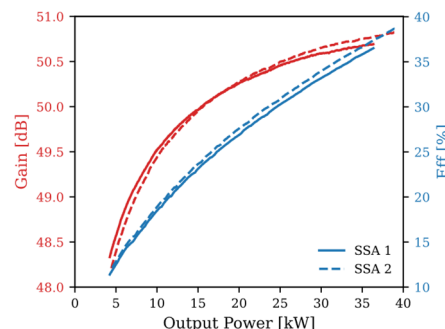
Figure 4: Sirius RF SSA towers efficiency and gain.
