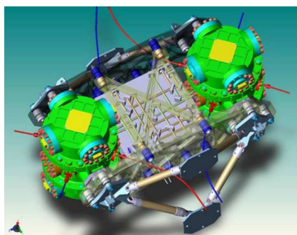
Figure 5. LTP core assembly. Two vertical Zerodur plates hold the optical bench and the two vacuum tanks containing the test masses. Laser light from the optical bench is reflected on the test masses allowing the interferometrical determination of their position fluctuations.
