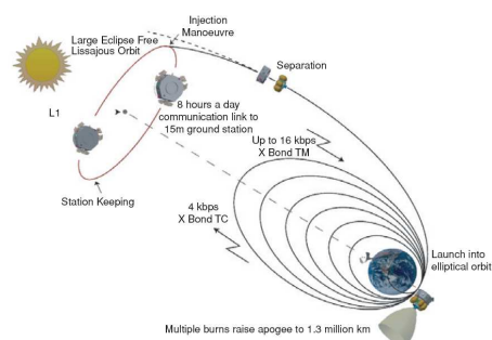
Figure 4. LISA Pathfinder will orbit the first Lagrange point.
