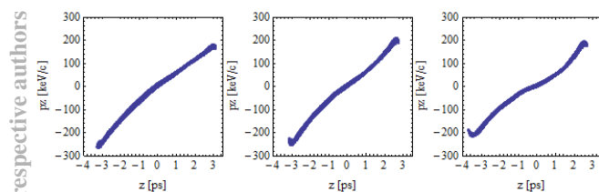
Figure 4: Longitudinal phase space at the exit of the CLARA first linac for gun first cell lengths of 0.4, 0.5, and 0.6 of the second cell (left to right).
