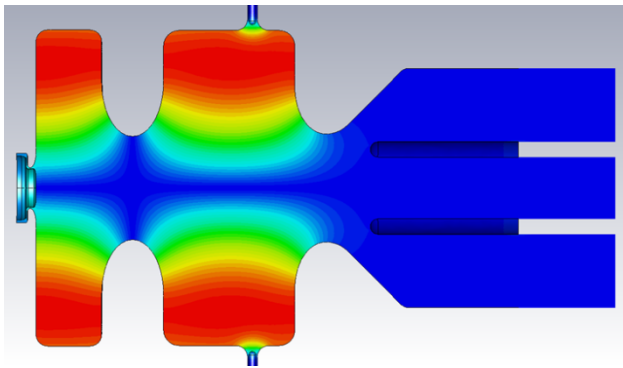
Figure 7: Magnetic field distribution.
