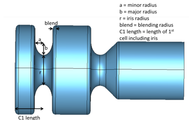
Figure 2: Parameterised 2D gun cavity model.
