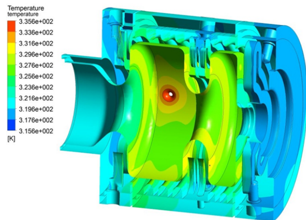
Figure 9: Temperature increases with the proposed cooling system with the gun operating at 100 MV/m at a 400 Hz repetition rate.
