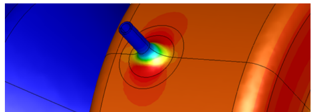
Figure 5: Magnetic field distribution around the RF probe.
