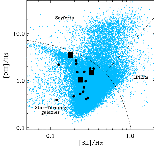
Figure 2.1: Emission-line diagnostic diagram displaying the [SII]/H\alpha versus [OIII]/H\beta line ratios of a large sample of galaxies, selected from the SDSS catalogue. Among these galaxies are the three sources being studied in this work, whose flux ratios are represented by the filled squares. The filled circles represent the flux ratios of the 16 remaining sources from the cross-correlation of SDSS and 2XMMp that were selected for their high X-ray luminosity (i.e., a luminosity > 10^{42} erg s ^{-1} ). The dot-dash curves represent the Kewley et al. (2001) theoretical maximum starburst line. The dashed line represents the Kauffman et al. (2003) border between the diagrams' LINER and Seyfert regions. The blue dots represent the line ratios of a large sample of galaxies, selected from the SDSS -DR7 catalogue.
