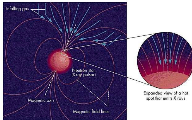
Figure 1.20: A cartoon of the accretion process X-ray pulsar systems. Taken from http://www.mhhe.com/ .
