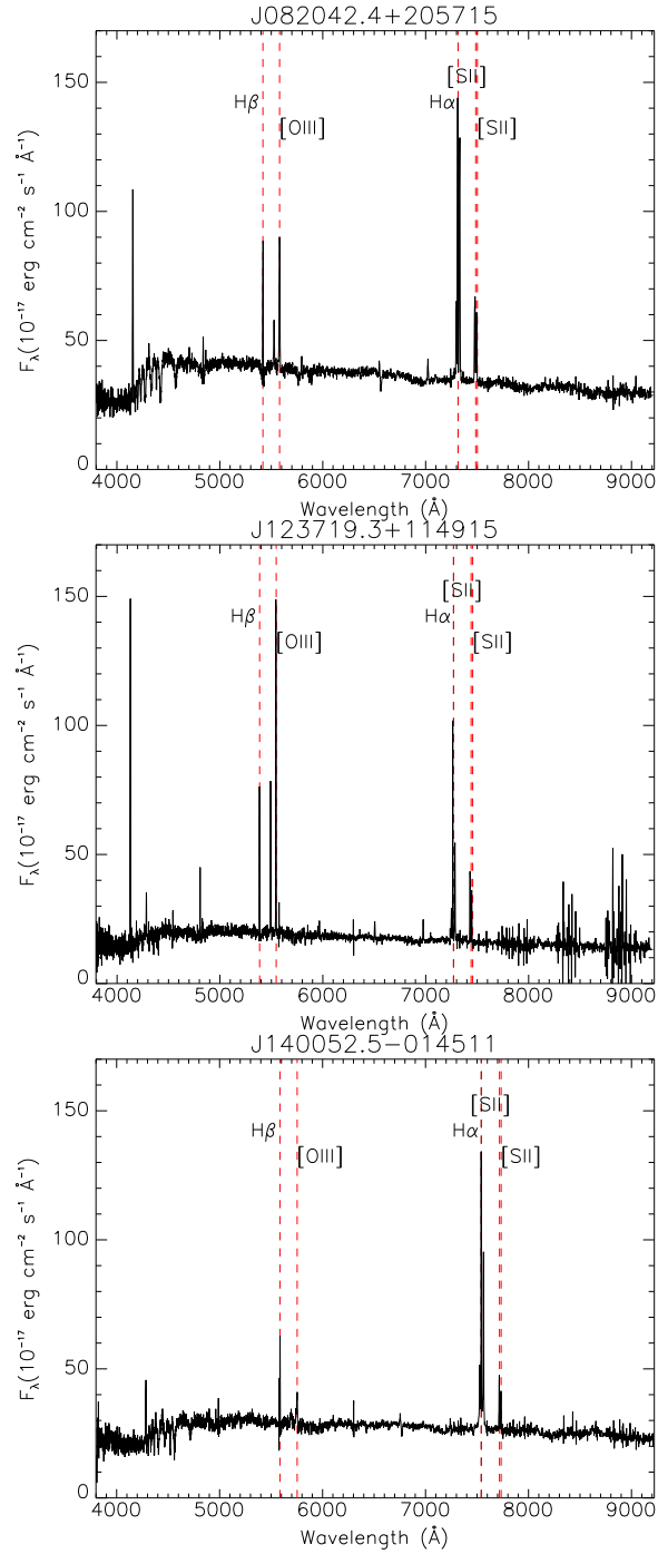
Figure 2.2: SDSS -DR7 optical spectra of J082042.4+205715 (top), J123719.3+114915 (middle), and J140052.5-014511 (bottom). None of the spectra show strong signs of AGN activity. Also, signatures for star formation, such as the presence of dominant narrow H \alpha and H \beta emission lines, can be seen within these spectra, indicating the existence of star forming activity within the sources' nuclei.
