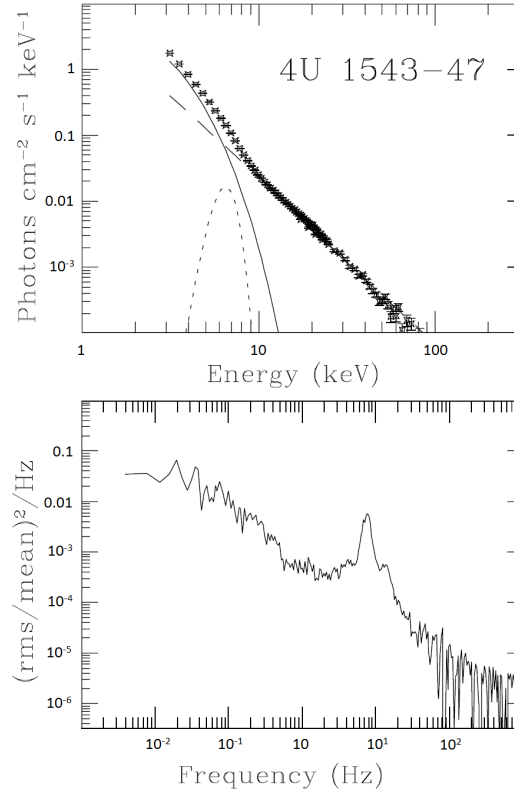
Figure 1.18: Top : A spectrum of the BHB 4U 1543-475 accreting in the SPL state, which is characterised by a steep power-law component. Bottom The PDS of the same source accreting in the SPL state. A QPO is clearly visible in the PDS. Both images taken from McClintock & Remillard (2006).
