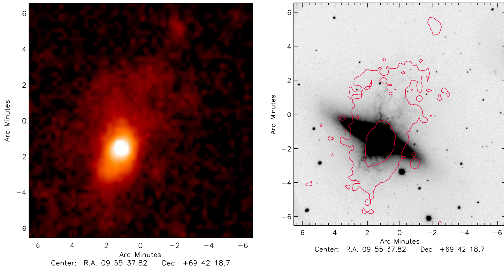
Figure 4.1: Left: A 0.1 – 2.4 keV ROSAT PSPC image of M82, created using data from an observation in 1991. Right: A KNPO H\alpha image of M82. Overlaid onto this image are contours representing the X-ray emission at photon count levels of 1 and 2 cts \text{pix}^{-1} . These contours were created using the ROSAT image in the left hand panel.
