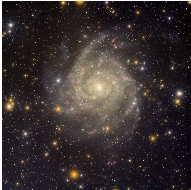
Figure 1.2: An optical image of IC 342, taken with the Mayall 4 m telescope in late 2006. This nuclear starburst shows evidence of star formation in the central \sim 100 pc region of the galaxy (e.g., Telesco et al. 1993). Image credited to T.A. Rector/University of Alaska Anchorage, H. Schweiker/WIYN and NOAO/AURA/NSF. Taken from http://www.noao.edu .
