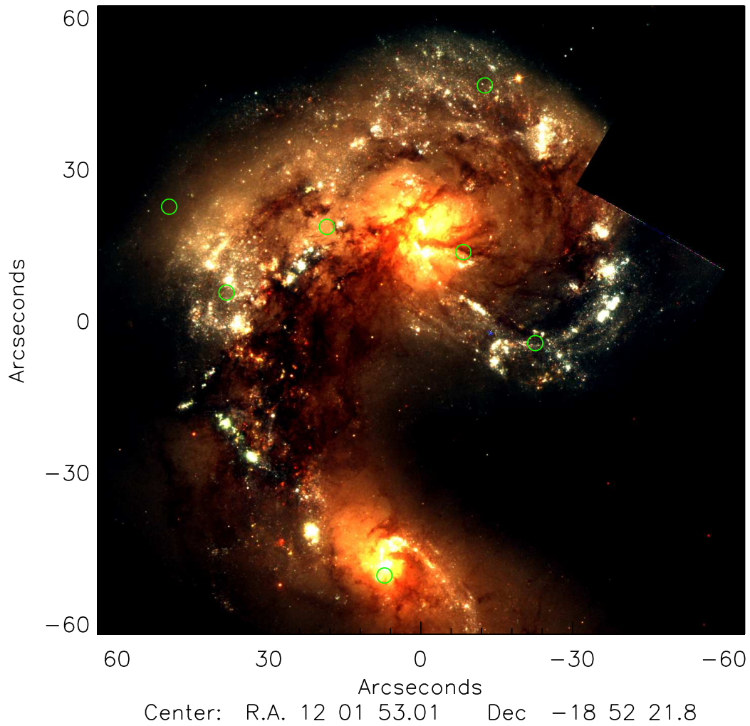
Figure 3.11: A 3-colour image of the Antennae galaxy system, created using HST WFC2 F439, F555, and F814 observations of the galaxy that were taken in January 1996 (PI Whitmore). The locations of the 7 ULXs identified by Rangelov et al. (2011) are represented by the green circles.
