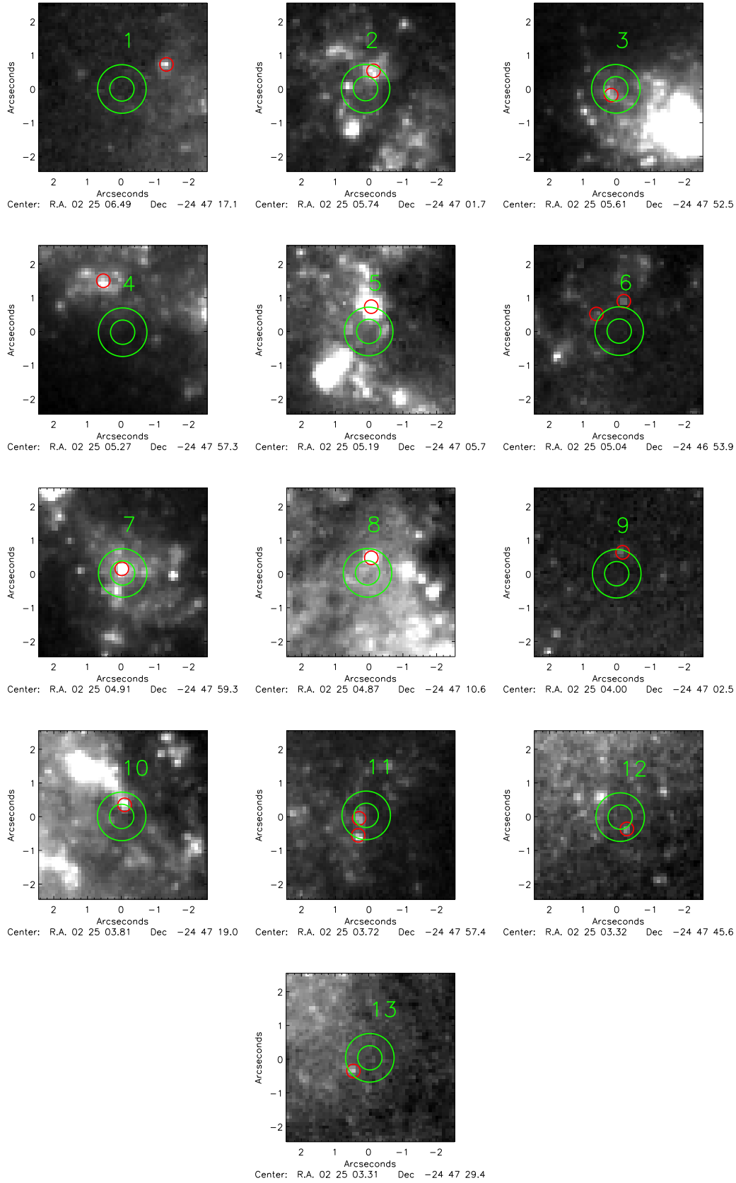
Figure 3.5: F439W-band images of the regions of NGC 922 containing the 13 X-ray binaries associated with stellar sources. These images were created using the HST F555W image of the galaxy. The green circles represent the 1.5 \sigma and 3 \sigma positional uncertainties of the X-ray sources. The smaller red circles represent the positions of the associated stellar clusters and stars. The orientation of the images is the same as that in Figure 3.4.
