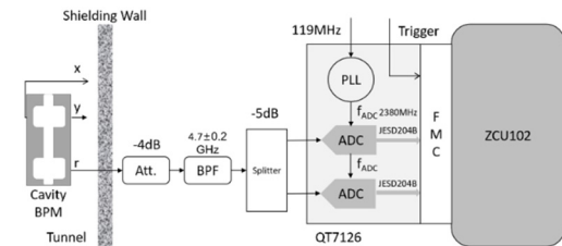
Figure 6: Test block diagram of RF processor.
