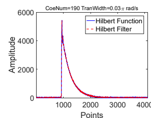
Figure 10: Envelope of cavity BPM signal.
