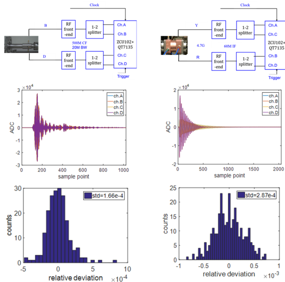
Figure 2: Relative resolution evaluations of stripline BPM(left) and cavity BPM(right) electronics on SXFEL beam.
