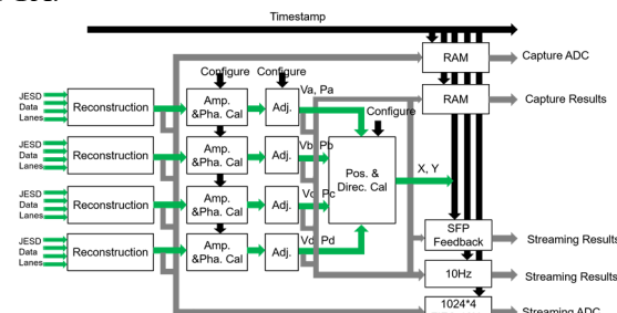
Figure 8: Block diagram of digital signal processing.
