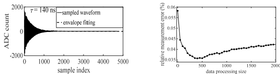
Figure 7: Sampled cavity BPM signal waveform(left) and relative resolution VS. data processing size(right).
