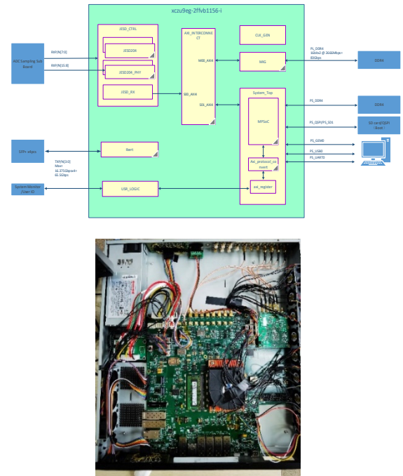
Figure 3: Block diagram(up) and picture(bottom) of the new developed processor.
