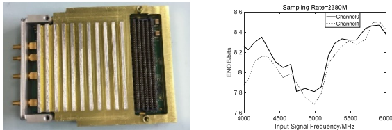
Figure 5: Direct RF sampling ADC card(left) and the ENOB result(right).
