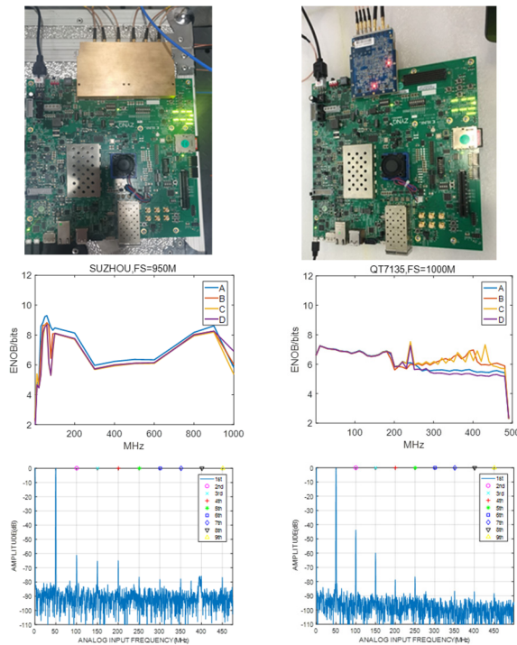
Figure 1: Lab evaluation of domestic(left) and abroad(right) ADCs.
