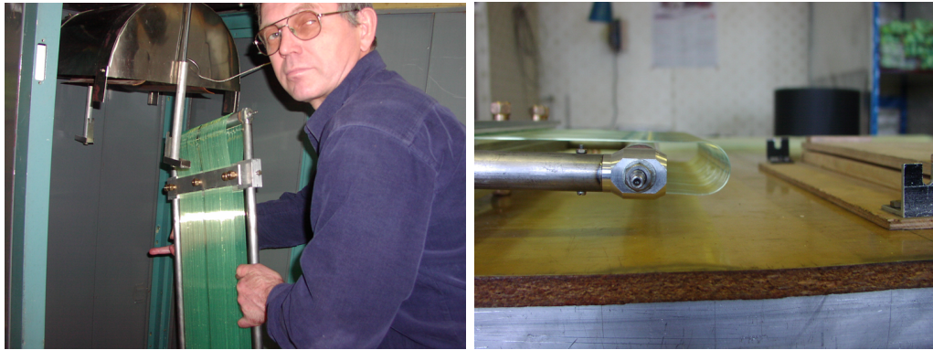
Figure 3.32: Preparation of fiber loops. Placing the frame in the oven, delivering uniformly distributed heat (left), and extraction of bent fibers from the frame (right)
