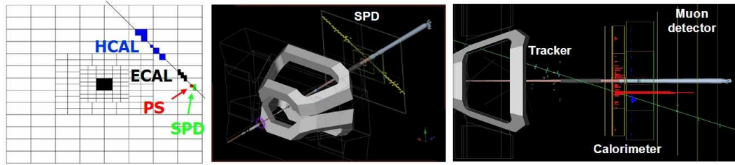
Figure 3.44: Projection of the cosmic particle track reconstructed in the calorimeter detectors (left), a rare cosmic particle track fully contained in SPD (center) and the example of the track triggered with calorimeter and reconstructed in the tracking system and muon detector stations (right)
