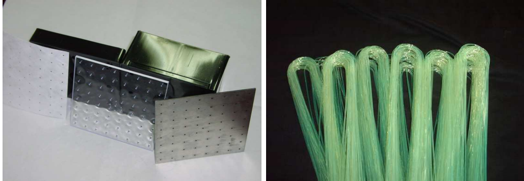
Figure 3.10: Components of the ECAL module stack, scintillator tiles, lead plates, TYVEK paper, fiber loop and fiber bundle plastic housings (left), WLS fiber loops (right)
