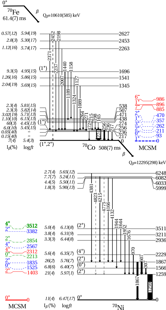
Fig. 2. (Color online.) Experimental and calculated level schemes of the decay ^{70}\text{Fe} \rightarrow ^{70}\text{Co} \rightarrow ^{70}\text{Ni} . Arrow widths are proportional to transition intensities. Transitions shown by dashed arrows are placed based only on energy-matching constraints. Apparent \beta feedings ( I_\beta ) and \log ft values (calculated assuming the lowest-lying level as the ground state) are shown. MCSM states predicted to be nearly spherical or slightly prolate-deformed ( \beta_2 \leq 0.2 ) are indicated in solid red, strongly prolate-deformed ( \beta_2 > 0.2 ) in dashed blue, and oblate-deformed ( \beta_2 \sim -0.13 ) in dotted-dashed green. Q_\beta values are taken from [33].
