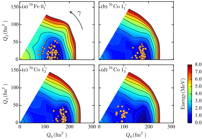
Fig. 3. (Color online.) Potential energy surface (PES) plots for (a) the 0^+ ground state of ^{70}\text{Fe} and (b)–(d) the 1^+ states of ^{70}\text{Co} . See the text for orange circles ( T -plot).
