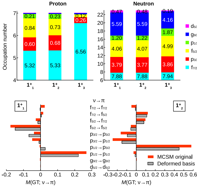
Fig. 4. (Color online.) Top: Occupancies of single-particle orbitals in the MCSM calculation for the 1^+ levels of ^{70}\text{Co} . Bottom: Gamow-Teller matrix elements for the 0^+ \rightarrow 1^+_1 (left) and 0^+ \rightarrow 1^+_2 (right) transitions. Filled and shaded bars represent the results of the original MCSM calculation and the deformed bases, respectively (see text). The latter are not multiplied by a quenching factor.
