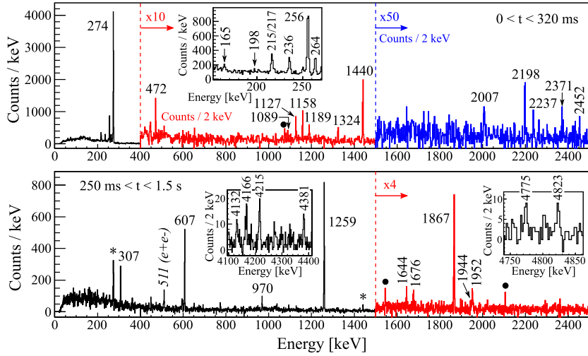
Fig. 1. (Color online.) Delayed \gamma spectra following \beta decay of ^{70}\text{Fe} . The time intervals 0–320 ms (top) and 250–1500 ms (bottom) are selected to enhance \gamma rays in ^{70}\text{Co} and ^{70}\text{Ni} , respectively. Transitions placed in the level schemes are labeled by their energies, unplaced \gamma rays are marked by circles, and transitions assigned to the progenitor are indicated by asterisks. Long-living background components have been subtracted. Inset panels: Parts of spectra zoomed in on energy regions where weak \gamma rays are observed.
