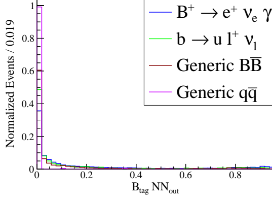
(a) Electron channel in the whole range.
