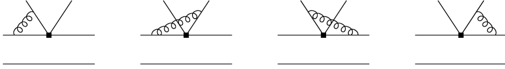
Figure 2.3: Leading order Feynman diagrams where the gluon attaches the bottom quark and the quarks of the emitted meson [1].
