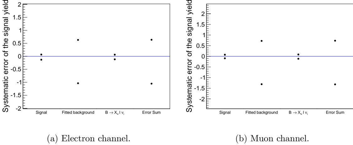
Figure 7.7: Systematic error of the PDF shape uncertainties separated for each fit component.
