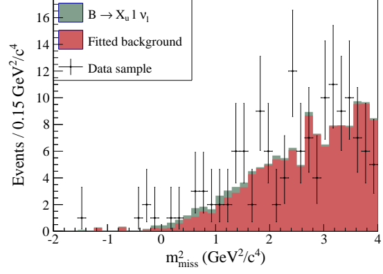
(b) Electron channel in the sideband satisfying M_{bc} < 5.27 \text{ GeV}/c^2 and n_{\text{out}} > 0.25 .
