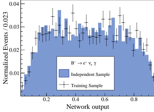
(a) Electron channel signal MC.
