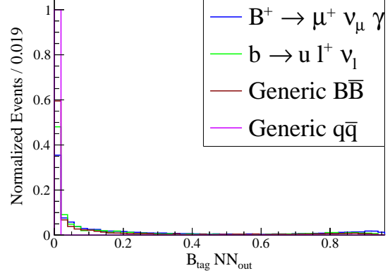
(b) Muon channel in the whole range.
