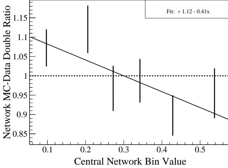
Figure 7.6: Double ratio in bins of the network output calculated with the B^+ \rightarrow K^*(892)\gamma signal MC and the sPlot subtracted data sample. A linear fit is used to obtain the deviations in the individual network output bins.
