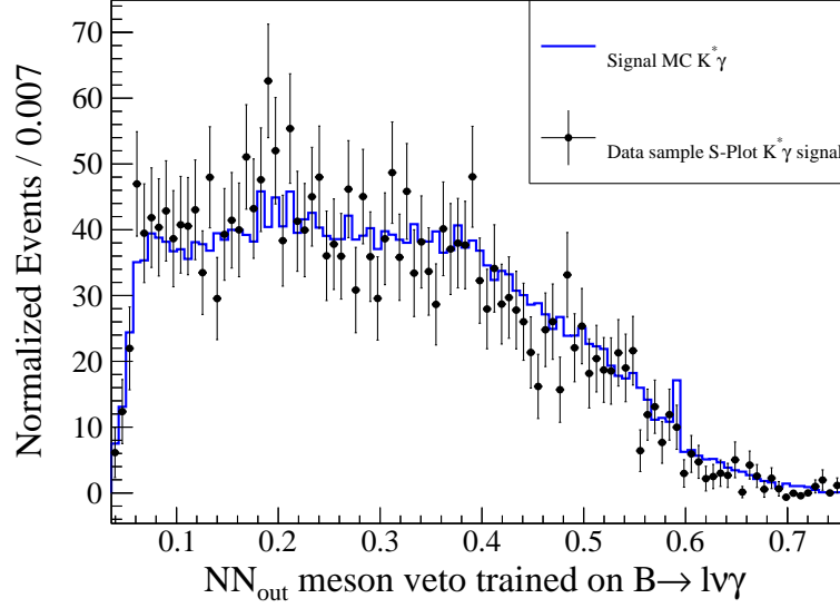
Figure 7.5: Network output distribution for sPlot subtracted data and B^+ \rightarrow K^*(892)\gamma signal MC. The training is performed on the B^+ \rightarrow \ell^+\nu_\ell\gamma MC samples where only with meson masses are used.
