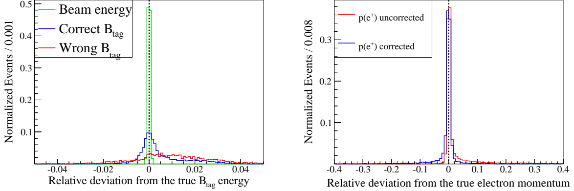
(a) Deviation of the true B_{\text{tag}} energy from the beam energy, and the reconstructed energy of wrong and correct tag-side candidates.
