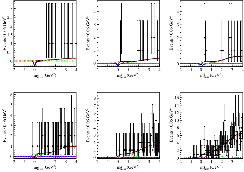
Figure 5.14: Fit of a toy sample generated without signal. A negative signal yield is fitted which is large enough to cause the total PDF to be negative in the signal-like n_{\text{out}} bins.
