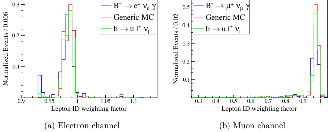
Figure 4.24: Event weights correcting the data-MC efficiency difference in the lepton ID.
