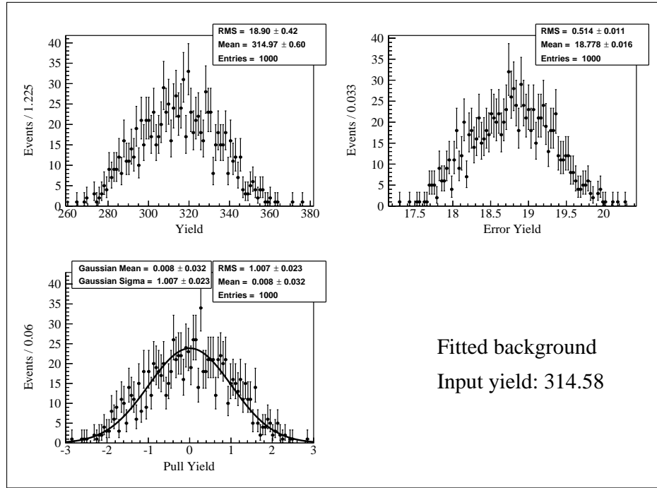
(a) Electron channel.
