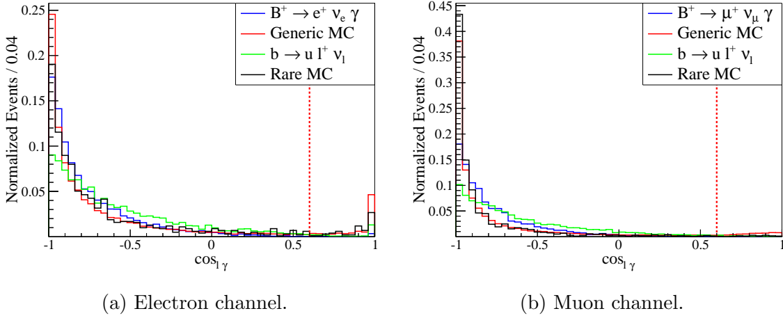
Figure 4.8: \cos \Theta_{\gamma\ell} angle which is selected to be below 0.6.
