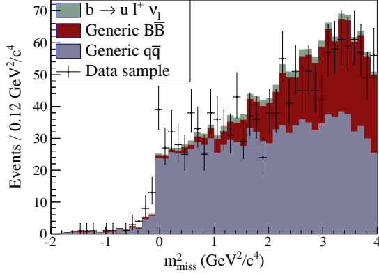
(a) Muon channel before requiring high p_{\text{miss}} .
