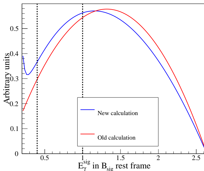
Figure 2.7: Photon energy spectrum for the latest next-to-leading order calculation from Ref. [9] and an leading order calculation from Ref. [11] without detector simulation. The difference between the curves is used as a measure of the systematic model uncertainty. The vertical lines show two energy thresholds at 400 MeV and 1 GeV which are used for the nominal and secondary analysis, respectively (see section 3.2.1).
