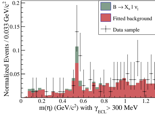
(a) Elec. channel: fitted background SB.
