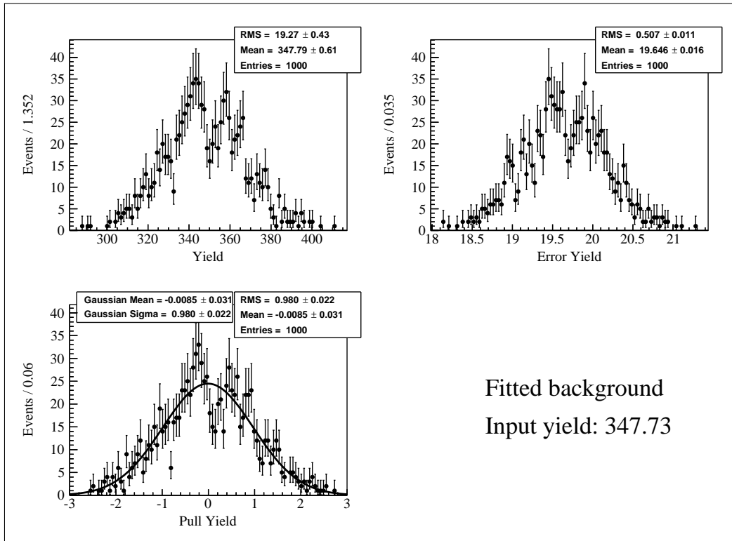
Figure 5.11: Toy study result for the muon channel with a signal branching fraction of 5 \times 10^{-6} . See Fig. 5.9 for a description of the plot.
