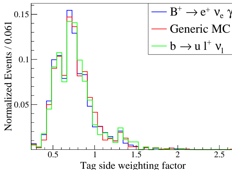
Figure 4.23: Event weights correcting for data-MC tag-side efficiency differences which are determined in [31]. The weights depend on the tag-side decay mode and the B_{\text{tag}} network output.
