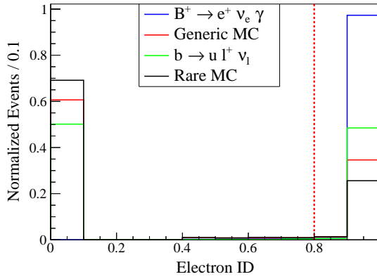
(a) Electron ID.
