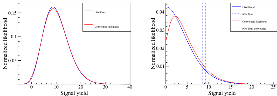
(a) The significance decrease after convolution, since the maximum likelihood decreases and the value of the null hypothesis at zero increases.
