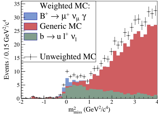
(c) Muon channel expected events.
