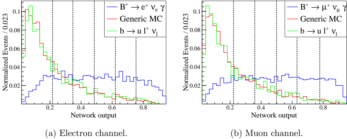
Figure 4.20: NN output for the independent MC samples. The vertical lines indicate the bin boundaries used for the binned fit described in section 5.
