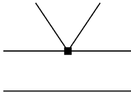
Figure 2.1: Feynman diagram showing the naive factorization approach of the B meson decaying into two mesons. Any exchange of gluons between the high-momentum meson M_1 and the (BM_2) system is assumed to be negligible. The Feynman diagrams in this section show in the lower line the spectator quark of the B meson and in the upper line the bottom quark. The non-horizontal lines show the quarks of the meson which is emitted from the weak decay [1].
