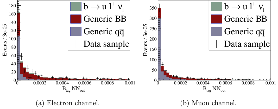
Figure 4.16: B_{\text{tag}} NN output with event shape variables in the side band of M_{bc} < 5.27 \text{ GeV}/c^2 . A good agreement between data and MC can be seen for both channels.
