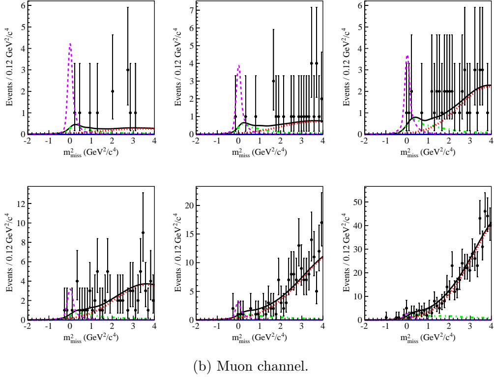
Figure 8.2: Measurement for the secondary analysis with the fit of the m_{\text{miss}}^2 in six bins of n_{\text{out}} on data. See description Fig. 8.1
