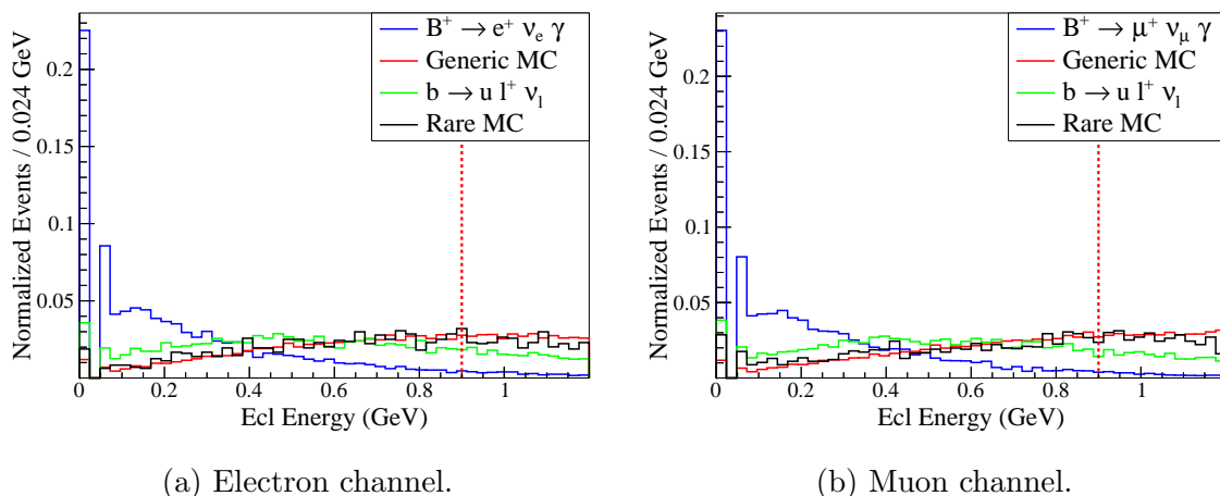
Figure 4.7: Extra energy in the ECL which is required to be below 900 MeV.
