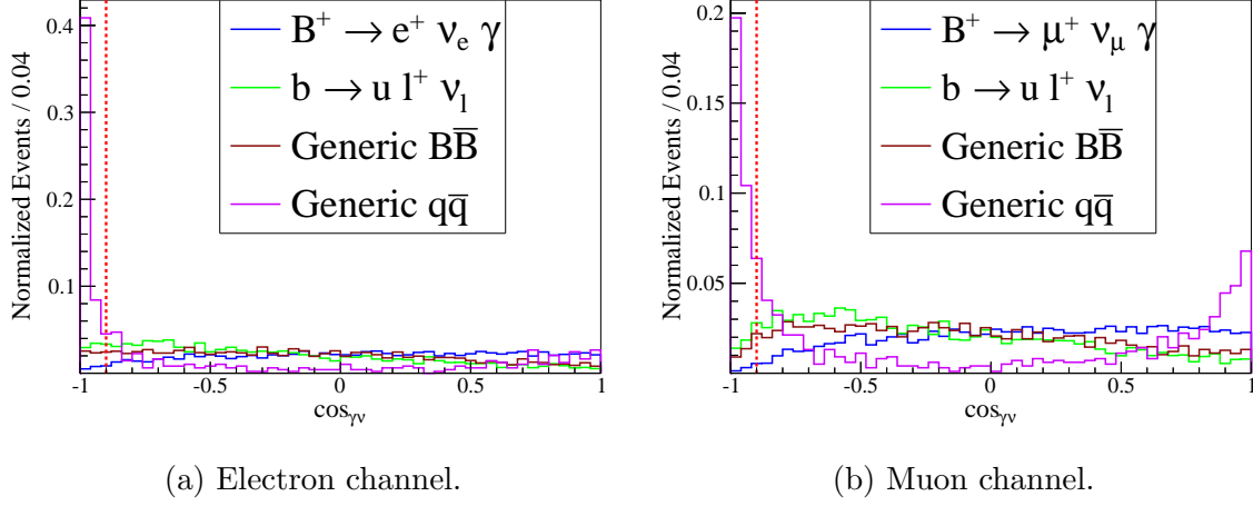
Figure 4.14: \cos \Theta_{\gamma\nu} angle which is selected to be larger than -0.9 .
