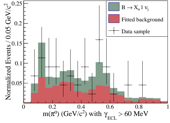
(b) Elec. channel: B \rightarrow X_u \ell^+ \nu_\ell enriched SB.
