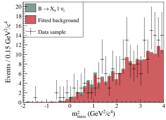
(d) Muon channel in the sideband satisfying M_{bc} < 5.27 \text{ GeV}/c^2 and n_{\text{out}} > 0.25 .
