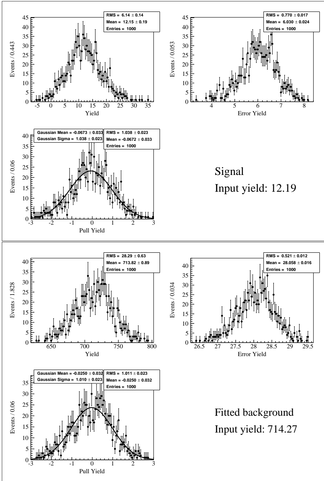
Figure 1.15: Toy study result for the fit in six bins of n_{\text{out}} for the muon channel
