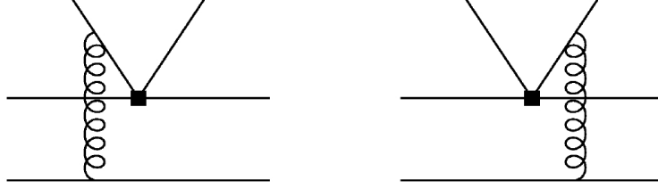
Figure 2.4: Higher-order Feynman diagrams showing the spectator scattering which is a correction of \mathcal{O}(\alpha_s) to the leading order term. Here, the constituents of the emitted meson exchange a gluon with the spectator quark [1].
