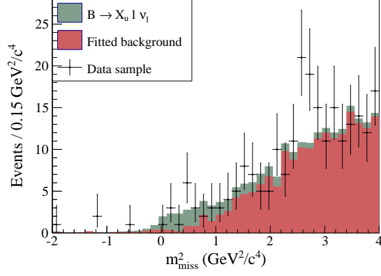
(a) Electron channel in the sideband satisfying M_{bc} > 5.27 \text{ GeV}/c^2 and n_{\text{out}} < 0.25 .
