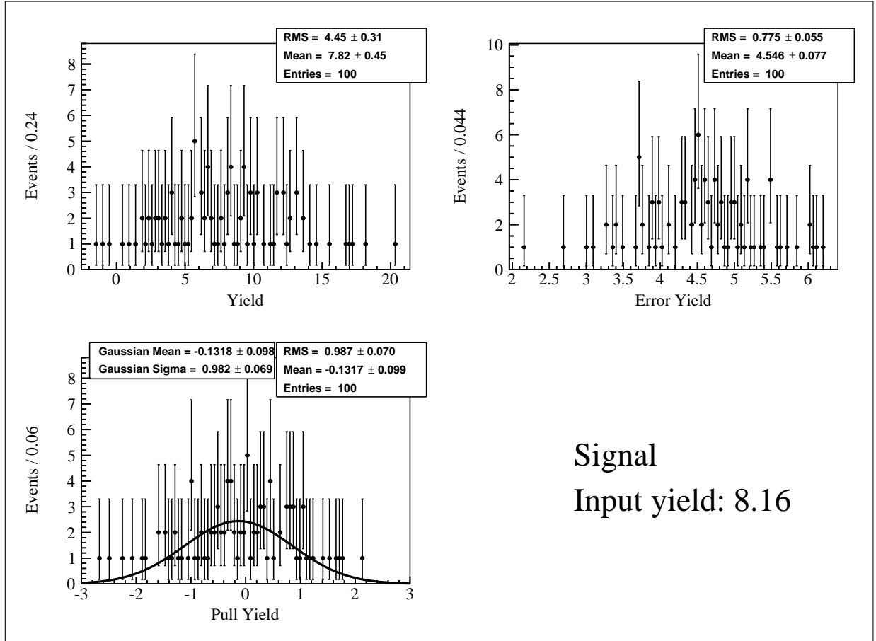
Figure 1.16: Toy study sampled from MC for the m_{\text{miss}}^2 fit in six bins for the electron channel of the nominal analysis.
