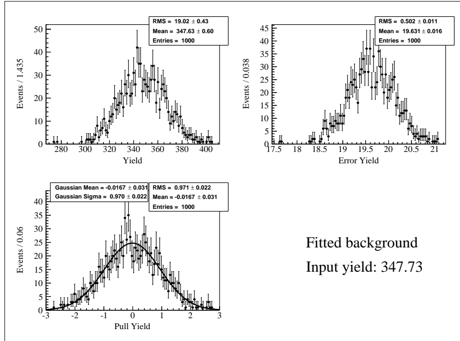
(b) Muon channel.
