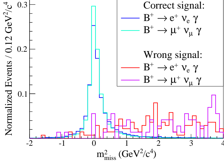
Figure 3.4: Comparison of m_{\text{miss}}^2 for correctly and wrongly matched signal MC for both signal channels. The distributions peak only for correctly matched MC.
