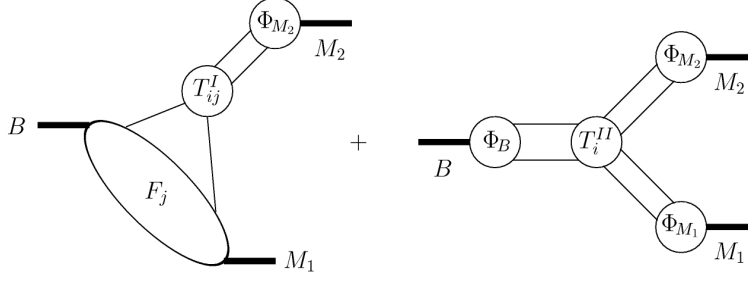
Figure 2.2: Graphical representation of the factorization formula given in Eq. 2 with its two factorization topologies [1].
