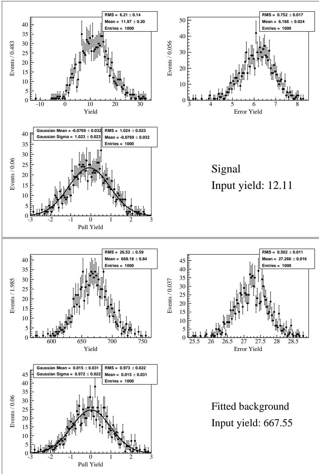
Figure 1.14: Toy study result for the fit in six bins of n_{\text{out}} for the electron channel
