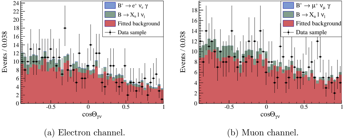
Figure 1.19: \cos \Theta_{\gamma\nu} angle in the signal region.
