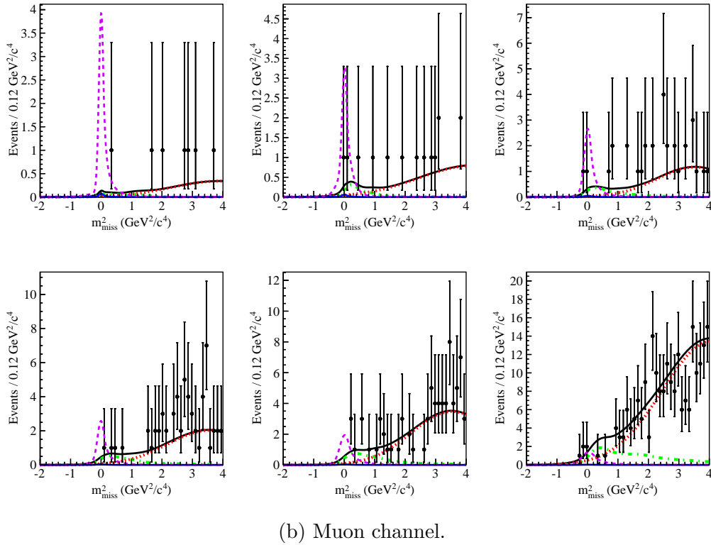
Figure 8.1: Measurement of the nominal analysis with the fit of the m_{\text{miss}}^2 in six bins of n_{\text{out}} on data (points with error bars). Shown are the PDFs for: the signal (blue), enhanced signal (dashed violet), fixed B \rightarrow X_u \ell^+ \nu_\ell backgrounds (green), fitted backgrounds (red), and the sum (black). The enhanced signal function, which has the same normalization for each bin, corresponds to a branching fraction of 30 \times 10^{-6} . The most signal-like bin is found in the upper left plot. Proceeding from left to right, the distributions become increasingly more background-like and the most background-like bin is shown in the lower right panel.
