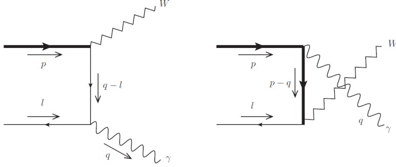
Figure 2.6: Feynman diagrams for the tree decay contributions. The left diagram shows the leading order term where the photon is emitted by the up quark. Here, the propagator joining the W and photon vertex is light. The bottom quark emission in the right diagram is suppressed since the propagator is now heavy [9].
