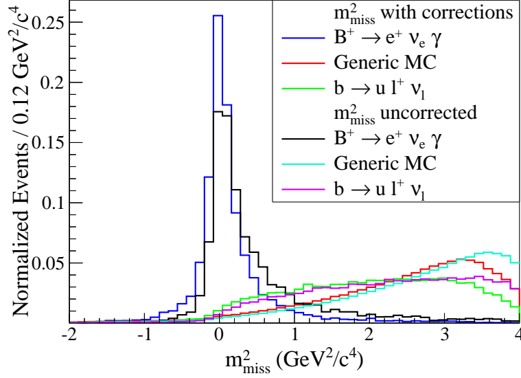
Figure 4.3: Comparison of m_{\text{miss}}^2 distributions with and without beam energy and bremsstrahlung correction for correctly identified signal MC of the electron channel. The most important background sources of b \rightarrow u \ell^+ \nu_\ell , generic B\bar{B} and q\bar{q} continuum decays are also shown.
