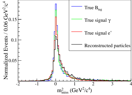
(b) m_{\text{miss}}^2 distribution for signal MC of the electron channel, where one of the input four-vectors for the m_{\text{miss}}^2 calculation is set to the MC truth and the remaining ones are taken from the reconstruction. All particles of signal and tag-side are selected to be correctly identified.
