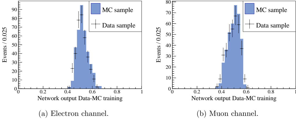
Figure 6.12: Network output obtained by training data against MC.
