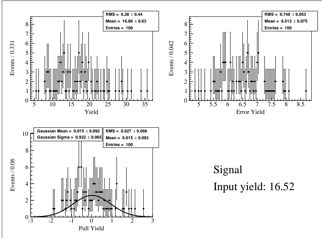
(b) Simultaneous fit.
