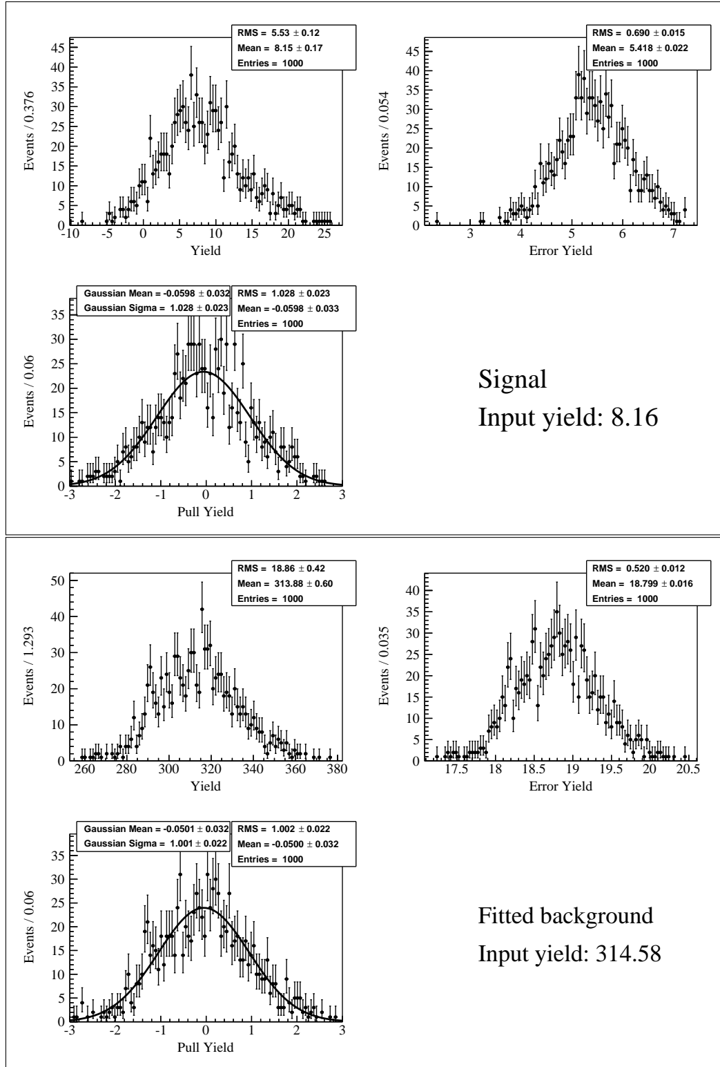
Figure 1.4: Toy study result for the optimal n_{\text{out}} selection of the cut-based procedure. Results show the electron channel of the nominal analysis.
