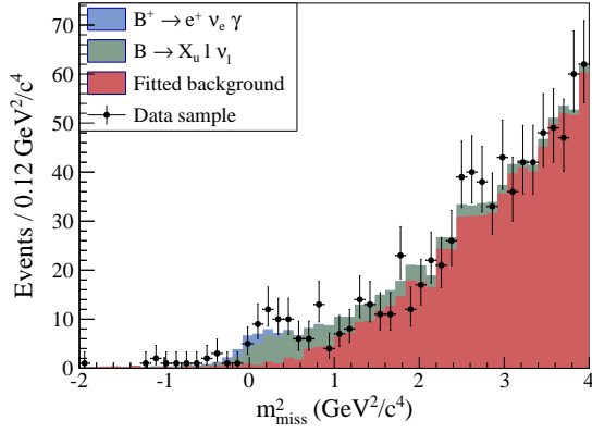
(c) Electron channel of the secondary analysis.
