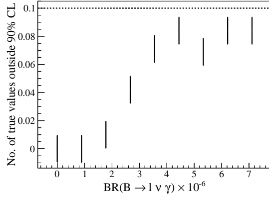
(c) Simultaneous fit to both channels.
