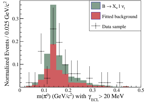
(b) Elec. channel: B \rightarrow X_u \ell^+ \nu_\ell enriched SB.
