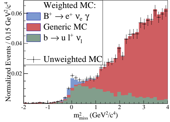
(b) Electron channel normalized.
