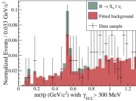
(c) Muon channel: fitted background SB.
