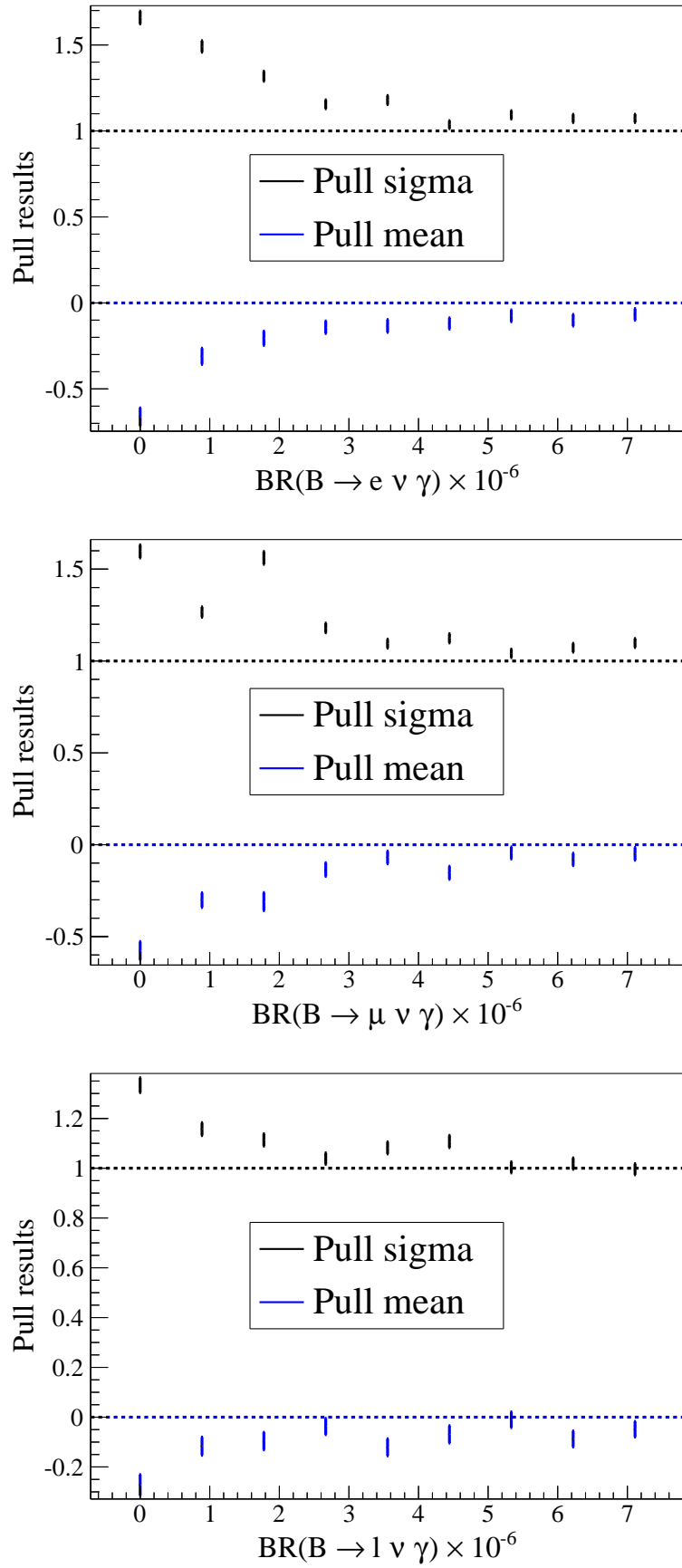
Figure 5.12: Linearity test for the nominal analysis showing the mean and width of the pull distribution for different signal branching fractions. The upper series shows the width and the mean of the pull distribution. Unbiased results are in agreement with the respective horizontal lines.
