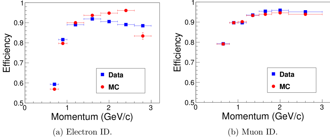
Figure 3.1: Efficiency of the Belle lepton ID determined in e^+e^- \rightarrow e^+e^-\ell^+\ell^- processes for a hard selection on the variables [17].
