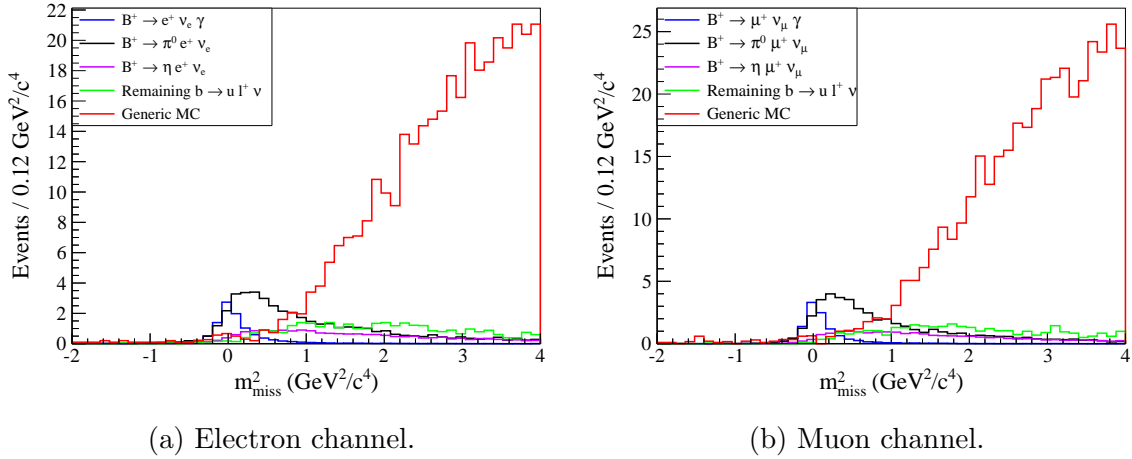
Figure 4.18: m_{\text{miss}}^2 distribution where the background sources of B^+ \rightarrow \pi^0\ell^+\nu_\ell and B^+ \rightarrow \eta\ell^+\nu_\ell dominate in the signal region below 1\text{GeV}^2/c^4 .
