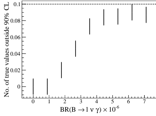
(c) Simultaneous fit to both channels.
