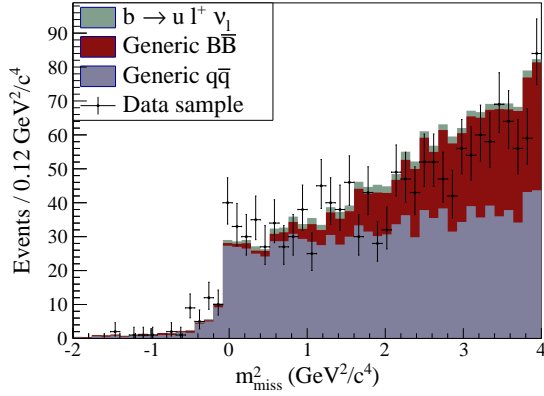
(c) Muon channel showing m_{\text{miss}}^2 computed using the beam energy without requiring high p_{\text{miss}} .
