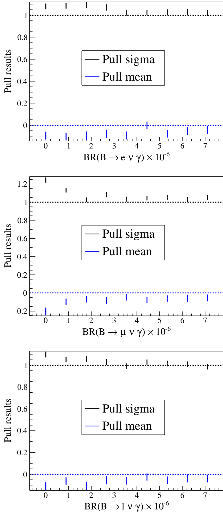
Figure 5.13: Linearity test for the secondary analysis. See description of Fig. 5.12.
