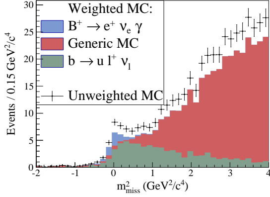
(a) Electron channel expected events.
