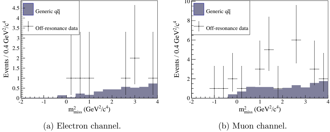
Figure 6.13: m_{\text{miss}}^2 distribution for q\bar{q} off-resonance data and generic q\bar{q} MC for the signal selection without the M_{\text{bc}} > 5.27 \text{ GeV}/c^2 requirement. The MC sample is scaled to the luminosity of the off-resonance data.
