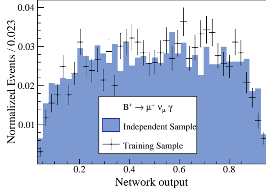
(b) Muon channel signal MC.
