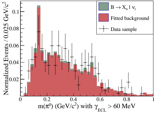
(c) Muon channel: fitted background SB.
