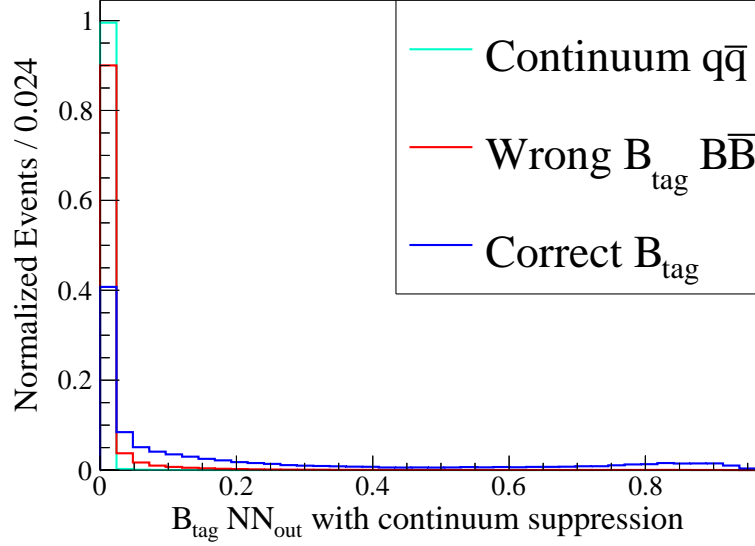
Figure 3.2: NN output of the full reconstruction for the B_{\text{tag}} meson with continuum suppression for Generic MC. The network output represents the Bayesian probability for the B meson to be correctly reconstructed. Correctly and wrongly reconstructed B_{\text{tag}} candidates are identified with the MC matching described in section 3.5.
