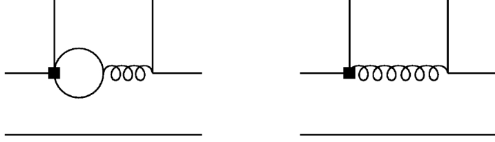
Figure 2.5: Higher-order Feynman diagrams which are a correction of \mathcal{O}(\alpha_s) to the leading order processes. Here, a gluon is emitted from the weak decay vertex of the bottom quark, either directly or with an intermediate penguin process. The gluon hadronizes into two quarks which form two separate mesons with the spectator quark of the B meson and the decay product of the bottom quark [1].
