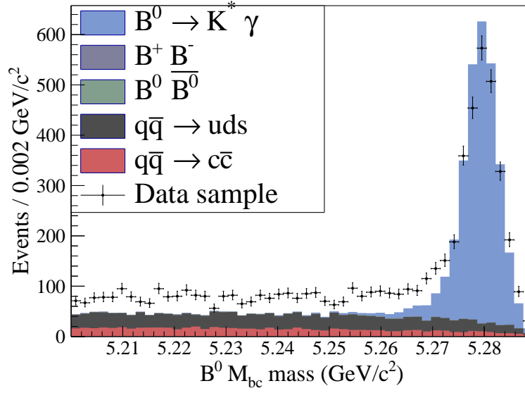
Figure 7.3: M_{bc} mass distribution of the B^0 after requiring the network output of the continuum suppression to be above 0.6.
