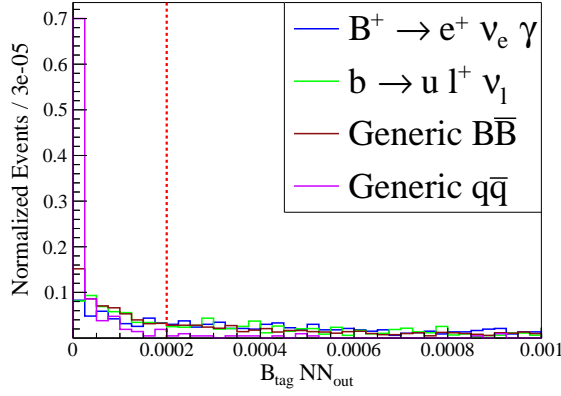
(c) Electron channel in the sub-range.
