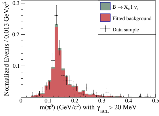
(a) Elec. channel: fitted background SB.
