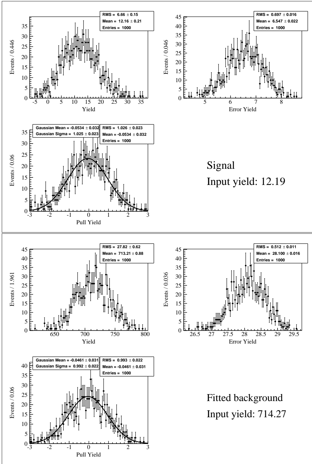
Figure 1.7: Toy study result for the optimal n_{\text{out}} selection of the cut-based procedure. Results show the muon channel of the secondary analysis.
