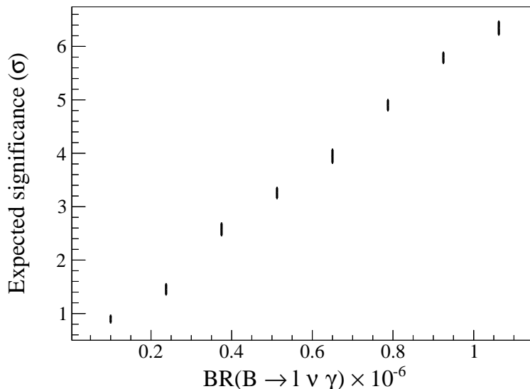
Figure 9.1: Expected significance of the B^+ \rightarrow \ell^+ \nu_\ell \gamma decay for the full Belle II data set of 50 \text{ ab}^{-1} .
