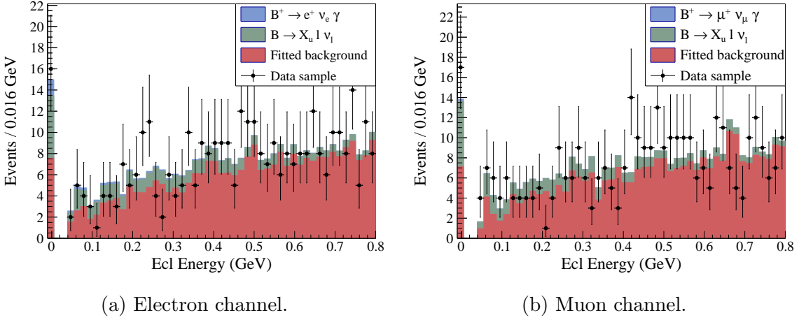
Figure 1.18: Extra energy in the ECL in the signal region.
