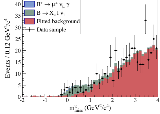
(b) Muon channel of the nominal analysis.
