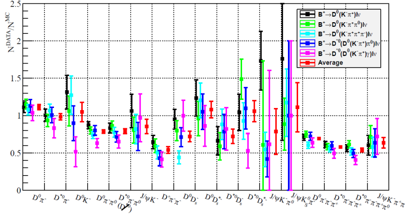
Figure 4.22: Data-MC tag-side efficiency difference plotted for all tag-side decay modes and several charmed signal-side decay channels [31].
