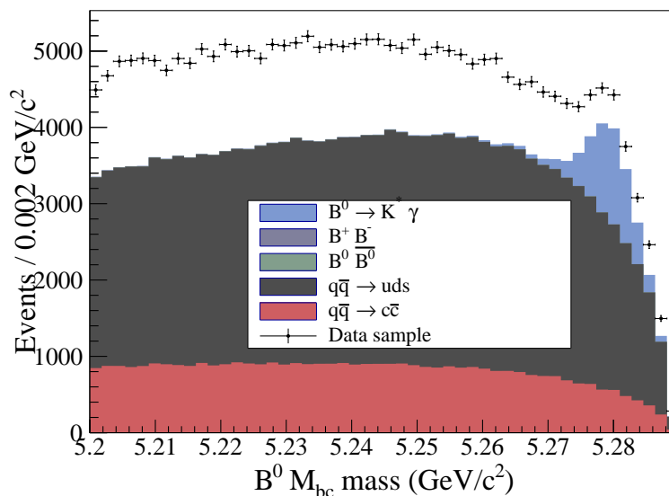
Figure 7.1: M_{bc} mass distribution of the B^0 meson after the K^*\gamma signal selection.
