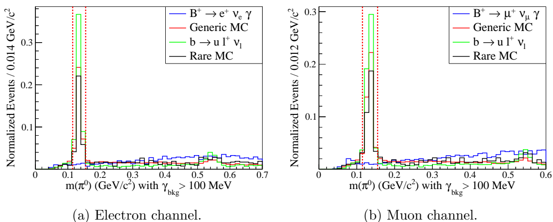
Figure 4.9: Invariant \pi^0 mass ( m_{\pi^0} ) reconstructed from the signal photon candidate and remaining photons in the ECL with energies above 100 \text{ MeV} , where a mass window of m_{\pi^0} \in (115, 155) \text{ MeV}/c^2 is selected.
