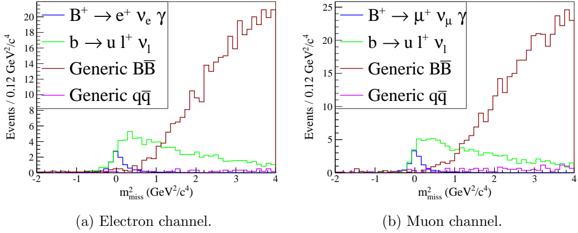
Figure 4.17: m_{\text{miss}}^2 distribution after all selections with the MC samples weighted to the luminosity of the data sample. The signal MC is shown with a branching fraction of 5 \times 10^{-6} .
