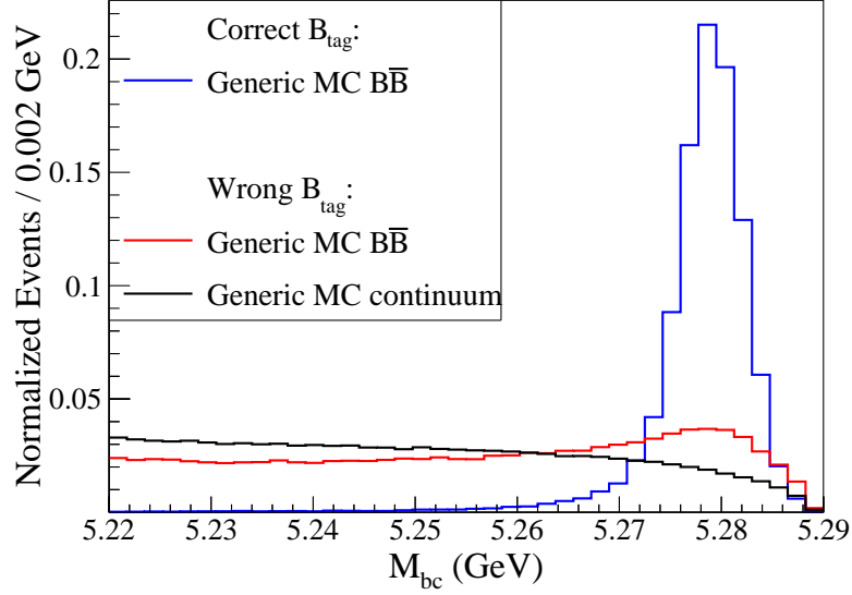
Figure 3.3: Beam-constrained B_{\text{tag}} mass for correctly and wrongly reconstructed B\bar{B} events for the generic MC. Correctly and wrongly reconstructed B_{\text{tag}} candidates are identified with the MC matching described in section 3.5.
