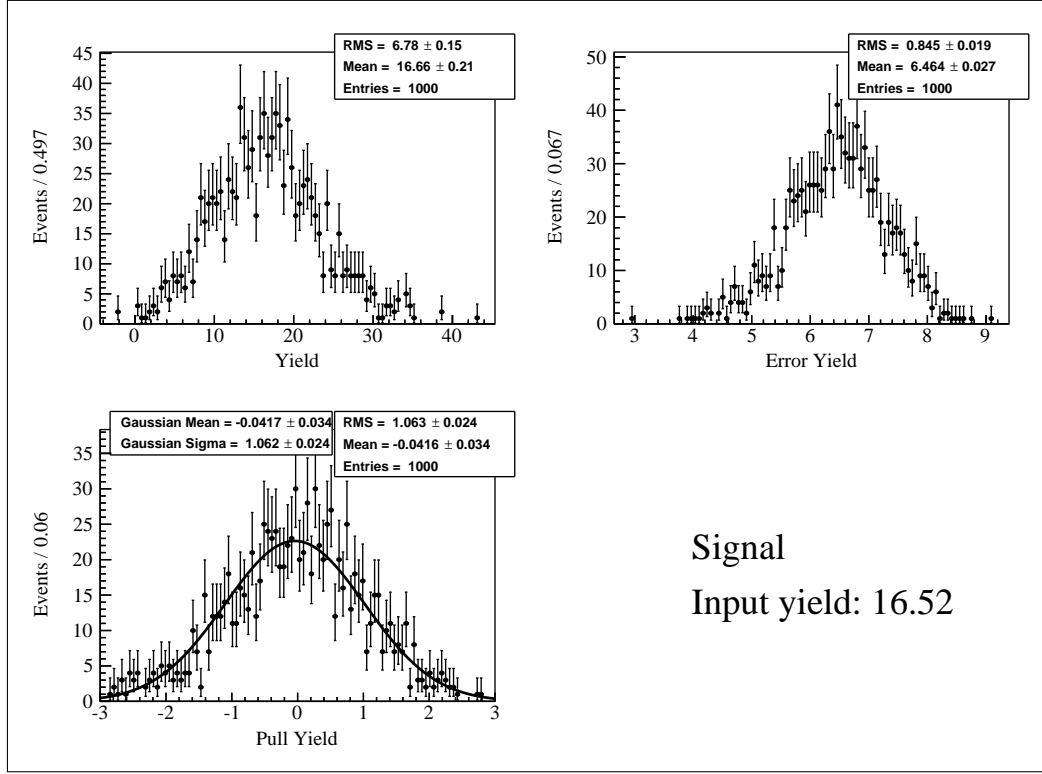
Figure 5.9: Toy study result for the joint signal yield of the simultaneous fit to both signal channels performed with a branching fraction of 5 \times 10^{-6} . The plot shows: the measured yields in the upper left panel, the statistical errors on the measured yields in the upper right panel, the pull distribution computed from the difference between measured and true yield divided by the statistical error in the lower left panel, and true yield used for toy generation in the lower right panel. A Gaussian is fitted to the pull distribution to determine its deviation from a unit Gaussian, where mean and standard deviation of the fit are displayed in the upper left corner of the panel. Each histogram has its number of entries, the mean, and the root mean square displayed in the upper right corner of the panel.
