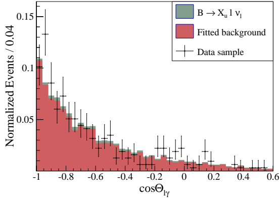
(c) Muon channel: fitted background SB.
