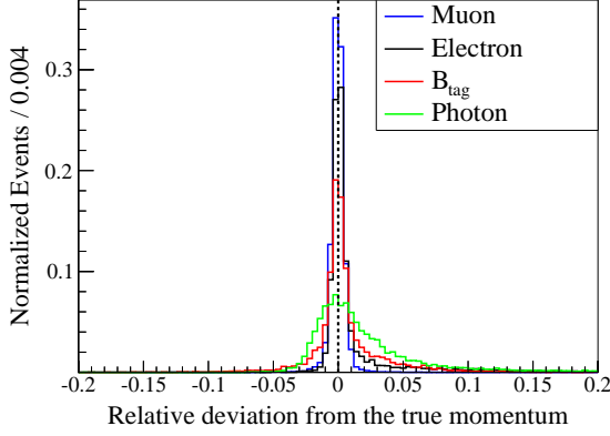
(a) Difference between reconstructed and true particle momenta for correctly identified signal and B_{\text{tag}} candidates, where the difference is divided by the true momentum.
