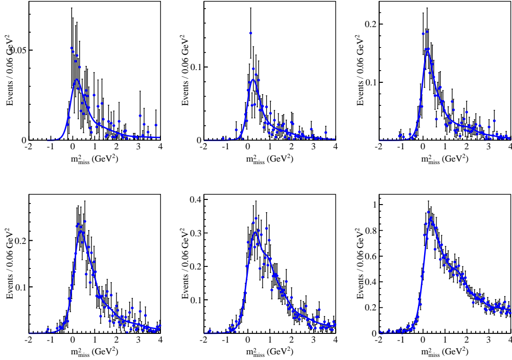
Figure 1.1: m_{\text{miss}}^2 distribution for the high luminosity samples of B^+ \rightarrow \pi^0 \ell^+ \nu_\ell and B^+ \rightarrow \eta \ell^+ \nu_\ell MC fitted in bins of the n_{\text{out}} . Results show the electron channel of the nominal analysis.
