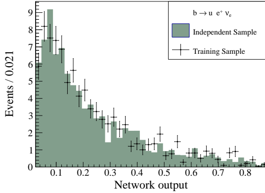
(c) Electron channel b \rightarrow u \ell^+ \nu_\ell MC.
