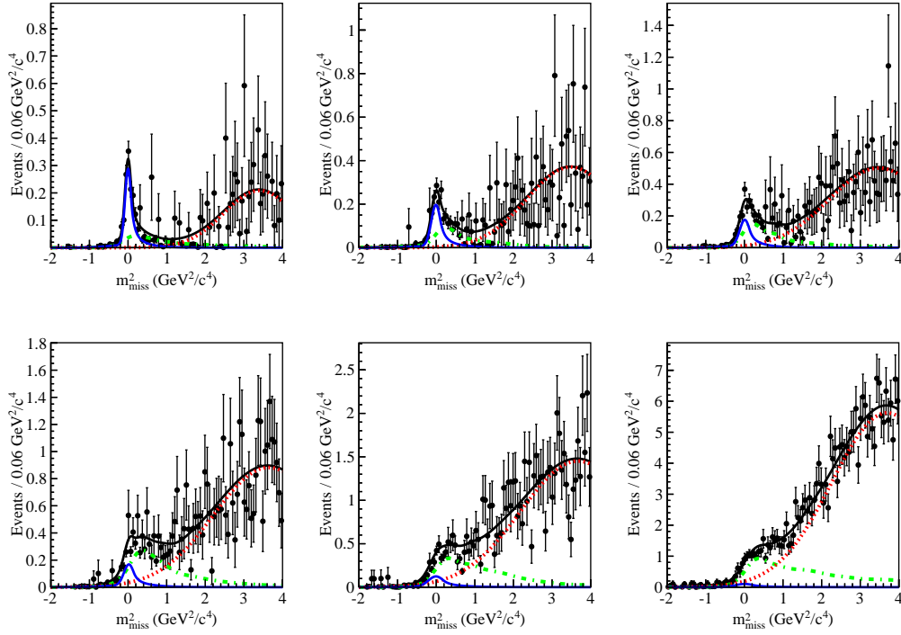
(a) Electron channel.
