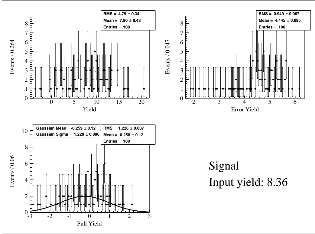
(a) Muon channel.
