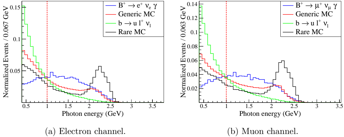
Figure 4.4: The initial distribution of the signal photon candidate energy in the B_{\text{sig}} rest frame. Thresholds are at 1 GeV for the nominal and 400 MeV for the secondary analysis. The peak in the rare MC originates from two-body decays of the form b \rightarrow s\gamma , where the strange-quark forms an excited kaon.
