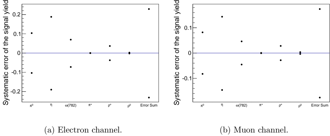
Figure 7.8: Systematic error obtained by varying the branching fraction of the B \rightarrow X_u \ell^+ \nu_\ell fit component.
