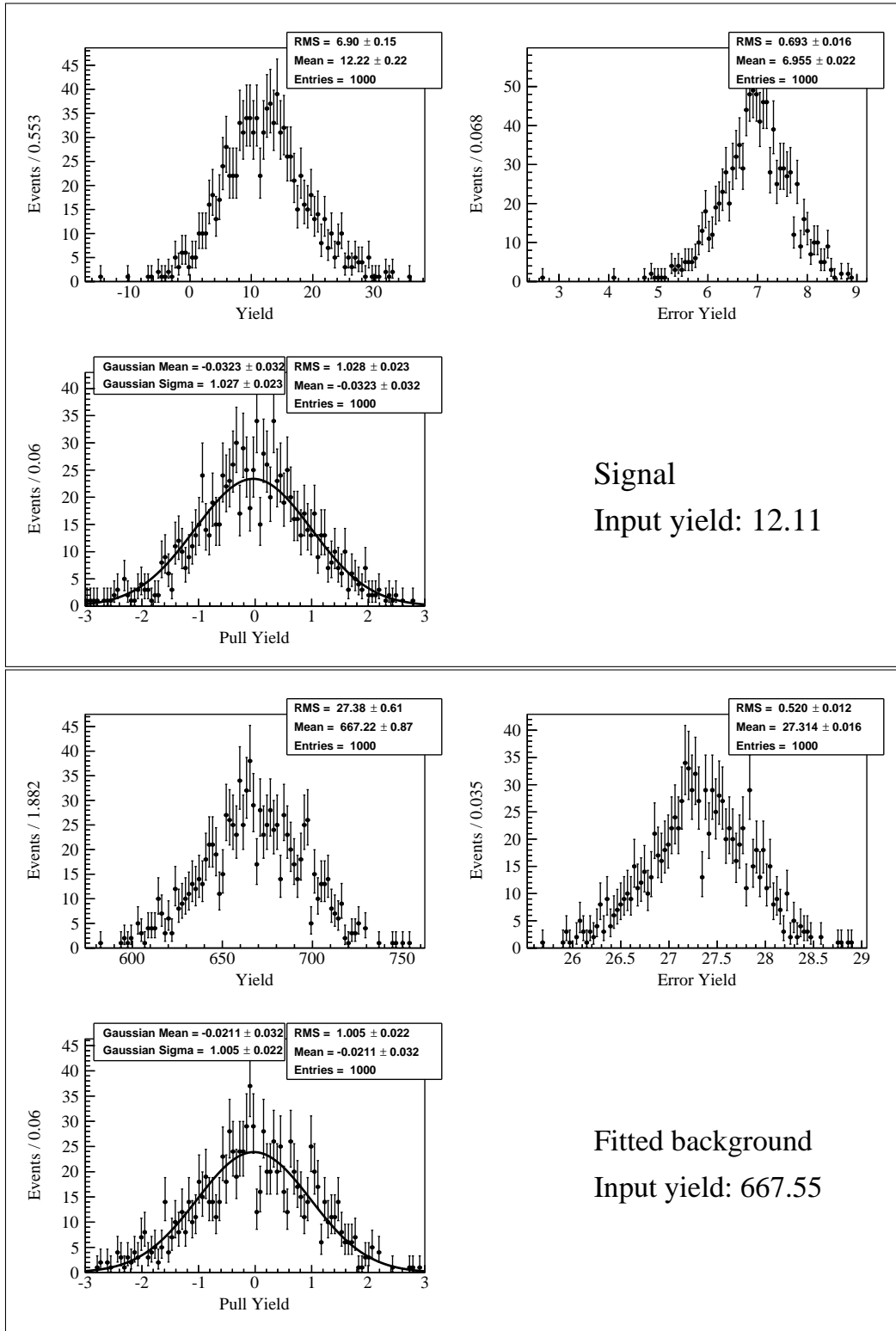
Figure 1.6: Toy study result for the optimal n_{\text{out}} selection of the cut-based procedure. Results show the electron channel of the secondary analysis.
