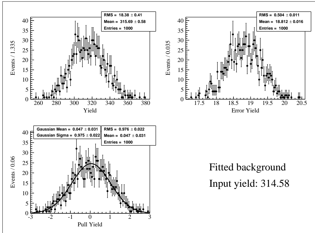
Figure 5.10: Toy study result for the electron channel with a signal branching fraction of 5 \times 10^{-6} . See Fig. 5.9 for a description of the plot.
