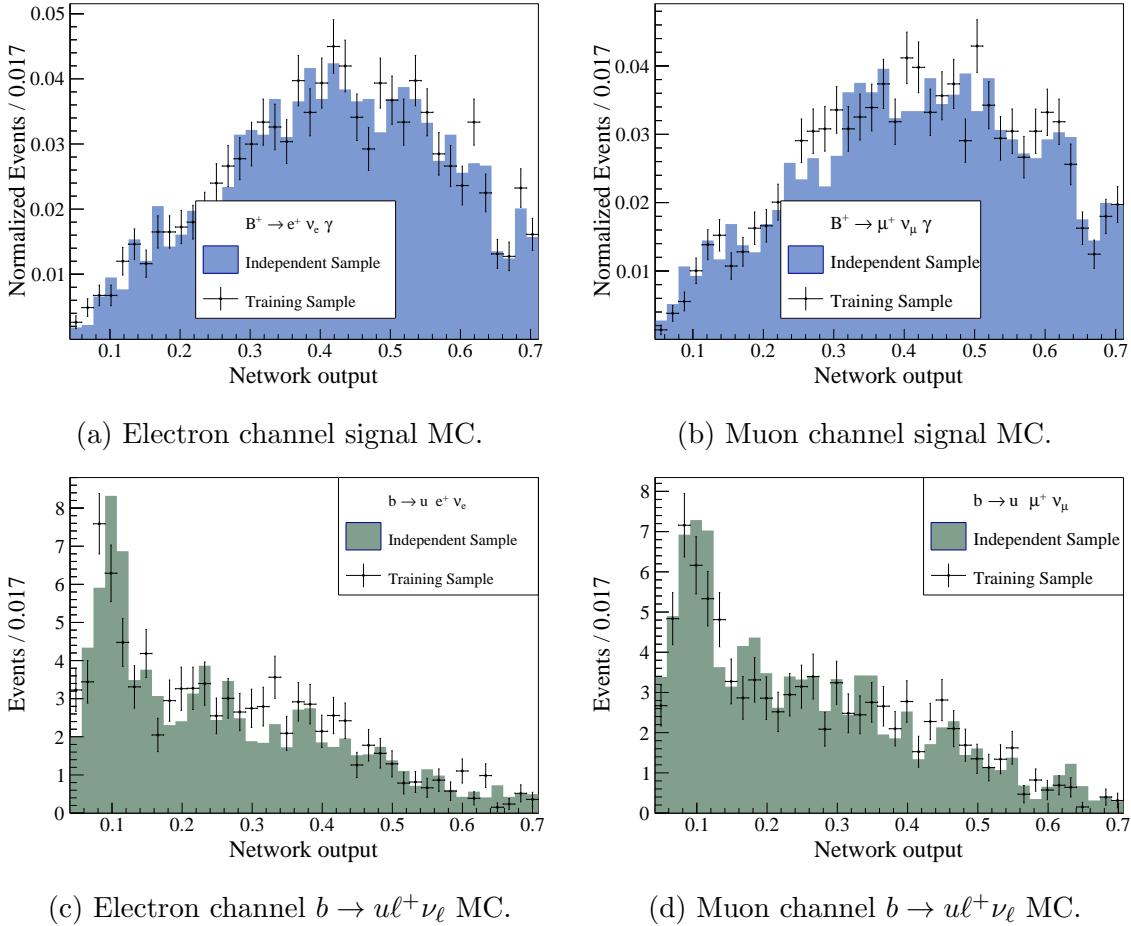
Figure 1.9: Secondary analysis n_{\text{out}} comparison between the training and independent sample for the training components of the signal MC and b \rightarrow u \ell^+ \nu_\ell MC.
