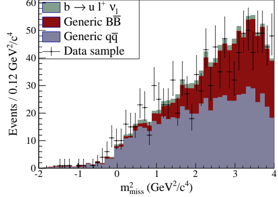
(b) Muon channel after requiring high p_{\text{miss}} .
