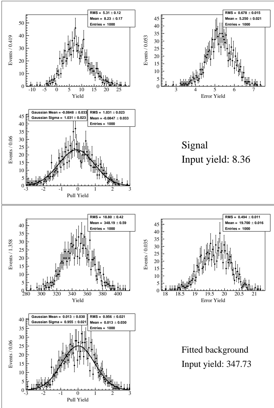
Figure 1.5: Toy study result for the optimal n_{\text{out}} selection of the cut-based procedure. Results show the muon channel of the nominal analysis.
