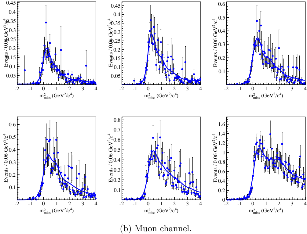
Figure 1.12: Combined B \rightarrow X_u \ell^+ \nu_\ell PDF of the m_{\text{miss}}^2 fit in six bins of n_{\text{out}} . The data points show well known decays of the b \rightarrow u \ell^+ \nu_\ell MC together with the high luminosity samples of B^+ \rightarrow \pi^0 \ell^+ \nu_\ell and B^+ \rightarrow \eta \ell^+ \nu_\ell . The differing luminosities lead to non-uniform error bars.
