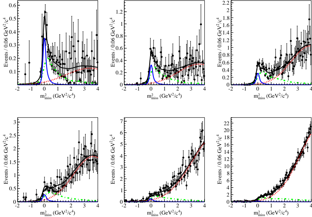
(b) Muon channel.
