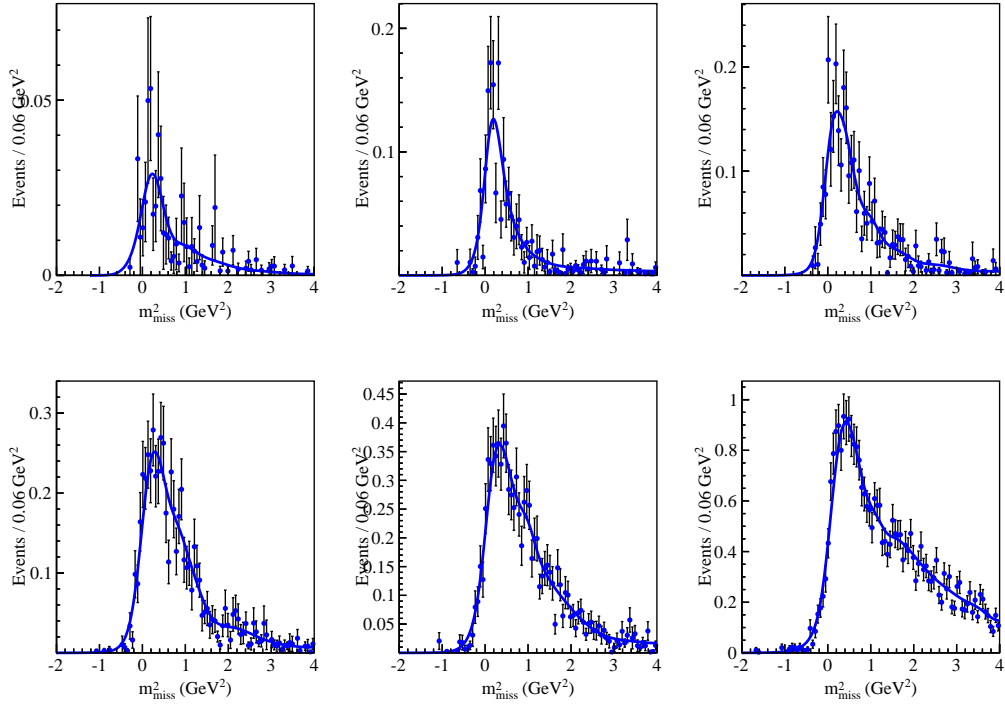
Figure 1.2: m_{\text{miss}}^2 distribution for the high luminosity samples of B^+ \rightarrow \pi^0 \ell^+ \nu_\ell and B^+ \rightarrow \eta \ell^+ \nu_\ell MC fitted in bins of the n_{\text{out}} . Results show the muon channel of the nominal analysis.
