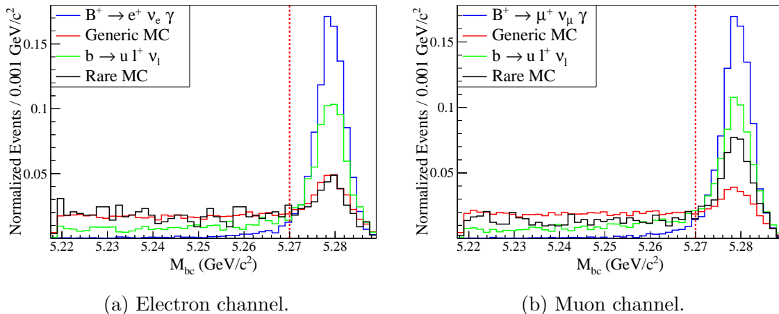
Figure 4.10: Beam-constrained B_{\text{tag}} mass M_{\text{bc}} which is required to be above 5.27 \text{ GeV}/c^2 .
