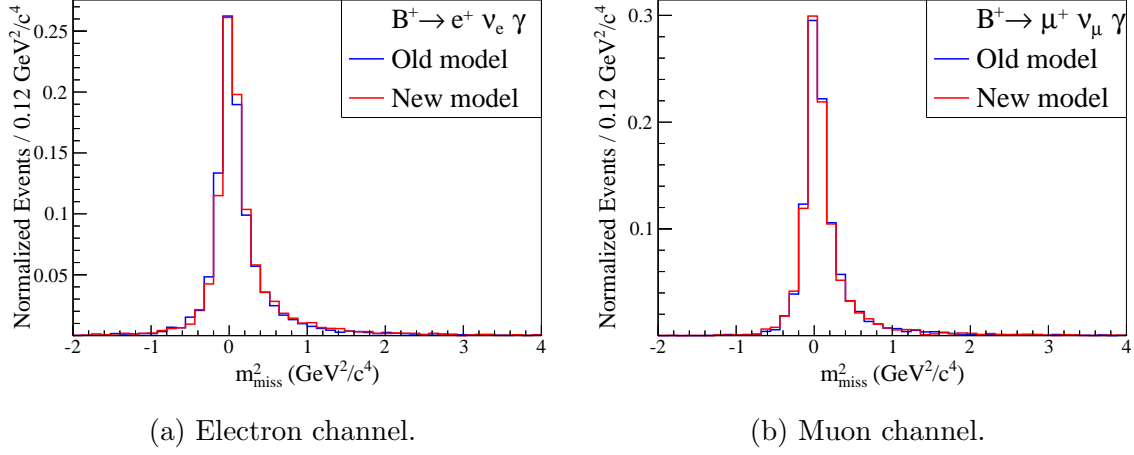
Figure 7.9: m^2_{\text{miss}} shape comparison for the LO and NLO calculations.
