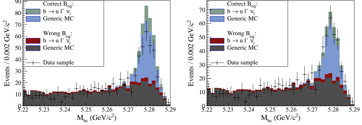
(a) Muon channel without corrective weights. (b) Muon channel with corrective weights.
