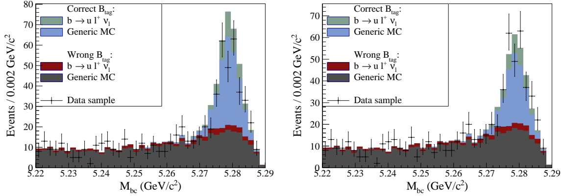
(c) Electron channel without corrective weights. (d) Electron channel with corrective weights.
