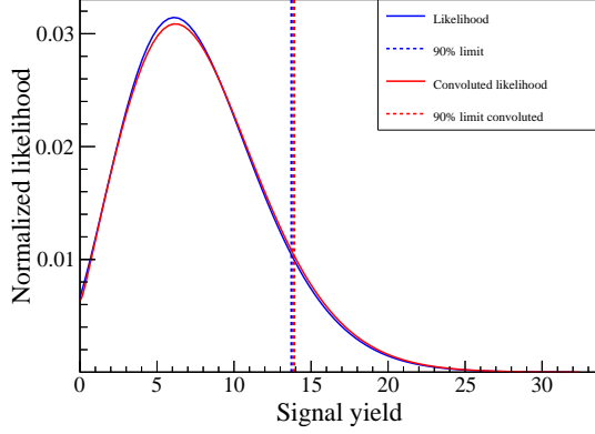
(a) Electron channel of the nominal analysis.
