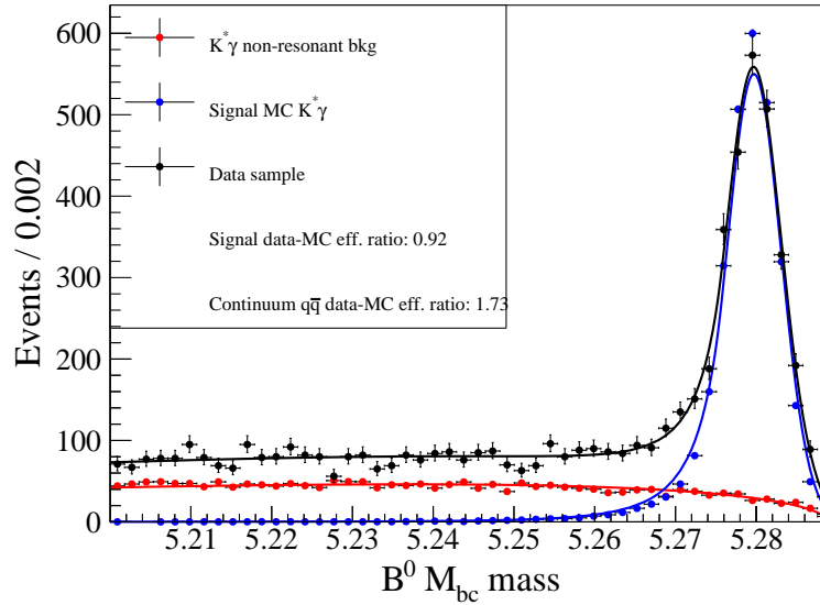
Figure 7.4: Signal and background shape comparison between data and MC for the M_{bc} mass. The PDFs are fitted on data and plotted on the MC samples. The background shape agrees well, and a broader signal peak is observed on data than on MC.
