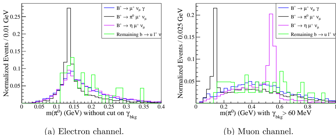
Figure 4.19: \pi^0 mass computed from the signal photon candidate and a remaining photon in the ECL. The masses are plotted for two different energy thresholds on the ECL photons where the artificial peak around the nominal \pi^0 mass disappears for the higher threshold.
