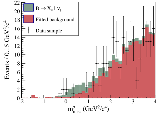
(c) Muon channel in the sideband satisfying M_{bc} > 5.27 \text{ GeV}/c^2 and n_{\text{out}} < 0.25 .
