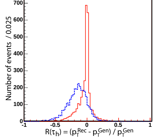
FIG. 2: Comparison of the true hadronic tau transverse energy (as obtained from MC) and the reconstructed tau candidate energy using CDF II detector simulation for Z \rightarrow \tau\tau events. The dashed line corresponds to using only calorimeter energy, while the solid line corresponds to the combination of track and \pi^0 energies with appropriate corrections.
