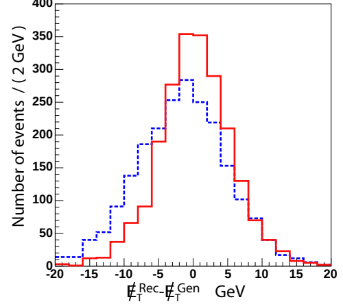
FIG. 7: Comparison of the reconstructed missing transverse energy with the true value obtained at the generator level in the pythia MC Z \rightarrow \tau_e \tau_h events. Dashed line shows the \vec{E}_T^{Rec} - \vec{E}_T^{Gen} distribution prior to the correction procedure, and the solid line shows the same distribution when all corrections have been applied.
