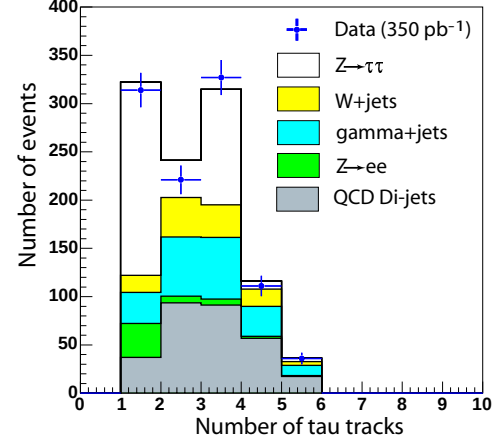
FIG. 14: Distribution of the prong multiplicity of hadronic tau candidates with the OS and N_{trk} = 1, 3 requirements dropped. Data (points) are compared to the sum of background and signal contributions. The Z \rightarrow \tau\tau and background predictions are normalized to the number of events extracted from the fit (with all cuts applied).
