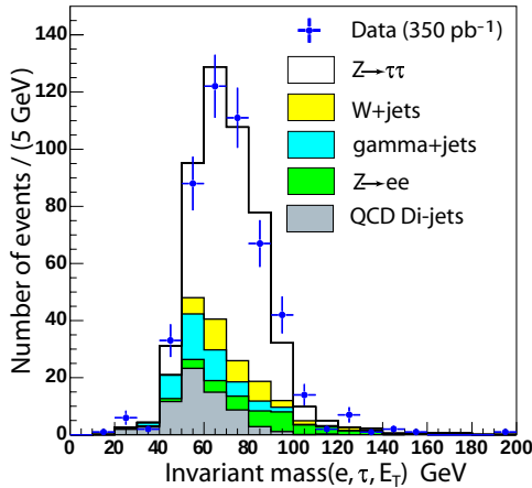
FIG. 13: Distribution of the invariant mass of e-\tau system for opposite sign events in data (points) compared to the sum of background and signal contributions. The Z \rightarrow \tau\tau and background predictions are normalized to the number of events extracted from the fit.
