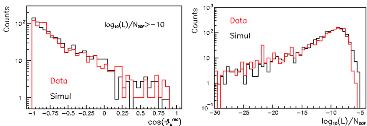
Figure 5. Angular distribution of reconstructed muon tracks in terms of the Zenith angle cosine and their likelihood spectrum compared with Monte Carlo simulations.
