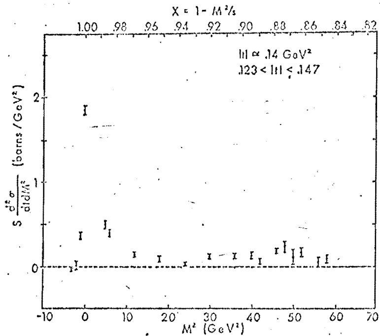
Fig. 11. Doubly differential cross section versus M^2 for |t| = 0.14 \text{ GeV}^2 .
