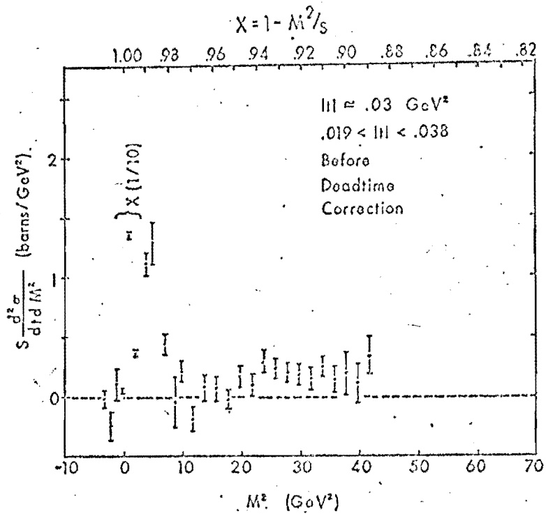
Fig. 7. Doubly differential cross section versus M^2 for |t| \approx 0.03 \text{ GeV}^2 before deadtime correction.
