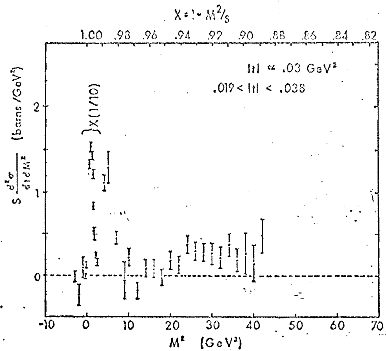
Fig. 8. Doubly differential cross section versus M^2 for |t| \approx 0.03 \text{ GeV}^2 .
