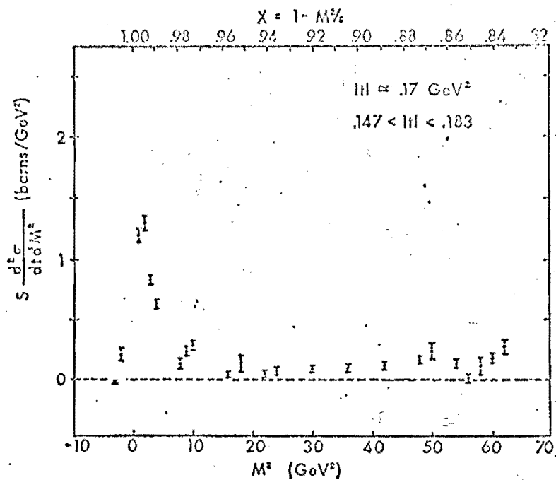
Fig. 12. Doubly differential cross section versus M^2 for |t| = 0.17 \text{ GeV}^2 .
