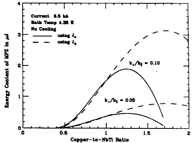
Fig. 6. Energy content of three-dimensional MPZ using J_c or J_q with interfilament copper neglected.
