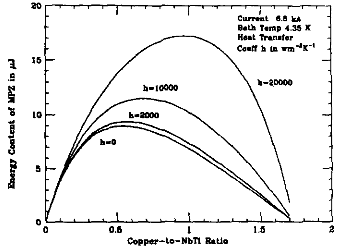
Fig. 3. Energy content of MPZ with surface cooling.
