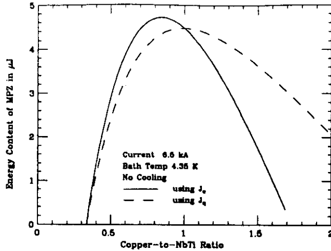
Fig. 4. Energy content of one-dimensional MPZ using J_c or J_q with interfilament copper neglected.
