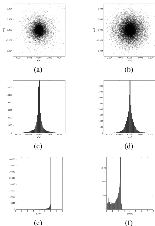
Figure 3: Beam spots (a, b), histograms of current transverse distribution (c, d), energy spectra of the beam (e, f) at the bremsstrahlung target for the energies of 6 MeV (left column) and 2.5 MeV (right column).
