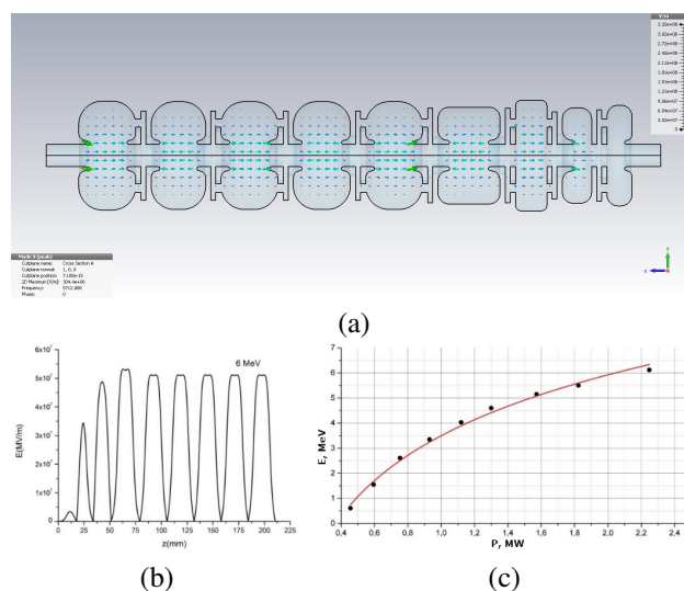
Figure 1: (a) Geometry of the accelerating structure with operating mode electric field distribution. (b) Distribution of the electric field along the axis. (c) Relationship between the output beam energy and the pulsed RF power loss in cavities walls.
