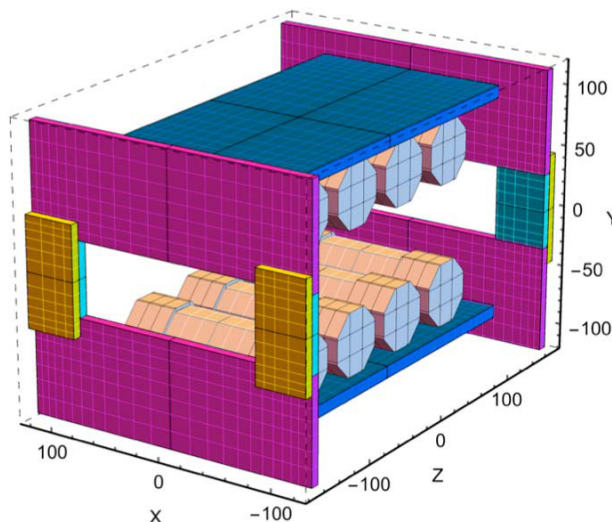
Figure 1: Outline of the permanent steering magnet.
