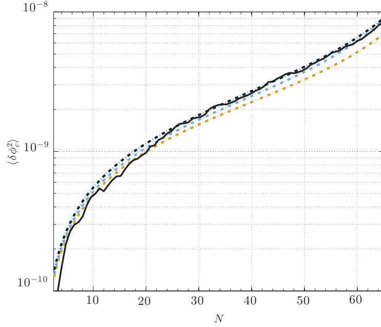
Figure 7.5 Total integrated power in, or variance of, the classical long-wavelength fluctuations, \langle \delta\phi_c^2 \rangle , in units of M_{\text{Pl}}^2 . The full (black) line is the numerical result, while the dashed light- and dark-blue dashed lines correspond to different analytic approximations to the integral in equation (7.43), see footnote 8 for details. The yellow dashed line corresponds to a noise variance of H^4(t)/(4\pi^2) , i.e. the naive approximation obtained by slow-roll corrected H(t) to account for the fact that the bath evolves in a slow-rolling background [47]. This graph was obtained by simulating 100 realizations, and, assuming a Gaussian underlying PDF, the mean and variances were inferred by maximizing the likelihood of the \mu - \sigma space. Simulations were performed using m = 6 \times 10^{-6} M_{\text{Pl}} , N_{\text{tot}} = 80 .
