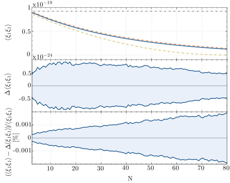
Figure 7.4 Power spectrum of the noise correlator at step 3 of the recursive method, \langle \xi_1 \xi_1 \rangle . Top panel: Average power spectrum, \langle \xi_1 \xi_1 \rangle , in units of M_{\text{Pl}}^4 . The full (blue) line is the corrected power spectrum obtained numerically at step 3, while the red line is the analytic computation. The grey dashed line is the variance obtained at the previous step of the recursion, H_0^4/(4\pi^2) , and the yellow dashed line is H^4(t)/(4\pi^2) , i.e. the naive correction to the noise to account for the fact that inflation happens in quasi-de Sitter space by simply making the Hubble radius a time-dependent quantity. Middle panel: 1\sigma deviation from the mean trajectory, i.e. standard deviation of maximum likelihood, again in units of M_{\text{Pl}}^4 . Bottom panel: Percentage error at 1\sigma . These graphs were obtained by simulating 100 realizations, and, assuming a Gaussian underlying PDF, the mean and variances were inferred by maximizing the likelihood of the \mu - \sigma space. Simulations were performed using m = 6 \times 10^{-6} M_{\text{Pl}} , N_{\text{tot}} = 80 .
