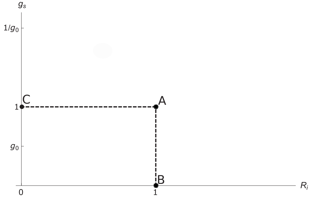
Figure 4.1 The Type IIB moduli space with the self-dual point denoted by A . The point B is for all R_i = 1 and the point C is for g_s = 1 . Our duality mappings are defined for the point A . Going away from the point A in any direction in the moduli space will imply switching on non-trivial values for the axio-dilaton.
