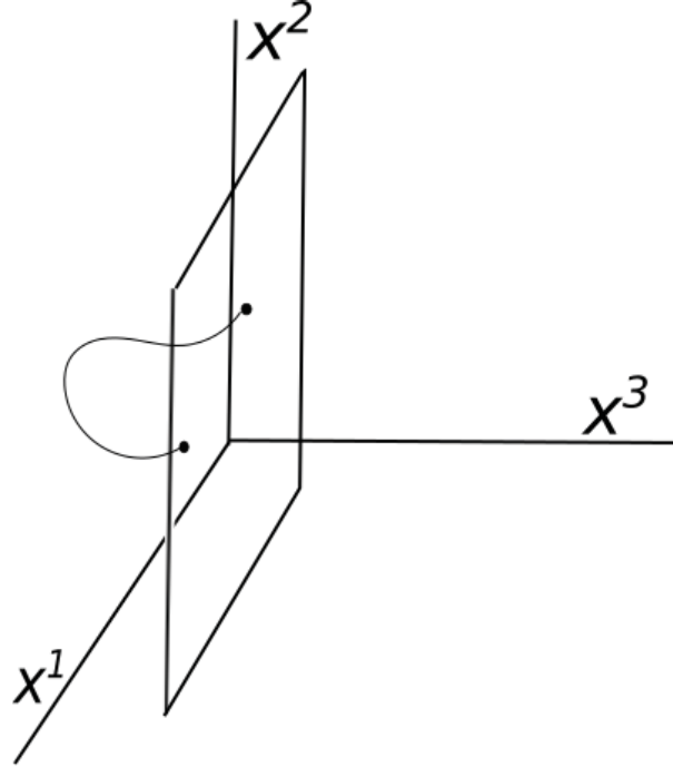
Figure 2.2 A D2 brane in 3+1 dimensions (the time-direction is suppressed)
