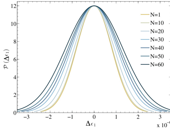
Figure 7.2 The reconstructed (un-normalized) probability density function of the slow-roll parameter \epsilon_1 (the subscript 1 denotes first slow-roll parameter) for a few fixed e -folds during the last 60 e -folds of inflation. These values were inferred from 250 realizations, with m = 6 \times 10^{-6} M_{\text{Pl}} , N_{\text{tot}} = 60 .
