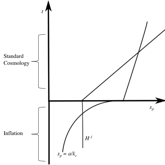
Figure 1.1 The evolution of the physical length of a fixed comoving length scale and the Hubble length scale during Inflation.
