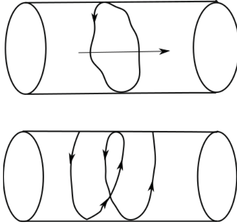
Figure 2.3 Momentum and Winding Modes (top and bottom respectively).
