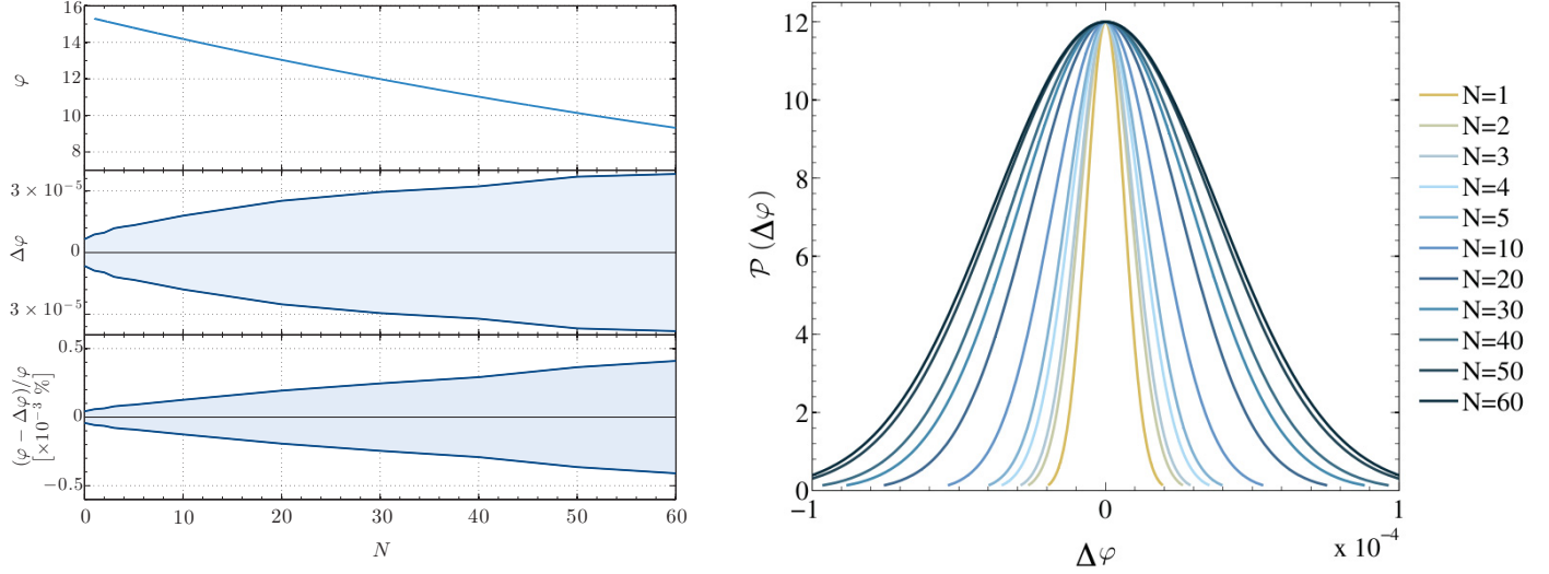
Figure 7.1 Left panel: Top: mean trajectory of the coarse grained inflaton \varphi . Note that the large discrepancy of \varphi(N = 60) compared to the standard slow-roll value is simply due to the fact that at this level in the recursion, we solved the EoM for \varphi keeping H = H_0 , a constant. This means that by the end of inflation, we can expect corrections to our coarse-grained solution as large as \epsilon_1 N . Middle: 1\sigma deviation from the mean trajectory, i.e. standard deviation of maximum likelihood. Bottom: percentage error at 1\sigma . Right panel: The reconstructed (un-normalized) PDF of the random variable \varphi(N) - \langle\varphi(N)\rangle for a few fixed e -folds during inflation, and assuming inflation lasted 60 e -folds. These values were inferred from 250 realizations, with m = 6 \times 10^{-6} M_{\text{Pl}} , N_{\text{tot}} = 60 , and \phi_c(0) = \sqrt{2(2N_{\text{tot}} - 1)} . All fields shown are in units of M_{\text{Pl}} .
