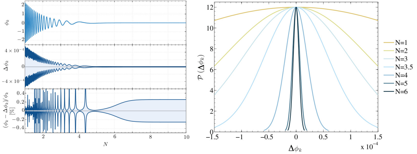
Figure 7.3 Left panel: Top: mean trajectory of the real part of the linearized mode function \phi_k with k = 1.26 \times 10^{-2} M_{\text{Pl}} , freezing at N \approx 5.5 . Middle: 1\text{-}\sigma deviation from the mean trajectory, i.e. standard deviation of maximum likelihood. Bottom: percentage error at 1\sigma . Right: The reconstructed (unnormalized) PDF of the random variable \phi_k(N) - \langle \phi_k(N) \rangle for a few fixed e -folds during the last 60 e -folds of inflation. These values were inferred from 250 realizations, with m = 6 \times 10^{-6} M_{\text{Pl}} , N_{\text{tot}} = 60 . Fields are shown in units of M_{\text{Pl}} .
