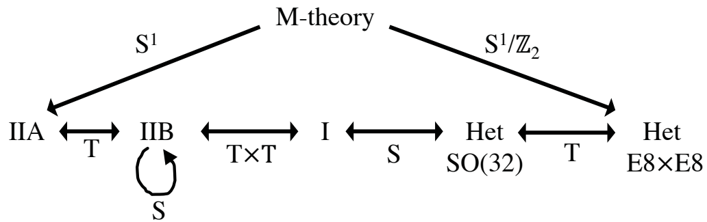
Figure 2.1 The Dualities of String Theory
