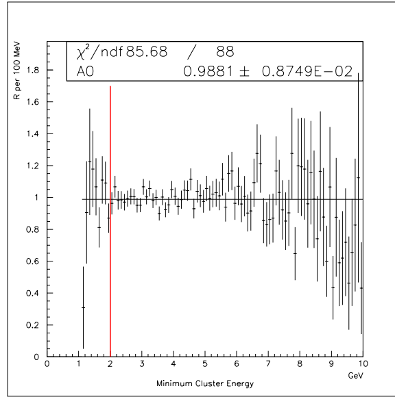
Figure 6.19: Double ratio as a function of the minimum cluster energy.
