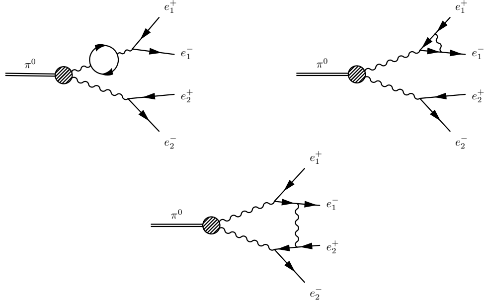
Figure 2.6: Examples of the three types of 1-loop contributions to the double Dalitz decay: vacuum polarization, vertex correction, and happy face.
