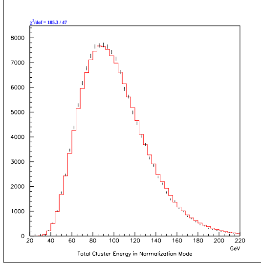
Figure 6.5: Comparison between normalization mode data (points with error bars) and normalization mode Monte Carlo (histogram) for the distribution of total cluster energy. All other cuts have been applied.
