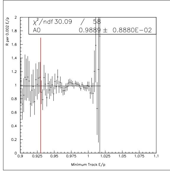
Figure 6.23: Double ratio as a function of the minimum E/p .
