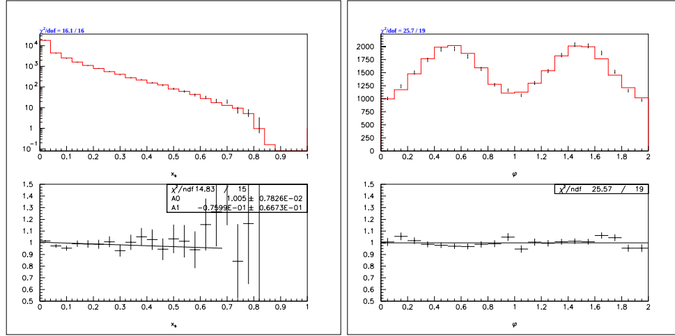
Figure 7.9: Comparison of the distributions of x_b and \phi between the data (points) and 5 MC samples (black histogram). The ratios are data over MC.
