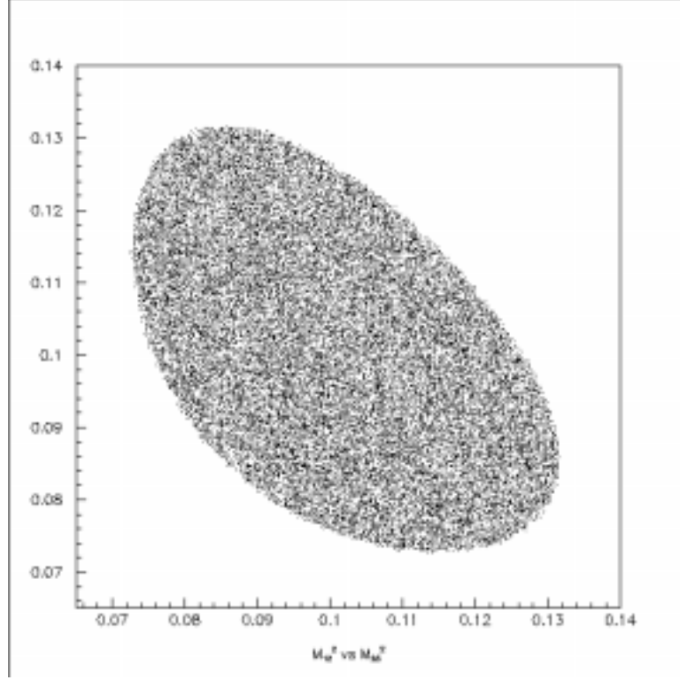
Figure 4.2: Dalitz plot for K_L \rightarrow \pi^0 \pi^0 \pi^0 decays at generation.
