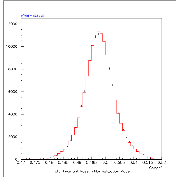
Figure 6.13: Comparison between normalization mode data (points with error bars) and normalization mode Monte Carlo (histogram) for the distribution of total invariant mass. All other cuts have been applied.
