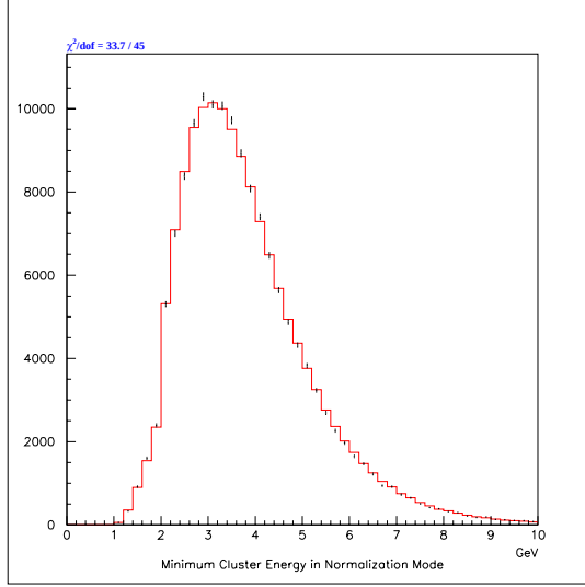
Figure 6.4: Comparison between normalization mode data (points with error bars) and normalization mode Monte Carlo (histogram) for the distribution of minimum cluster energies. All other cuts have been applied.
