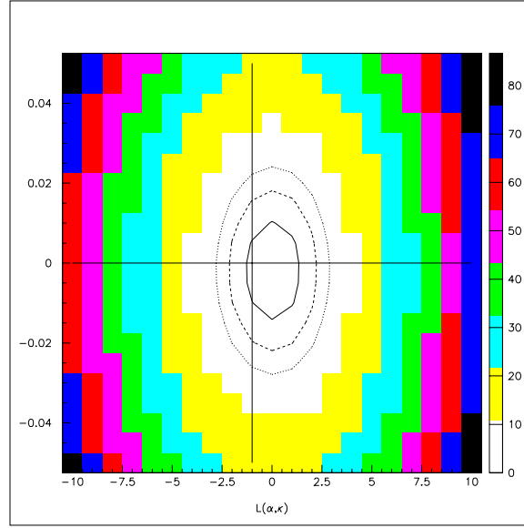
Figure 7.2: Likelihood function in two variables at the minimum of the third variable, using a Monte Carlo sample equivalent to one dataset. The two free variables are \alpha-\kappa . The contours indicate the 1, 2, and 3\sigma levels appropriate for two free parameters. The generated point (0,0) is given by the crossing of the two lines.
