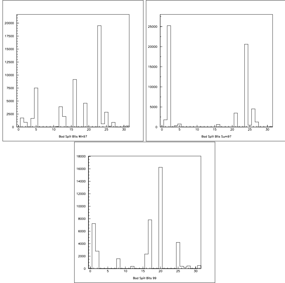
Figure 6.1: Distribution of bad spill bits in the 4e8c dataset for each of the three run periods.
