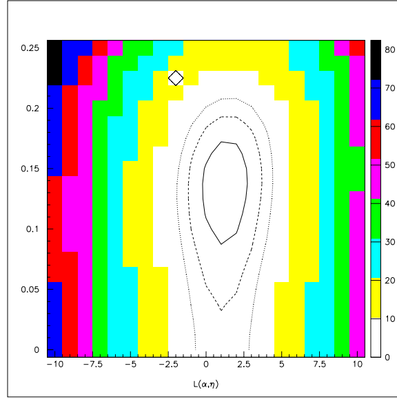
Figure 7.11: Likelihood function in two variables at the minimum of the third variable, using the complete KTeV dataset. The two free variables are \alpha – \eta . The contours indicate the 1, 2, and 3 \sigma levels appropriate for two free parameters.
