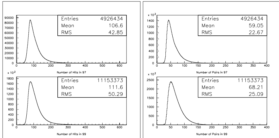
Figure 5.2: Distributions of the number of hits per event (left) and the number of pairs per event (right), in both 97 and 99 2e-nclus 4-track data.
