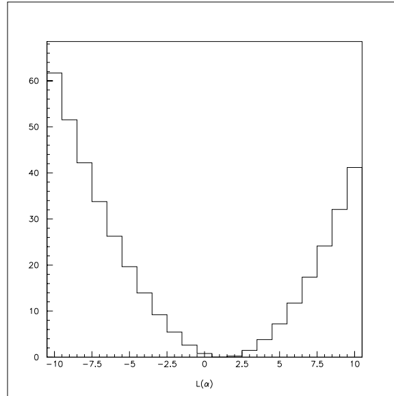
Figure 7.13: Likelihood function in one variable at the minimum of the other two variables, using the complete KTeV dataset. The free variable is \alpha .
