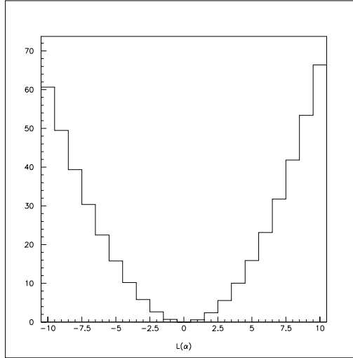
Figure 7.5: Likelihood function in one variable at the minimum of the other two variables, using a Monte Carlo sample equivalent to one dataset. The free variable is \alpha and the generated point is \alpha = 0 .
