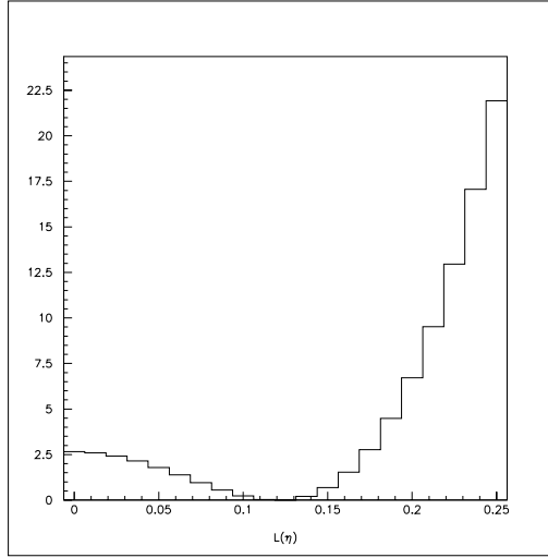
Figure 7.7: Likelihood function in one variable at the minimum of the other two variables, using a Monte Carlo sample equivalent to one dataset. The free variable is \eta and the generated point is \eta = 0 .
