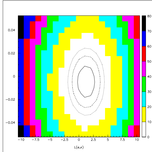
Figure 7.10: Likelihood function in two variables at the minimum of the third variable, using the complete KTeV dataset. The two free variables are \alpha - \kappa . The contours indicate the 1, 2, and 3 \sigma levels appropriate for two free parameters.
