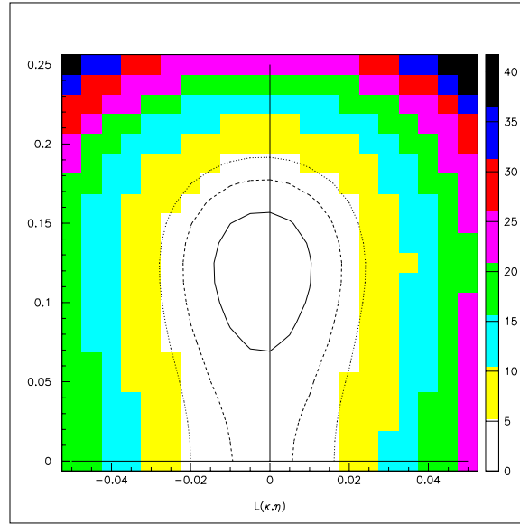
Figure 7.4: Likelihood function in two variables at the minimum of the third variable, using a Monte Carlo sample equivalent to one dataset. The two free variables are \kappa - \eta . The contours indicate the 1, 2, and 3 \sigma levels appropriate for two free parameters. The generated point (0,0) is given by the crossing of the two lines.
