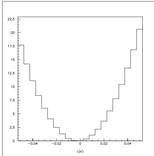
Figure 7.6: Likelihood function in one variable at the minimum of the other two variables, using a Monte Carlo sample equivalent to one dataset. The free variable is \kappa and the generated point is \kappa = 0 .
