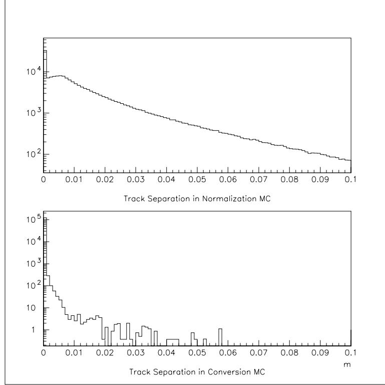
Figure 6.17: Distribution of minimum track separation at DC1 on a logarithmic scale. The top plot contains normalization mode Monte Carlo events. The bottom plot contains single conversion Monte Carlo events.
