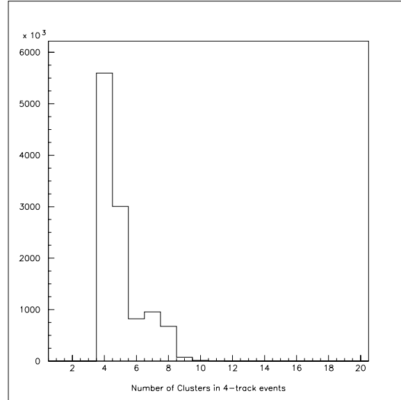
Figure 5.15: Distribution of the number of clusters in 4TRACK events.
