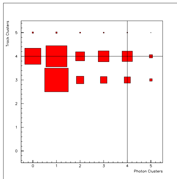
Figure 5.10: Two dimensional distribution of the number of clusters identified as photons versus the number of clusters associated with tracks.
