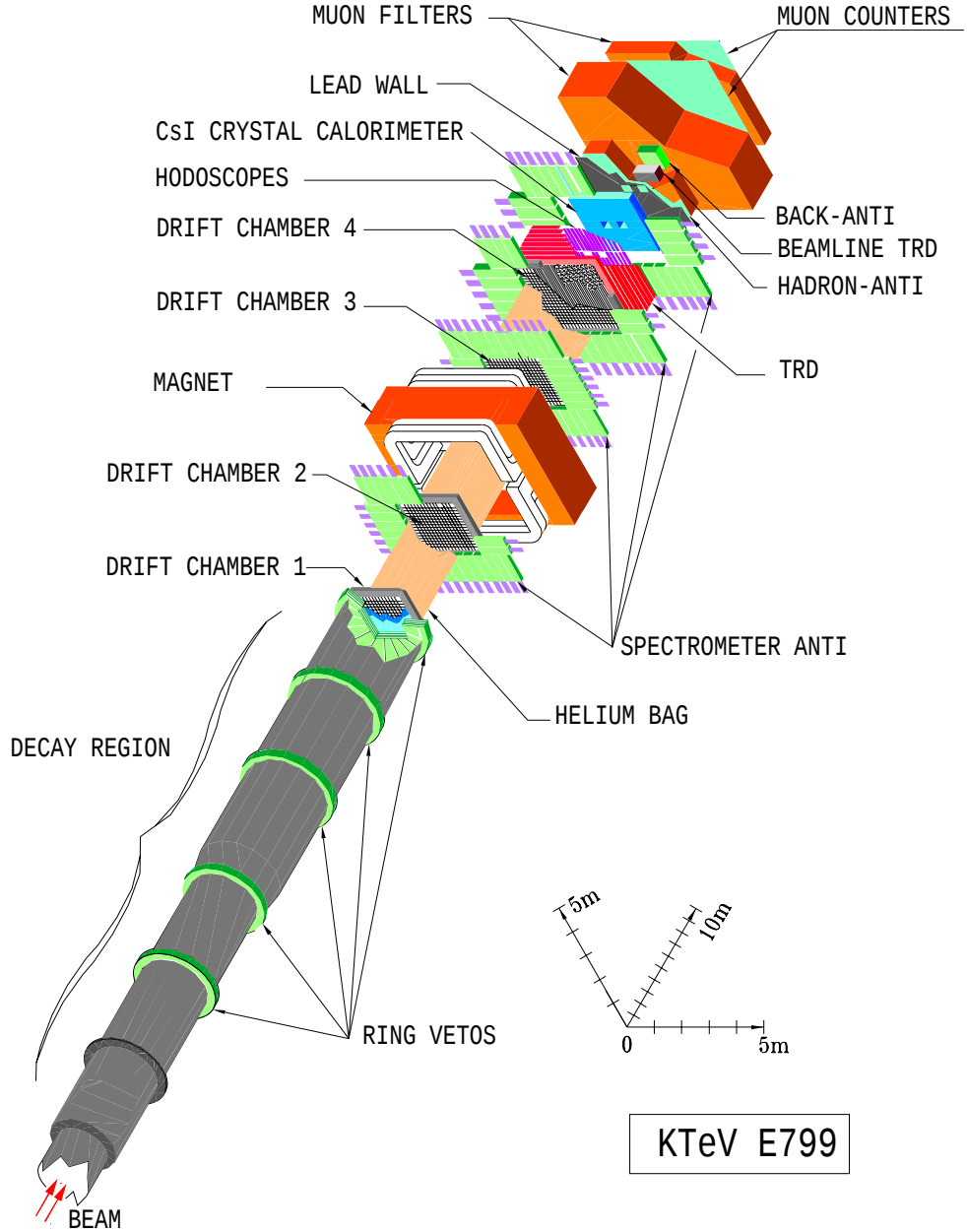
Figure 3.3: The KTeV Detector. The axis parallel to the beam defines \hat{z} and is shown elongated by a factor of 2 \times 1 relative to the transverse directions.
