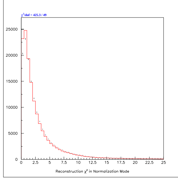
Figure 6.15: Comparison between normalization mode data (points with error bars) and normalization mode Monte Carlo (histogram) in the reconstruction \chi^2 variable.
