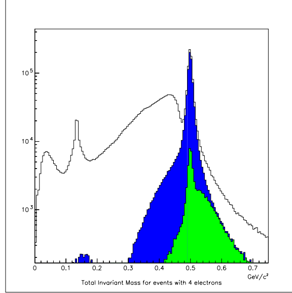
Figure 5.12: Distribution of the total invariant mass in events which have four tracks with E/p > 0.9 . The events in the blue histogram have, in addition to the electrons, four photons (4e8c), while those in green have five photons (4e9c).
