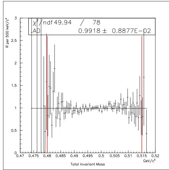
Figure 6.28: Double ratio as a function of the total mass.
