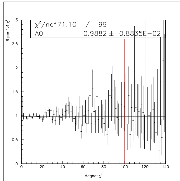
Figure 6.26: Double ratio as a function of the magnet \chi^2 .
