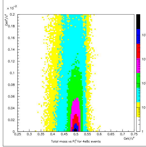
Figure 5.14: Two dimensional distribution of the total invariant mass versus the transverse momentum squared for events with four electrons and four photons.
