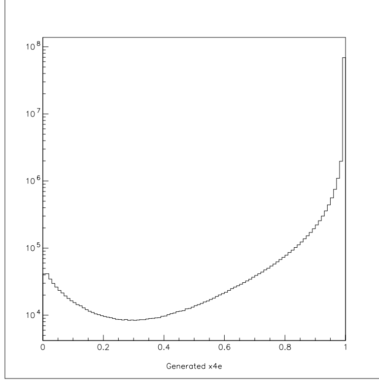
Figure 4.3: Distribution of generated x_{4e} values from both \pi^0 \rightarrow e^+e^-e^+e^- and \pi^0 \rightarrow e^+e^-e^+e^-\gamma events.
