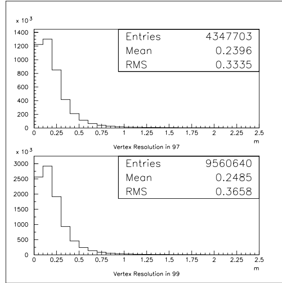
Figure 5.8: Vertex z resolution.
