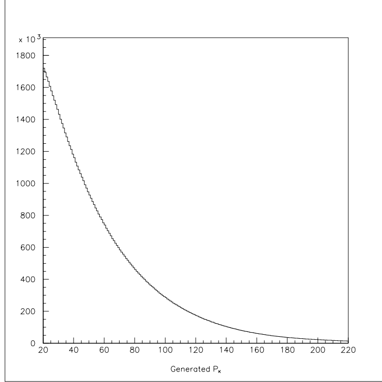
Figure 4.1: Distribution of the kaon momentum in the generated range of 20 to 220 GeV.
