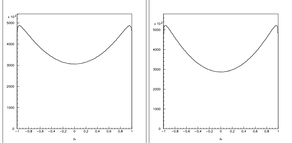
Figure 4.5: Distribution of y_a (left) and y_b (right). The plots include all \pi^0 \rightarrow e^+e^-e^+e^- events plus \pi^0 \rightarrow e^+e^-e^+e^-\gamma events with x_{4e} > 0.9 .
