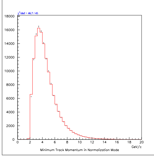
Figure 6.7: Comparison between normalization mode data (points with error bars) and normalization mode Monte Carlo (histogram) for the distribution of minimum track momentum. All other cuts have been applied.
