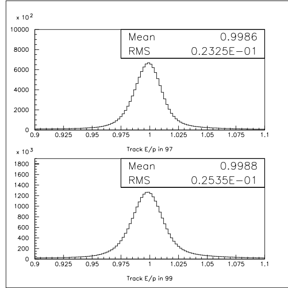
Figure 5.9: Distribution of the energy deposited in the calorimeter divided by the momentum measured in the spectrometer, for 97 (top) and 99 (bottom).
