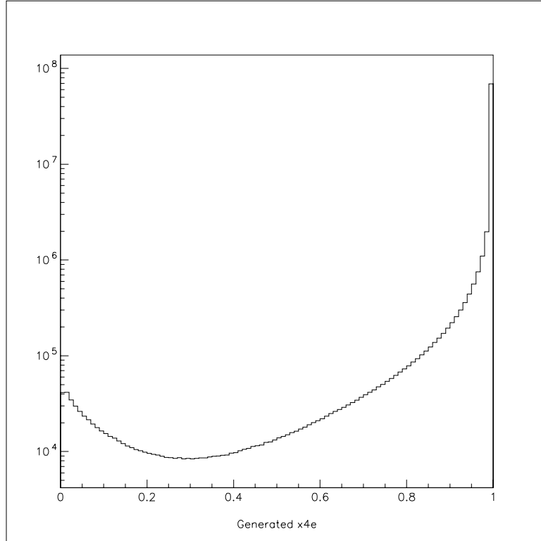
Figure 2.5: Monte Carlo distribution of x_{4e} .
