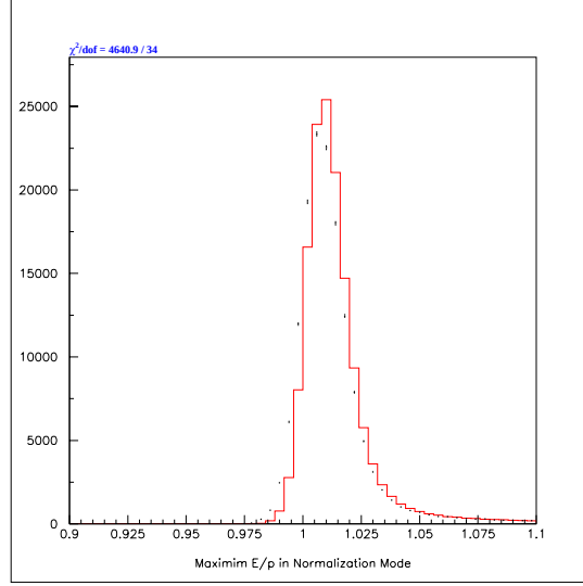
Figure 6.9: Comparison between normalization mode data (points with error bars) and normalization mode Monte Carlo (histogram) for the distribution of largest E/p . All other cuts have been applied.
