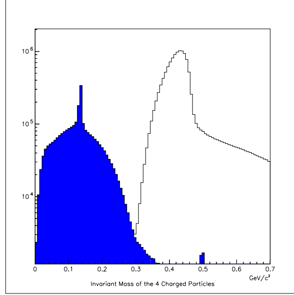
Figure 5.11: Distribution of the invariant mass of the four charged particles in events in the 4TRACK crunch stream. The events in the blue histogram have all four E/p 's greater than 0.9.
