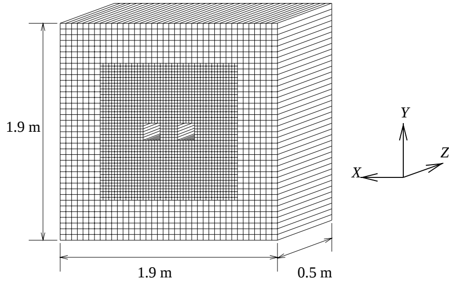
Figure 3.5: Sketch depicting the upstream face of the CsI array.
