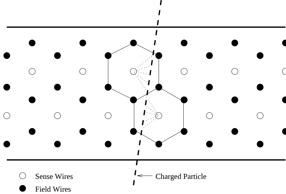
Figure 3.4: Drift chamber plane pair geometry and illustration of ionization process.
