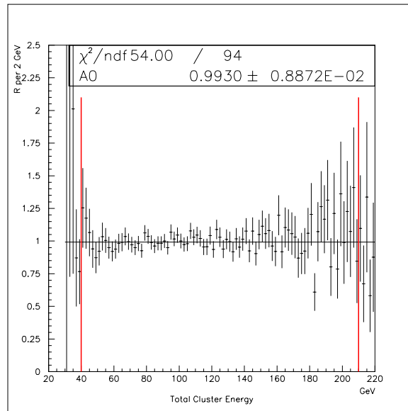
Figure 6.20: Double ratio as a function of the total energy.
