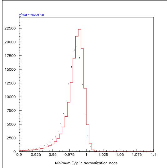
Figure 6.8: Comparison between normalization mode data (points with error bars) and normalization mode Monte Carlo (histogram) for the distribution of smallest E/p . All other cuts have been applied.
