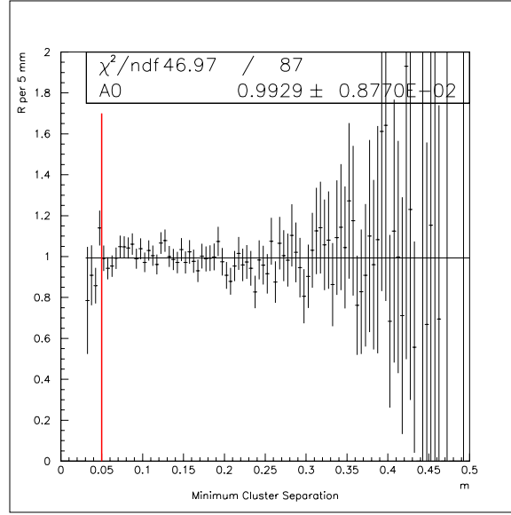
Figure 6.21: Double ratio as a function of the minimum cluster separation.
