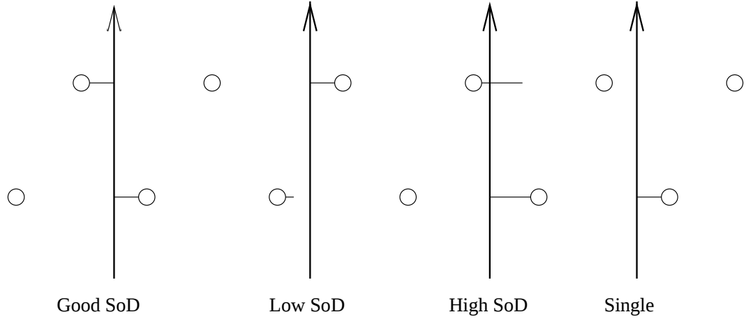
Figure 5.4: Cartoon of various pair configurations.
