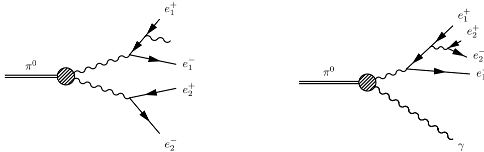
Figure 2.4: Two examples of contributions to the radiative double Dalitz decay.
