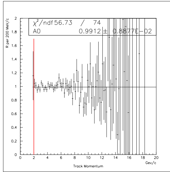
Figure 6.22: Double ratio as a function of the minimum track momentum.
