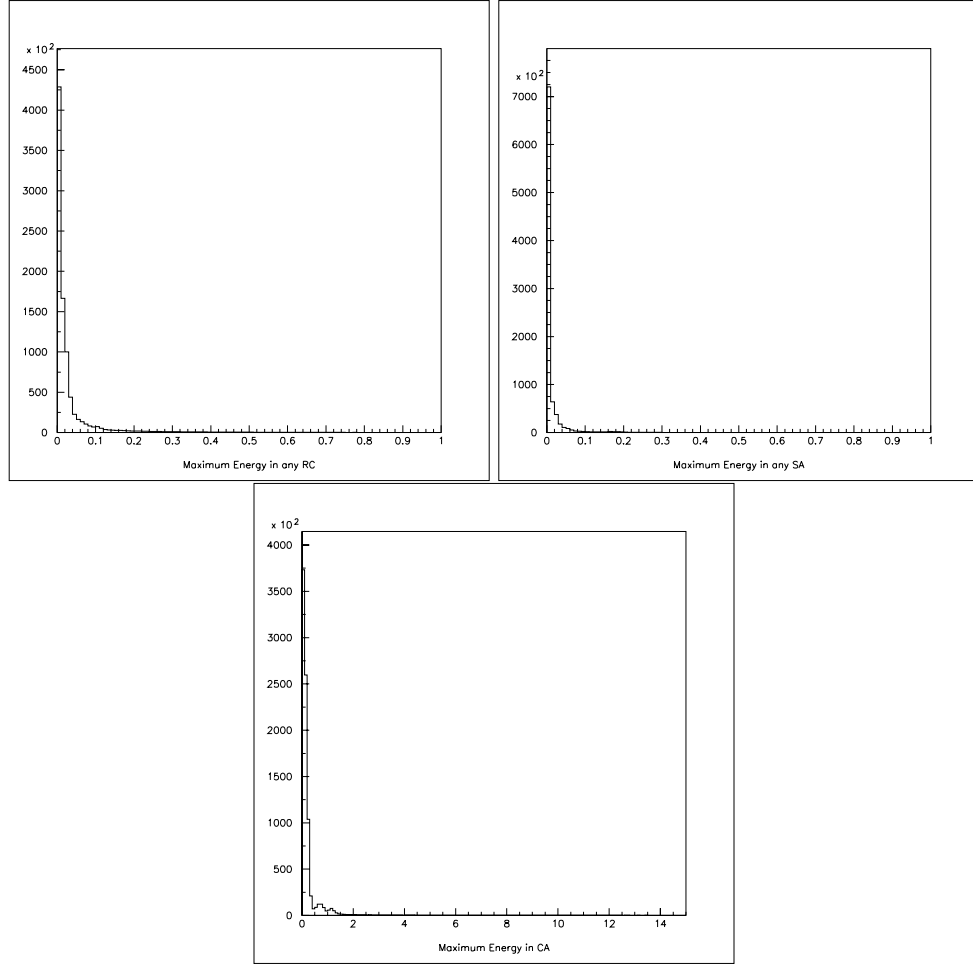
Figure 6.2: Distributions of the maximum energy deposited in, from left to right, the RC's, the SA's, and the CA's, for the entire 4e8c dataset (in GeV).
