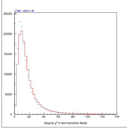
Figure 6.11: Comparison between normalization mode data (points with error bars) and normalization mode Monte Carlo (histogram) for the distribution of magnet \chi^2 . All other cuts have been applied.
