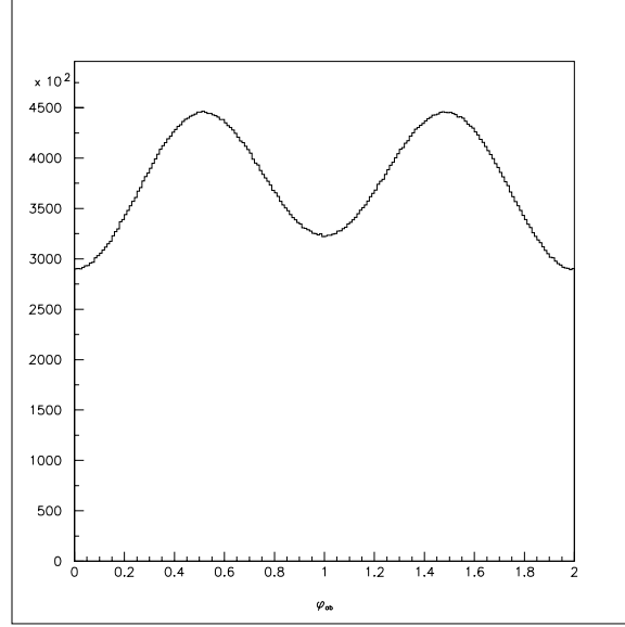
Figure 4.6: Distribution of \phi . The plots include all \pi^0 \rightarrow e^+e^-e^+e^- events plus \pi^0 \rightarrow e^+e^-e^+e^-\gamma events with x_{4e} > 0.9 .
