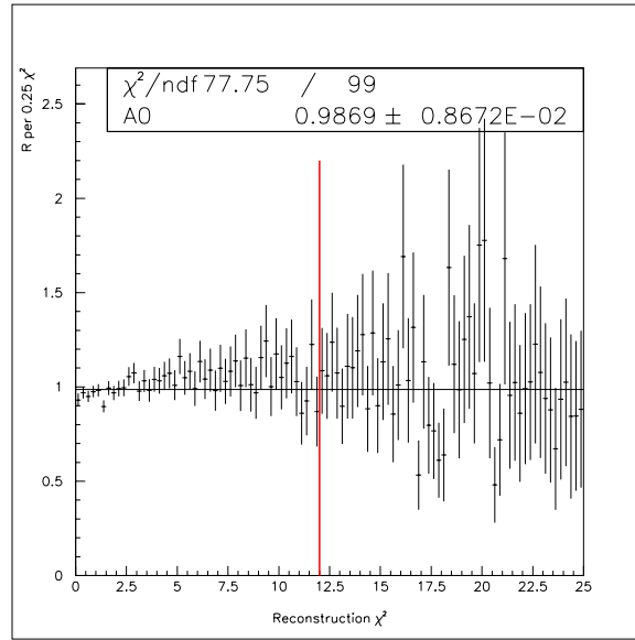
Figure 6.30: Double ratio as a function of the pairing \chi^2 .
