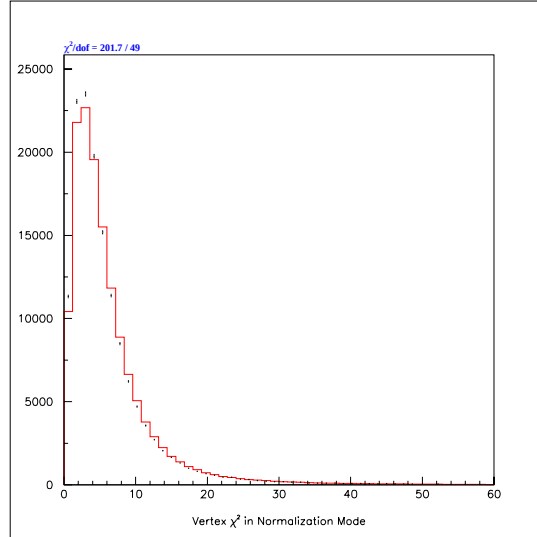
Figure 6.10: Comparison between normalization mode data (points with error bars) and normalization mode Monte Carlo (histogram) for the distribution of vertex \chi^2 . All other cuts have been applied.
