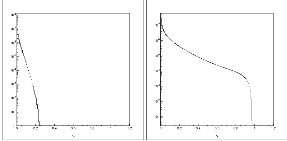
Figure 4.4: Distribution of x_a (left) and x_b (right). The plots include all \pi^0 \rightarrow e^+e^-e^+e^- events plus \pi^0 \rightarrow e^+e^-e^+e^-\gamma events with x_{4e} > 0.9 .
