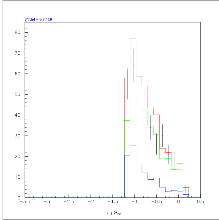
Figure 8.2: Distribution of \log \theta_{\min} . The points with error bars are the data, the green histogram is the internal radiation MC, the blue histogram is the external radiation MC, and the red histogram is the sum of the MC.
