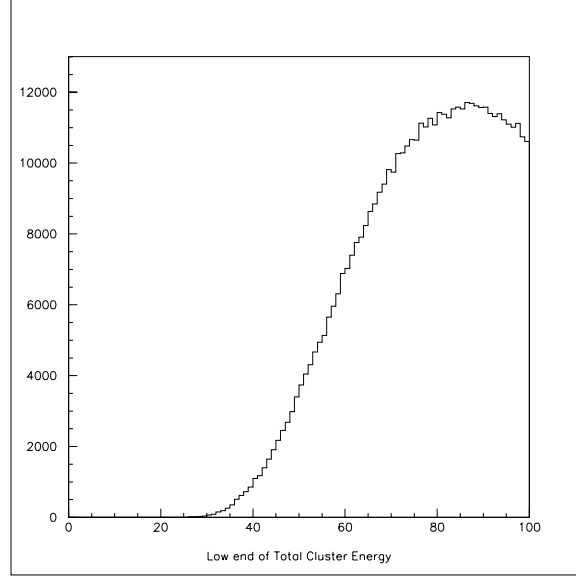
Figure 6.3: Low end of the distribution of total energy (in GeV) in the 8 hardware clusters.
