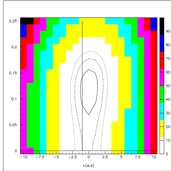
Figure 7.3: Likelihood function in two variables at the minimum of the third variable, using a Monte Carlo sample equivalent to one dataset. The two free variables are \alpha-\eta . The contours indicate the 1, 2, and 3\sigma levels appropriate for two free parameters. The generated point (0,0) is given by the crossing of the two lines.
