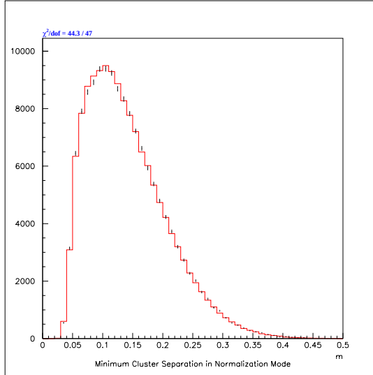
Figure 6.6: Comparison between normalization mode data (points with error bars) and normalization mode Monte Carlo (histogram) for the distribution of minimum cluster separation. All other cuts have been applied.
