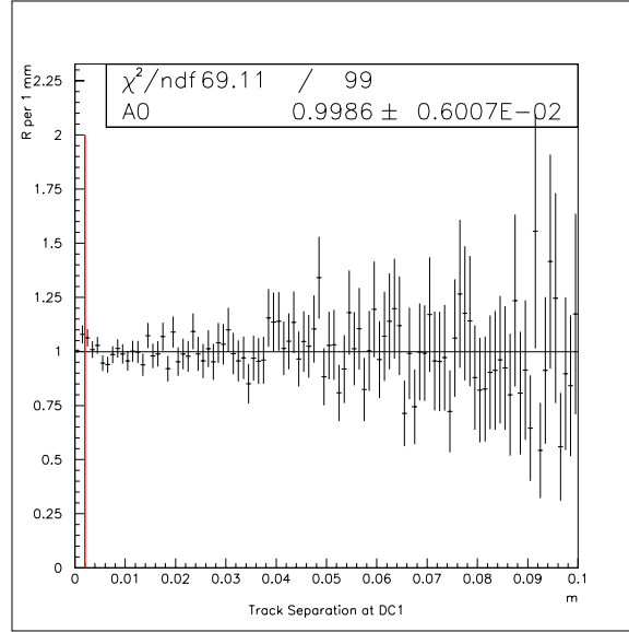
Figure 6.31: Double ratio as a function of the minimum track separation.
