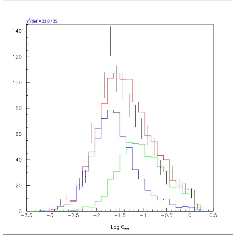
Figure 8.1: Distribution of \log \theta_{\min} . The points with error bars are the data, the green histogram is the internal radiation MC, the blue histogram is the external radiation MC, and the red histogram is the sum of the MC.
