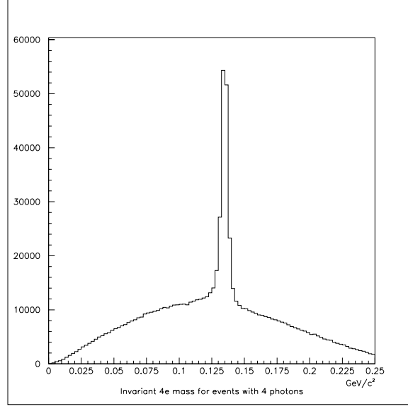
Figure 5.13: Distribution of the invariant mass of the four electrons in events with four photons.
