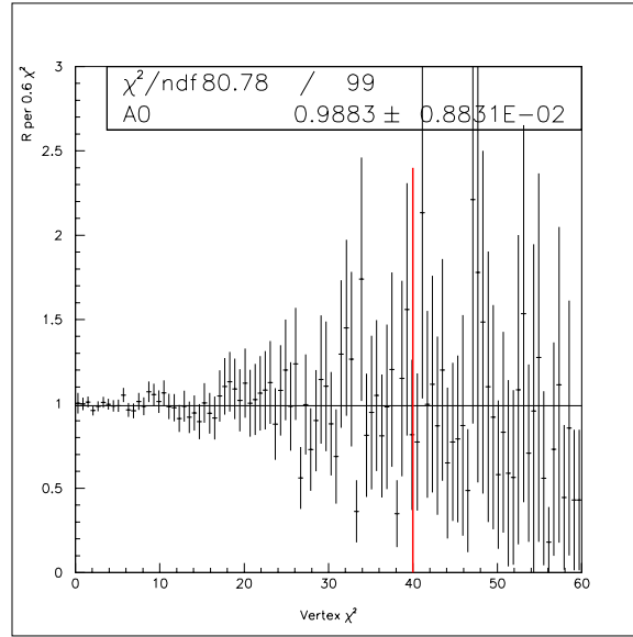
Figure 6.25: Double ratio as a function of the vertex \chi^2 .
