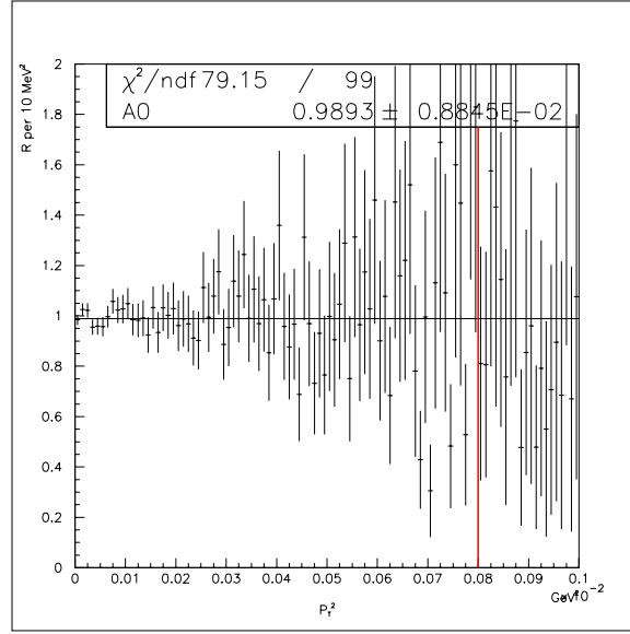
Figure 6.29: Double ratio as a function of the transverse momentum squared.
