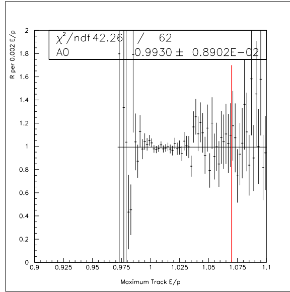
Figure 6.24: Double ratio as a function of the maximum E/p .
