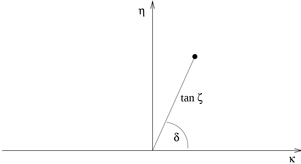
Figure 7.1: \kappa - \eta Plane.
