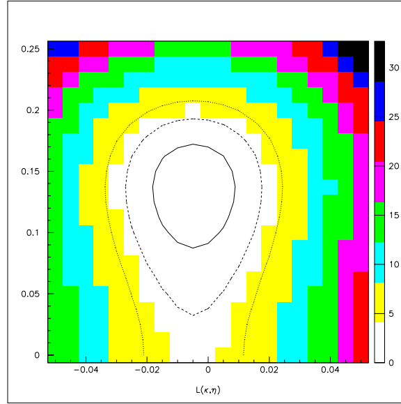
Figure 7.12: Likelihood function in two variables at the minimum of the third variable, using the complete KTeV dataset. The two free variables are \kappa – \eta . The contours indicate the 1, 2, and 3 \sigma levels appropriate for two free parameters.
