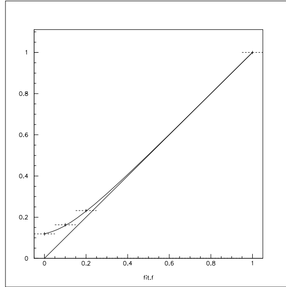
Figure 7.8: Map of extracted versus generated values of \eta .
