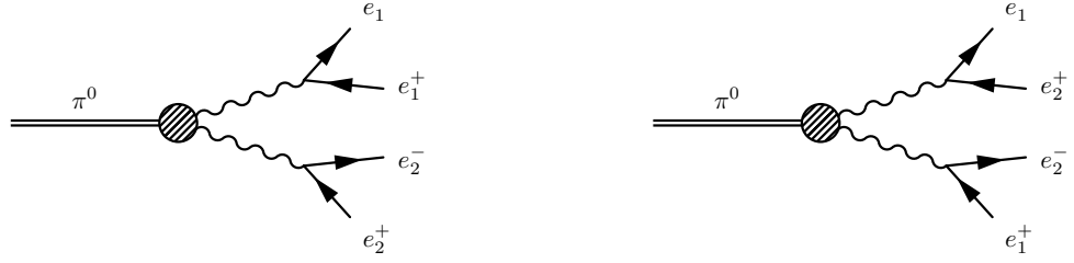
Figure 2.3: The two contributions to the double Dalitz decay at tree level.
