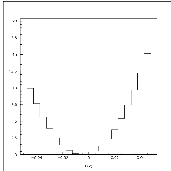
Figure 7.14: Likelihood function in one variable at the minimum of the other two variables, using the complete KTeV dataset. The free variable is \kappa .
