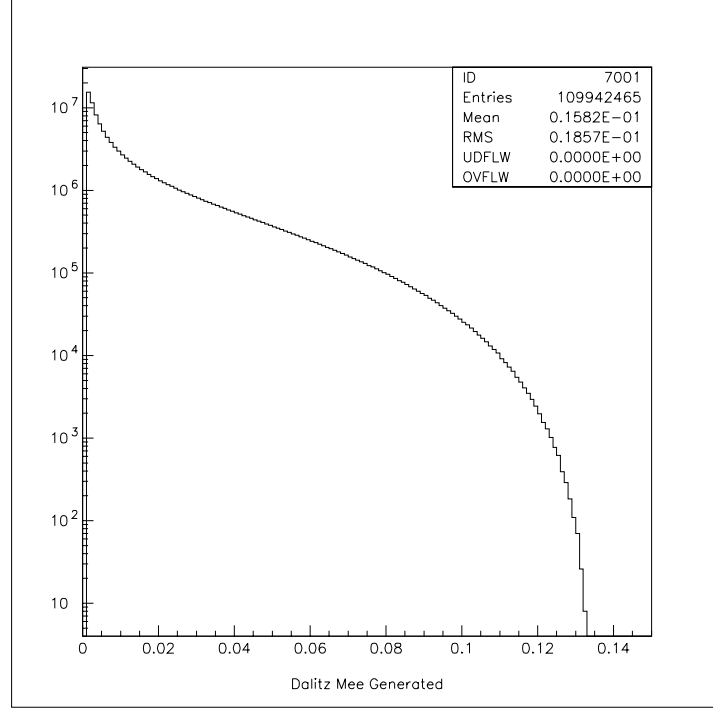
Figure 2.2: Predicted distribution of e^+e^- invariant masses in \pi^0 \rightarrow e^+e^-\gamma decays shown on a logarithmic scale.
