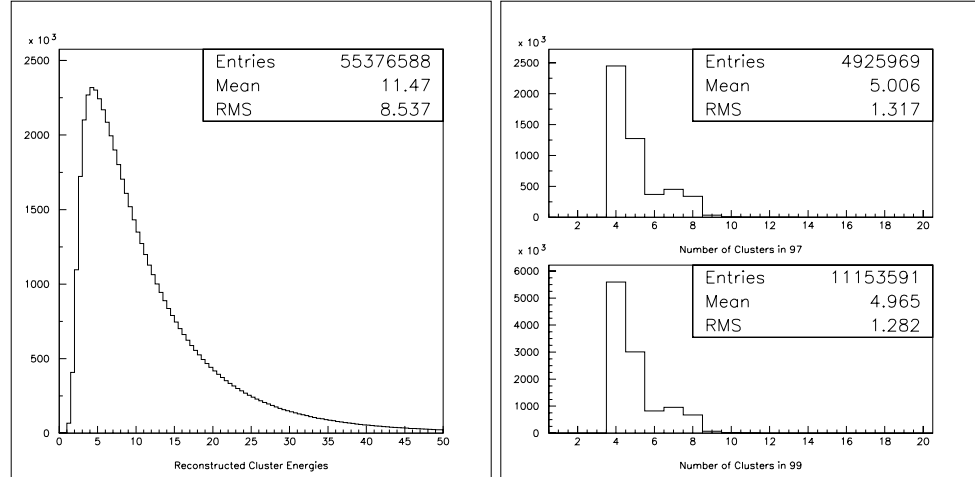
Figure 5.6: Distributions of the reconstructed cluster energies in the 99 2e-nclus 4-track data (left) and the number of clusters per event in the 97 data (top right) and in the 99 data (bottom right).
