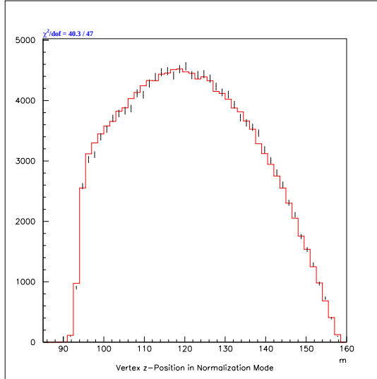
Figure 6.12: Comparison between normalization mode data (points with error bars) and normalization mode Monte Carlo (histogram) for the distribution of vertex z -position. All other cuts have been applied.
