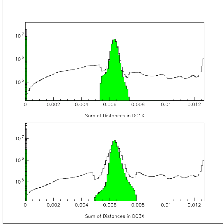
Figure 5.3: Distribution of Sum-of-Distances in the 4-track data. The top plot shows the SOD of all pairs (clear histogram) and the SOD of pairs used on tracks (green histogram) in DC1X. The bottom plot shows the same thing but in DC3X.
