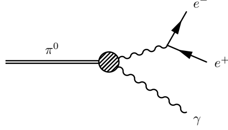
Figure 2.1: Single Dalitz Tree Level Feynman Diagram.
