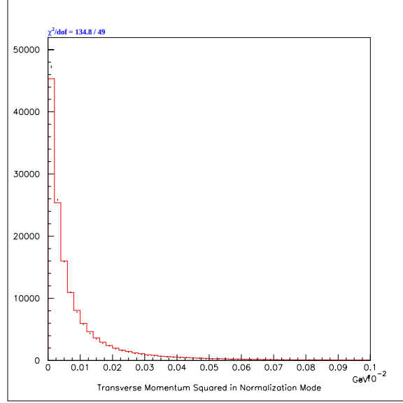
Figure 6.14: Comparison between normalization mode data (points with error bars) and normalization mode Monte Carlo (histogram) for the distribution of the square of the transverse momentum. All other cuts have been applied.
