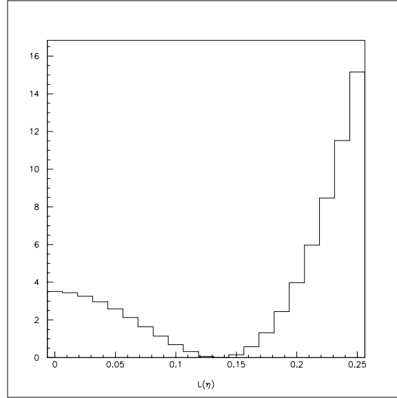
Figure 7.15: Likelihood function in one variable at the minimum of the other two variables, using the complete KTeV dataset. The free variable is \eta .
