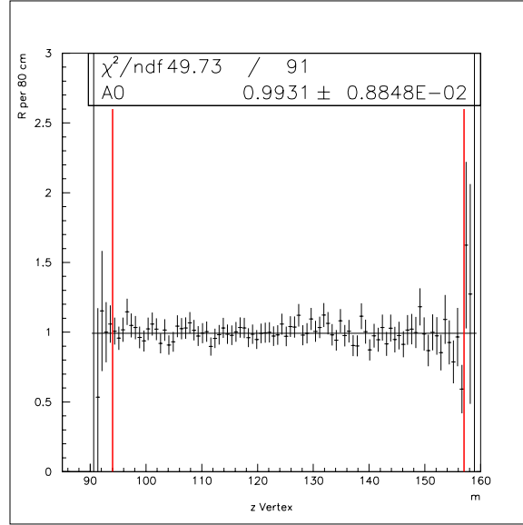
Figure 6.27: Double ratio as a function of the vertex z -position.
