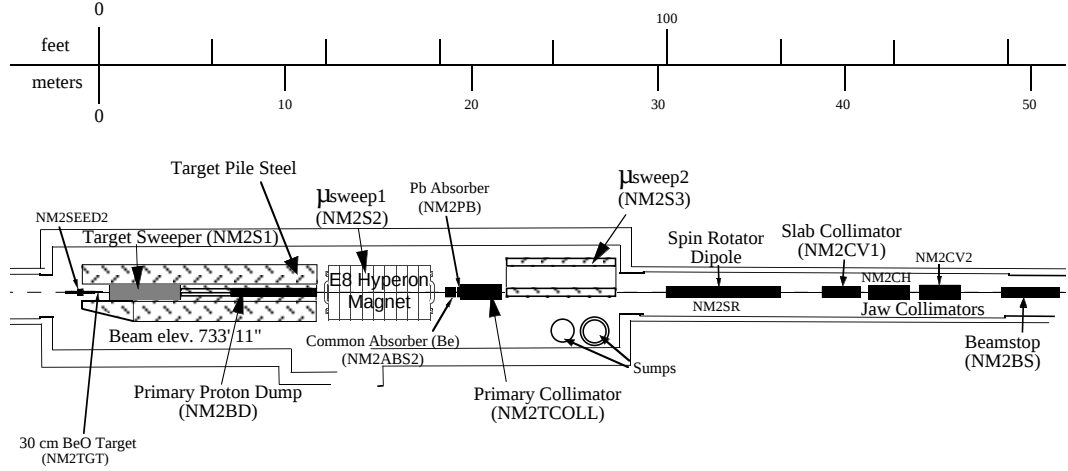
Figure 3.2: KTeV Beam-line. The NM2 enclosure houses the target, beam dump, sweeper magnets, absorbers and collimators.
