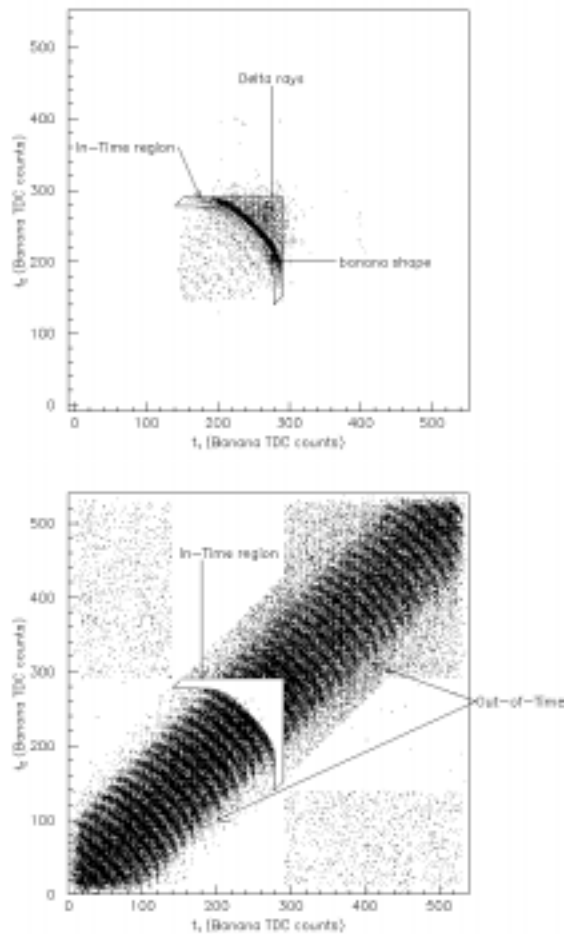
Figure 3.6: Banana TDC counts t_1 vs. t_2 . The top figure contains hits used on tracks in good 2-track events. The lower figure contains all rejected hits. The in-time pair region is shown in both.
