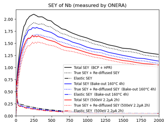
Figure 3: SEY of Niobium measured by ONERA.
