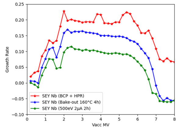
Figure 4: Multipactor growth rate in MYRRHA Spoke cavity simulated with SPARK3D.
