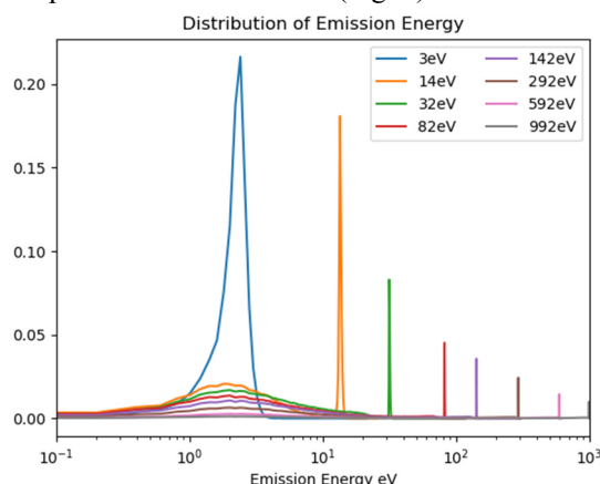
Figure 2: Energy distribution of secondary electrons for different primary electron energies.
