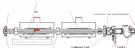
Figure 4: Schematic diagram of the extended EBIS. The polarized ^3\text{He} gas is injected into the drift tube in the Gas Trap of EBIS. Low Energy Beam Transport (LEBT) transfer the extracted beam from EBIS to the Radio Frequency Quadrupole (RFQ) e accelerator.
