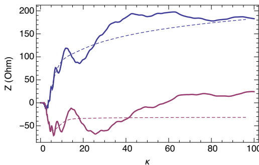
Figure 4: Plot of the real (blue) and imaginary (magenta) parts of the impedance Z for \ell = 20 . The dashed lines show the real and imaginary parts of Z from Fig. 1 corresponding to \ell = \infty .
