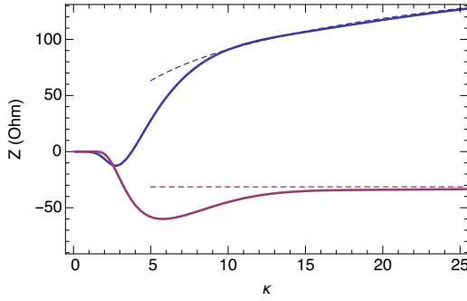
Figure 2: Plot of the real (blue) and imaginary (magenta) parts of the impedance Z (in Ohms) given by Eq. (10) as a function of the dimensionless wavenumber \kappa . The dashed lines show the high-frequency approximation Eq. (13).
