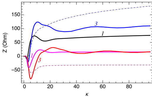
Figure 3: Plot of the impedance for l/\sqrt{a\rho} = 1 ( \Re Z - black, \Im Z - magenta) and for l/\sqrt{a\rho} = 3 ( \Re Z - blue, \Im Z - red) calculated with Eq. (14). The dashed lines show the real and imaginary parts of Z from Fig. 1 corresponding to \ell = \infty .
