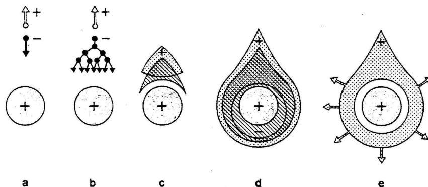
Figure 4.4: Development of a charge avalanche [21]: a) An electron-ion pair is generated. b) The electron is accelerated by the electric field and ionises other atoms. c) The electrons continue drifting to the anode wire, still ionising more atoms. d) Now, the electron cloud surrounds the anode wire. e) The electrons are collected by the anode wire and a cloud of ions drifts to the cathode.
