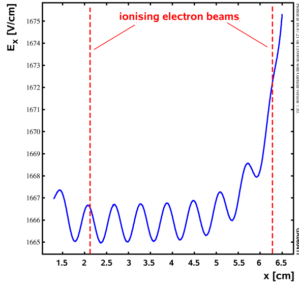
Figure 6.11: The effect on the electric field when increasing the value of the resistor between the 1th and 2nd row (at x_1 = 6.6 cm and x_2 = 6.0 cm) of the field electrodes by 10 k \Omega .
