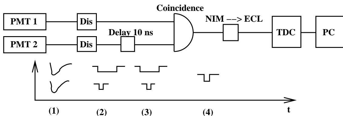
Figure 8.2: The signals from the two PMTs are first sent to discriminators, where the signal from PMT1 is translated into a long ( \sim 50 - 100 ns) NIM-pulse, the signal from PMT2 in a short ( \sim 10 ns) one. The latter is delayed by 10 ns so that it arrives always later at the coincidence than the PMT1 signal. Thus, the start of the coincidence signal is always defined by the pulse from PMT2.
