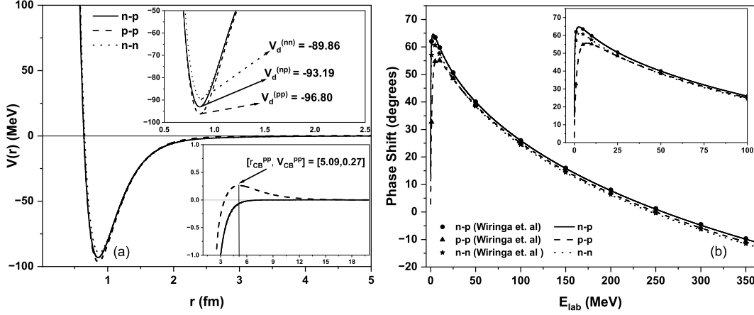
FIG. 1: Scattering Potential for ^1S_0 state of n-p, p-p and n-n scattering along with their corresponding scattering phase shifts.
