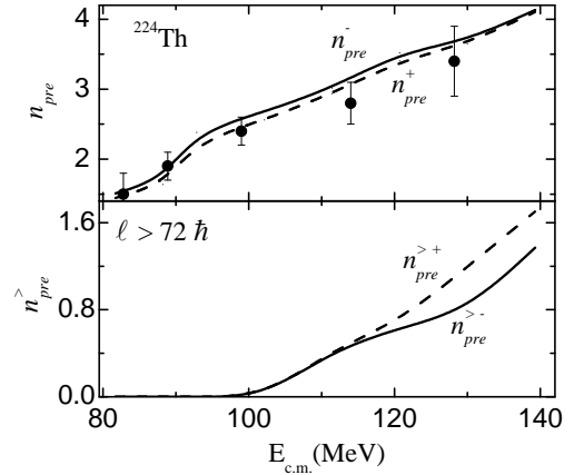
FIG. 1: n_{pre}^- (solid line) and n_{pre}^+ (dashed line) calculated with deformation independent \Gamma_n(\ell, c = 1) and deformation dependent \Gamma_n(\ell, c) , respectively. Experimental values (solid circles) of n_{pre} is taken from Ref. [1]
