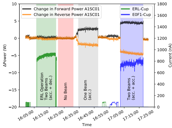
Figure 7: The forward (black curve) and reverse power (orange curve) changes of A1SC01 as well as beam currents for ERL (green curve) and once recirculating operation (blue curve) have been measured during four different beam modes: ERL mode (green area), no beam in the main linac (red area), one accelerated beam (grey area) and two accelerated beams (blue area) in the main linac.
