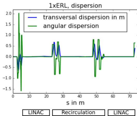
Figure 5: Simulation of dispersion curves for once recirculating ERL mode along the beam line.
