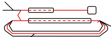
Figure 2: Scheme of the once recirculating ERL operation.
