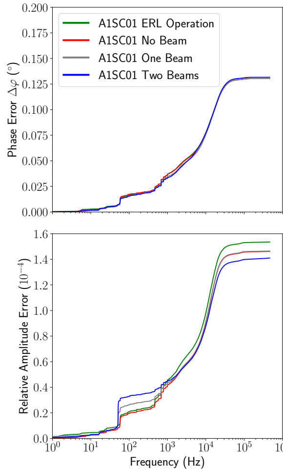
Figure 8: Phase and relative amplitude errors of A1SC01 have been measured during the four different beam modes. The data was transformed to frequency domain and integrated.
