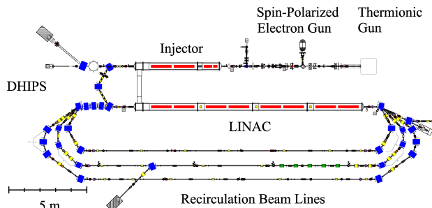
Figure 1: Floorplan of the S-DALINAC.
