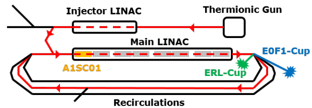
Figure 6: Beam path (red) of the once recirculating ERL mode is shown. The power of the first main linac cavity (A1SC01) as well as the beam currents corresponding to ERL (ERL cup) and once recirculating operation (E0F1) have been measured.
