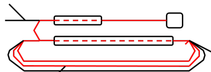
Figure 3: Scheme of the twice recirculating ERL operation.
