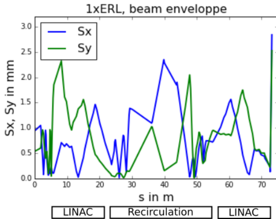
Figure 4: Simulation of horizontal ( S_x ) and vertical ( S_y ) beam envelopes for once recirculating ERL mode in x and y along the beam line.
