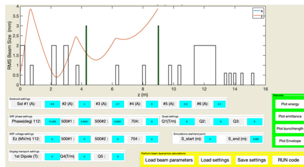
Figure 7. An online modelling of beam dynamics in accelerator section based on beam simulation for CeC experiment.
