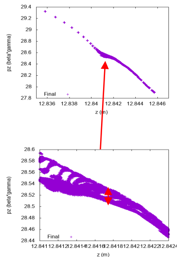
Figure 5. longitudinal phase space at the end of linac shows the beam has a core with peak current > 100 \text{ A} and slice energy spread < 2e-4 with correlated energy chirp \sim 2e-4 . The core consists of \sim 80\% of the total charge of 1 nC.
