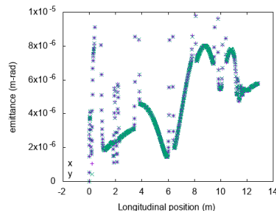
Figure 6. beam emittance at the end of beamline with optimized settings \sim 5.7 \mu\text{m} , satisfies the experimental requirement.
