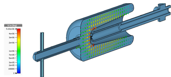
Figure 2: RF fields simulated in CST with cathode stalk inserted shows strong focusing at the cathode.
