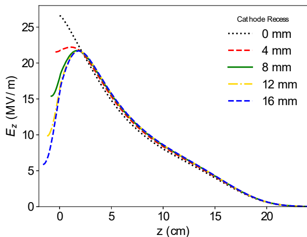
Figure 3. With adjustable cathode recess position, the proper focusing force can be selected to better suit beam dynamics in the gun.
