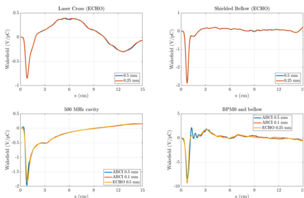
Figure 4. wakefields (around bunching cavities) simulated in ABCI and ECHO have decent agreement.
