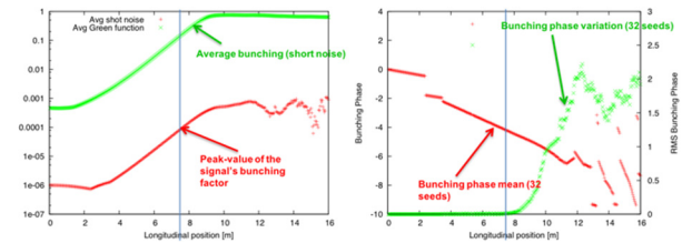
Figure 11. GENESIS simulated evolution of bunching factor of an imprint indicates we have plenty of gain for cooling (left). We operate our FEL in linear regime where phase variation due to shot noise stays low (right).
