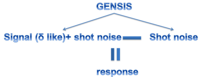
Figure 10. We calculate the gain (growth of bunching factor) of the imprint from ion beam on electron beam by taking the difference of bunching factor evolution (amplitude and phase) in GENESIS with and without signal.
