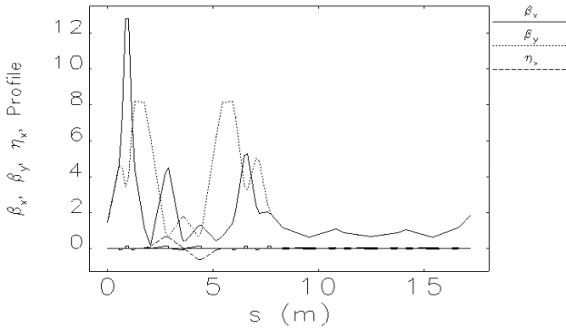
Figure 8. optics matching from the end of LEBT to and along the FEL section was done in ELEGANT using alternating quadrupoles.
