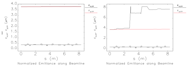
Figure 9. beam emittance can be blown up when the energy spread is large ( \sim 1\% , right). The emittance growth in dogleg is minimal while energy spread is reasonably low ( \sim 0.1\% , left).
