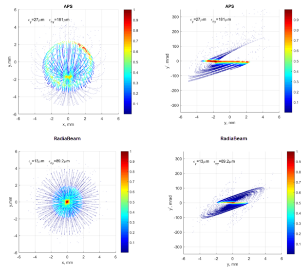
Figure 3: Comparison of beam profile (left) and transverse phase space (right) of the existing APS (top) and developed RadiaBeam (bottom) thermionic guns.
