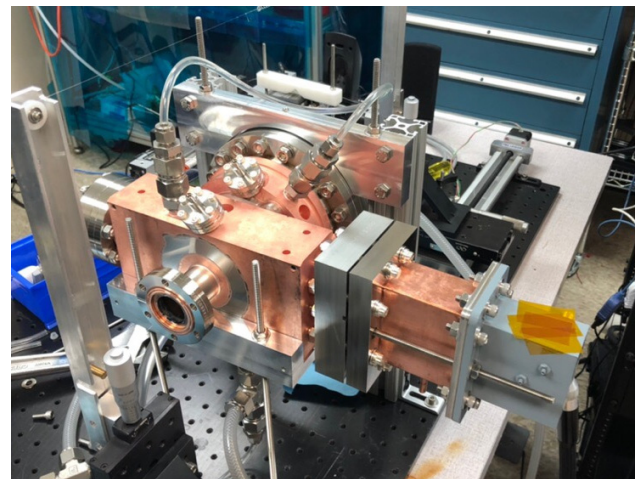
Figure 1: Picture of RadiaBeam's thermionic gun.
