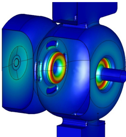
Figure 2: Electromagnetic design of the thermionic gun: surface electric field distribution.
