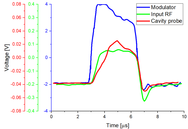
Figure 5: Measured RF signals during the conditioning: modulator RF pulse (blue), input RF power (green) and RF field envelope inside the structure (red).
