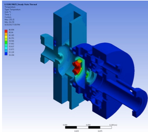
Figure 4: ANSYS thermal simulation of the gun.
