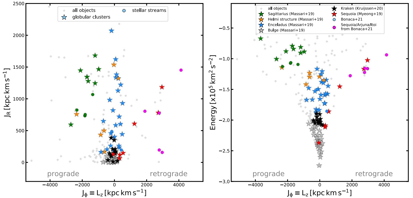
Figure 17. (J, E) space showing groupings of objects as found by previous studies. Different groups are shown with different colors, the globular clusters are shown with the “star” markers, and stellar streams are shown with the “circle” markers.
