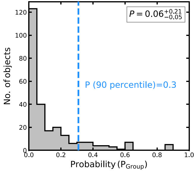
Figure 16. Same as Figure 4, but for the artificially randomized (J, E) distribution of objects. The vertical line shows the 90th percentile of this PDF, and we use the corresponding value to set the desired P_{\text{Threshold}} value. The other quoted value is the median of the distribution, and the corresponding uncertainties reflect its 16th and 84th percentiles.
