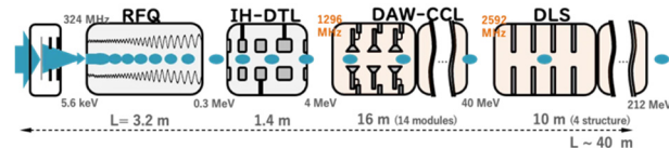
Figure 1: Layout of muon LINAC.
