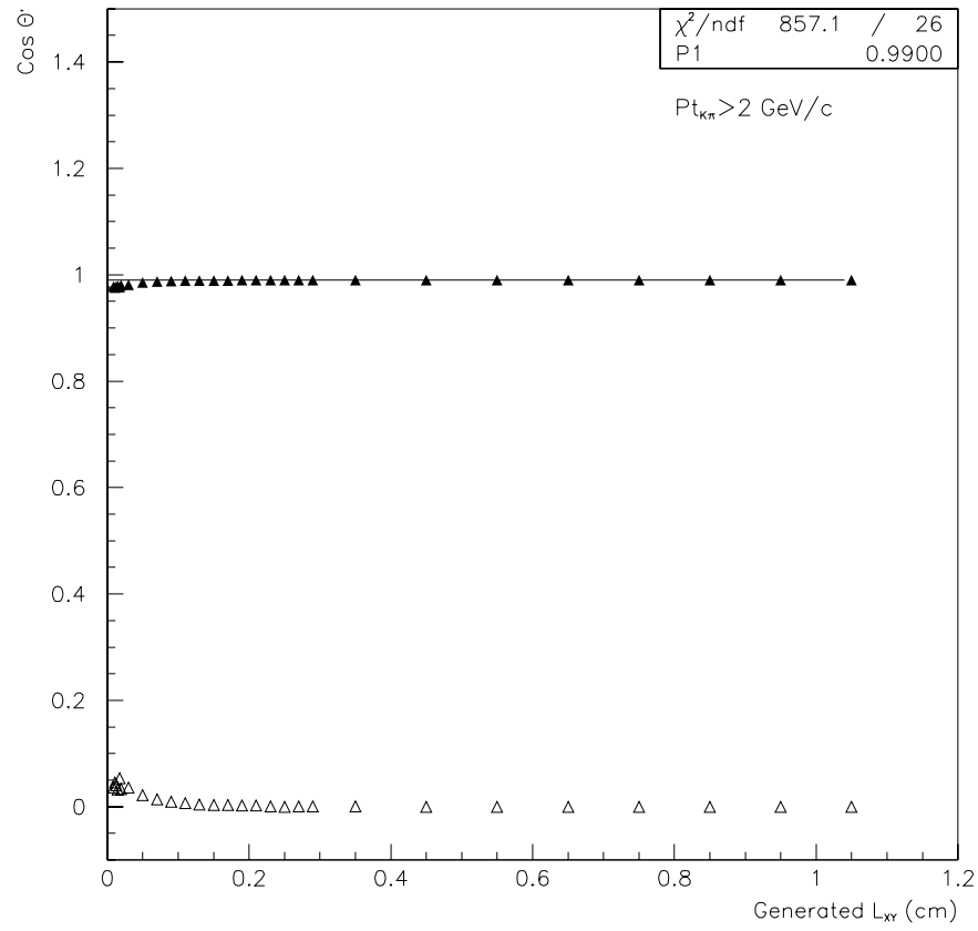
Figure 4-8. \cos \theta' with P_{t_{K^*}} > 2 \text{ GeV}/c . Black triangles are the mean values and the white triangles are the errors of the mean.
