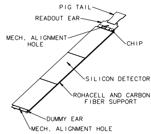
Figure 2-6. Schematic drawing of an SVX' ladder.
