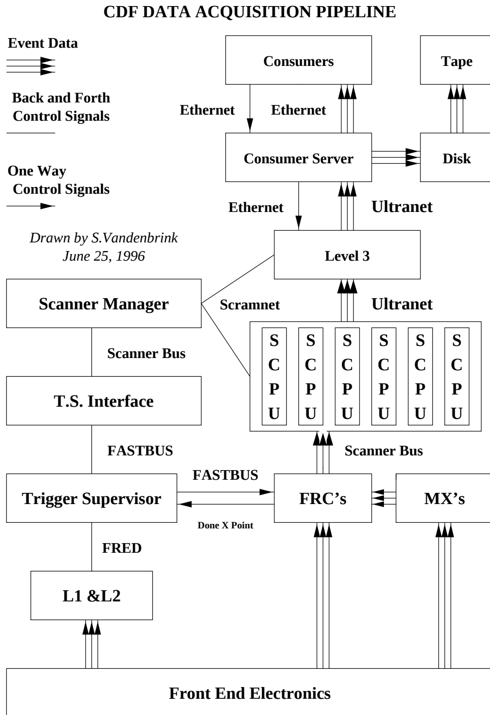
Figure 3-1. CDF data acquisition system flow chart.
