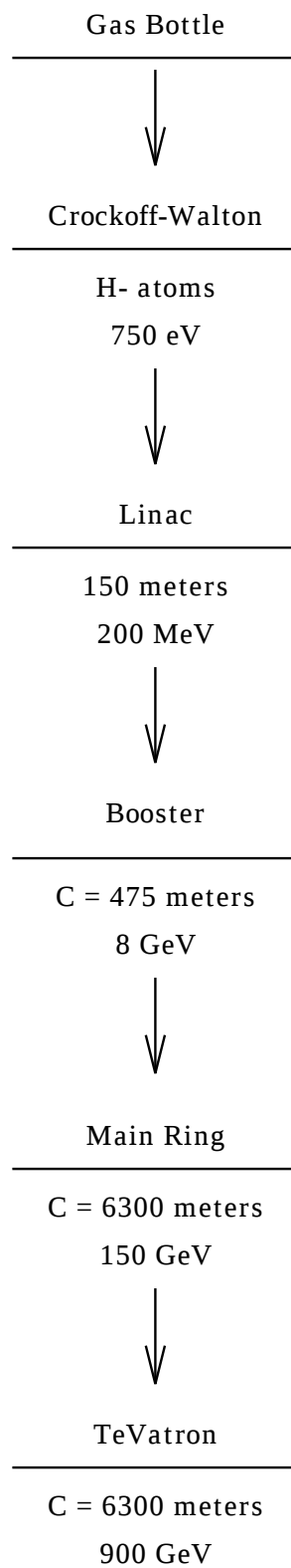
Figure 2-3. Flowchart of the protons acceleration up to 900 \text{ GeV}/c^2
