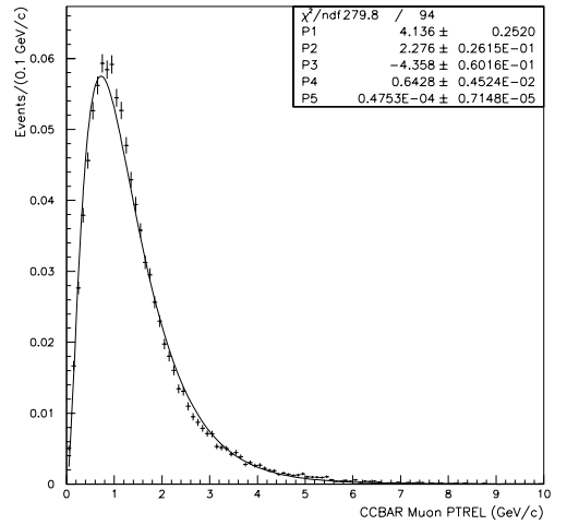
Figure 4-26. Normalized PTREL distribution for Run 1B c\bar{c} \mu 's fitted with P_1 x^{P_2} \exp(P_3 x^{P_4}) + P_5 function.
