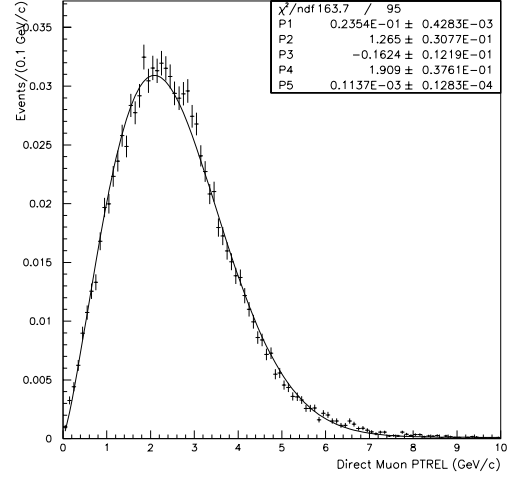
Figure 4-28. Normalized PTREL distribution for Run 1A direct \mu 's fitted with P_1 x^{P_2} \exp(P_3 x^{P_4}) + P_5 function.
