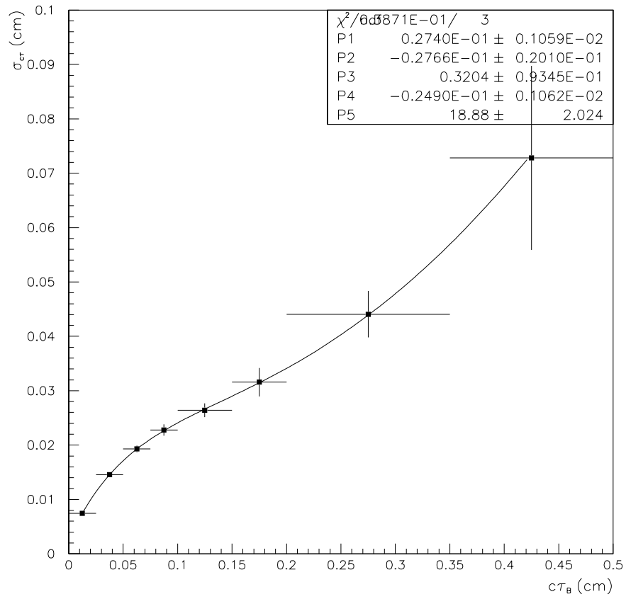
Figure 4-54. \sigma_{c\tau} = P_1 + P_2x + P_3x^2 + P_4e^{-P_5x} .
