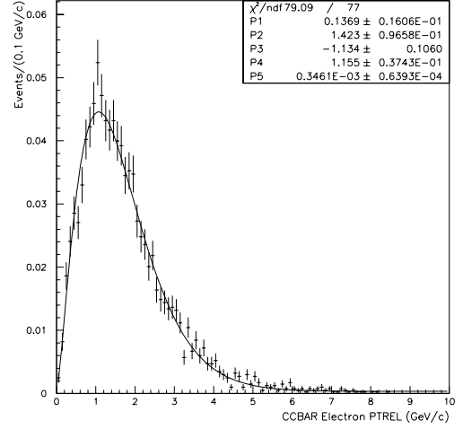
Figure 4-20. Normalized PTREL distribution for Run 1B c\bar{c} electrons fitted with P_1 x^{P_2} \exp(P_3 x^{P_4}) + P_5 .
