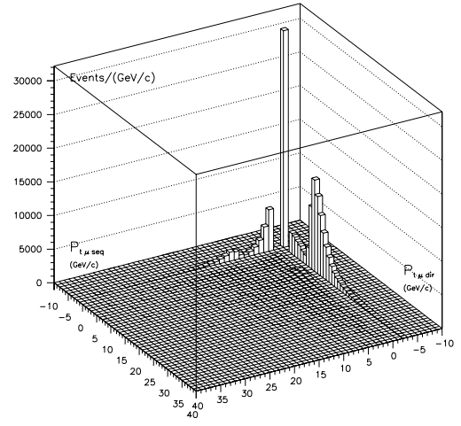
Figure 4-24. 3 dimensional scatter plot of P_t of sequential \mu 's and P_t of direct \mu 's. Notice that above P_{t,cutoff} \approx 6 \text{ GeV}/c there is a very little amount of sequentials passing the trigger cutoff.
