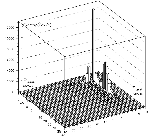
Figure 4-22. 3 dimensional scatter plot of P_t of sequential electrons and P_t of direct electrons. Notice that above P_{t,cutoff} \approx 6 \text{ GeV}/c there is a very little amount of sequentials passing the trigger cutoff.
