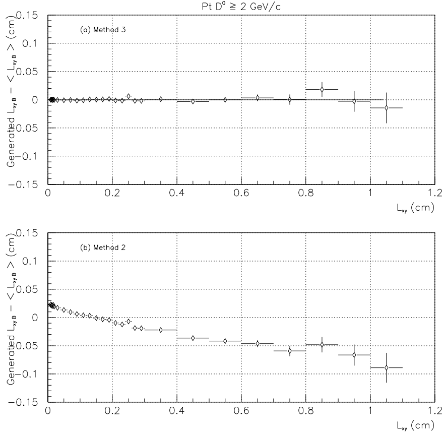
Figure 4-3. The difference between the generated and estimated L_{xyB} and its RMS for Method 3 (a) and for Method 2 (b) as a function of L_{xy} .
