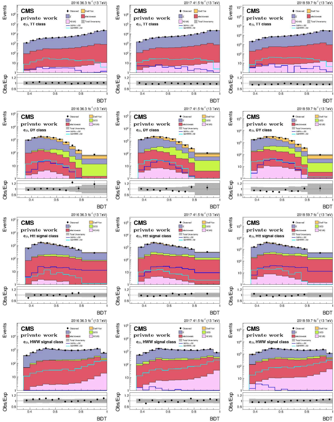
Figure 7.1: Profit plots for all the categories in e\mu channel for 2016, 2017 and 2018 years separately. The first row shows the t\bar{t} and single top class, the second one the DY+jet background, while the third the bbH \rightarrow \tau\tau signal and the fourth the bbH \rightarrow WW .
