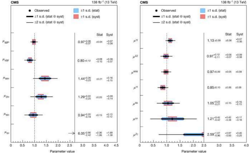
Figure 2.6: The figures show the signal strength and agreement with the SM for different production modes \mu_i on the left and decay channels \mu^f on the right. The thick and thin black lines represent the 1 and 2 standard deviations, and the blue and red bands, respectively, indicate the statistical and systematics components of the 1 standard deviations [33].
