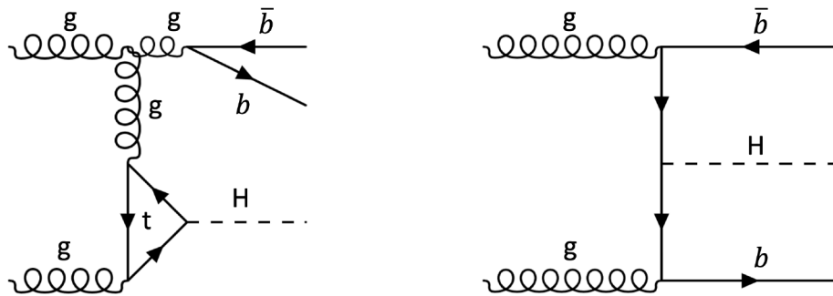
Figure 6.1: Feynman diagrams of the two main production modes of Higgs boson in association with a pair of b-quarks, (left) gluon-gluon fusion (ggF) with two additional b-quarks in the final state, (right) b-quark fusion.
