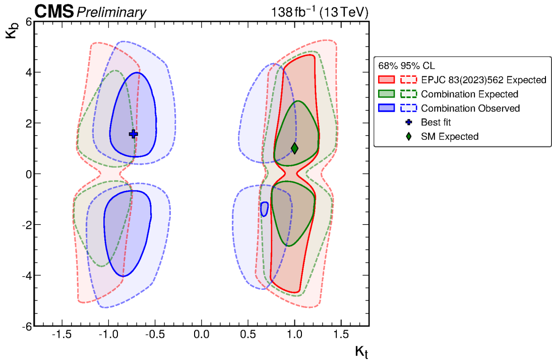
Figure 7.7: Two-dimensional scan of (\kappa_b, \kappa_t) for the inclusive Higgs measurement in the tau decay channel for the dominant Higgs production modes [129](labelled in the legend as EPJC) in red and its combination with the present bbH analysis in green. The observed limits using the full Run 2 dataset are shown with blue lines. The dashed (continuous) lines indicate respectively the 95(68)% confidence areas [128].
