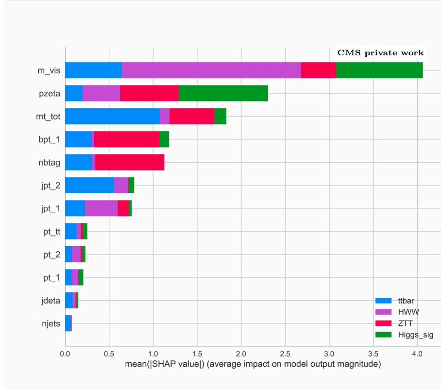
Figure 6.18: Input features ranked in decreasing order of their impact on the model output magnitude using the corresponding SHAP value, with the separation power of each class versus the rest highlighted with a different colour for each feature.
