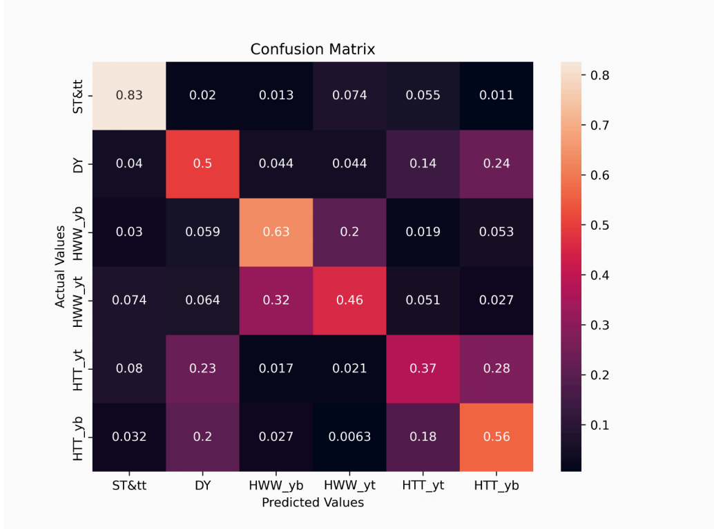
Figure B.7: Figure shows the confusion matrix for the training of the second level model to separate the bbH signal processes considering different amplitudes y_b and y_t .
