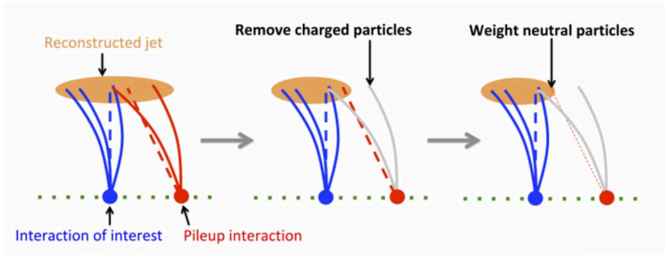
Figure 4.4: Sketch of the Pile Up mitigation techniques (CHS & PUPPI) used at CMS [84].
