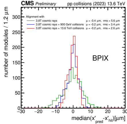
Figure 3: Distribution of median residuals in the local x coordinate on the barrel pixel detector according to alignment geometries derived iteratively in 2023.
